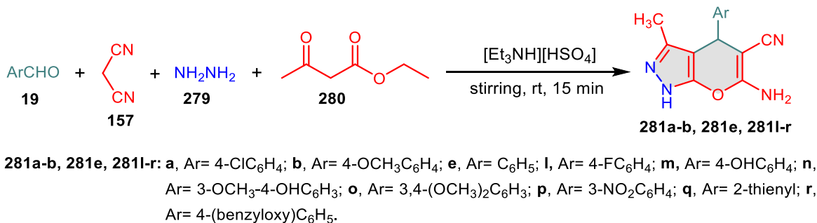
Scheme 63. Four-component reaction for the synthesis of dihydropyrano[2,3- c ]pyrazoles 281 .
