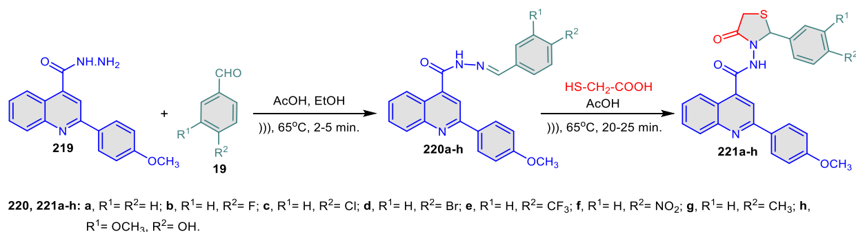
Scheme 49. Synthesis quinoline-based thiazolidinones 221a-h .
