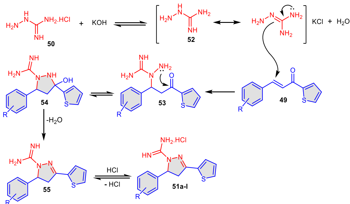
Scheme 13. Mechanism of the formation of 51a-l .
