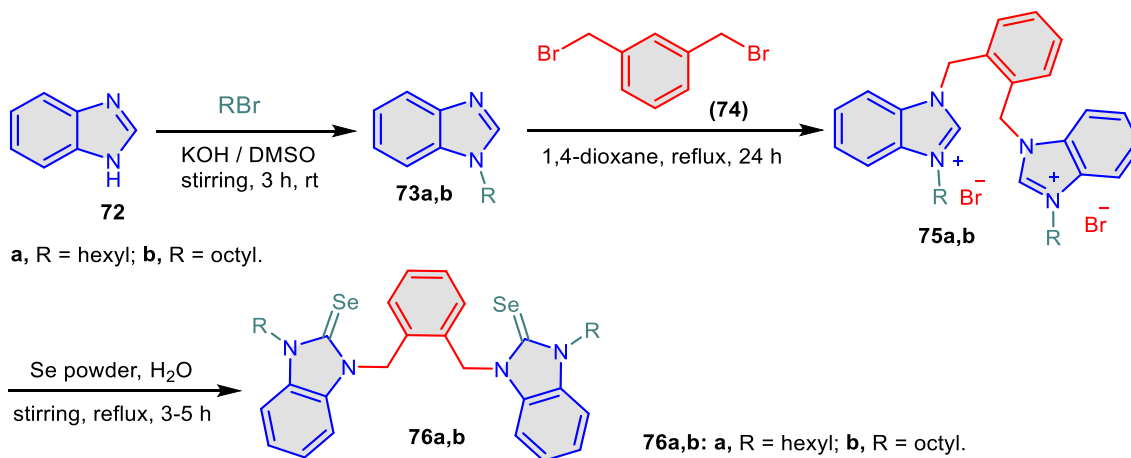
Scheme 18. Synthesis of selenium-bis-benzimidazoliums 76a,b .
