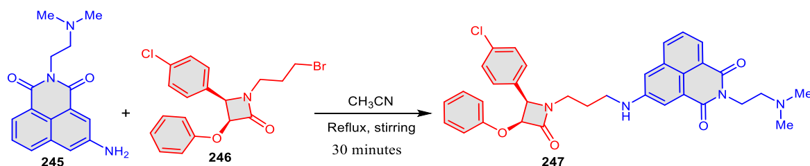
Scheme 53. Coupling reaction of amonafide 245 with \beta -lactam derivative 246 .
