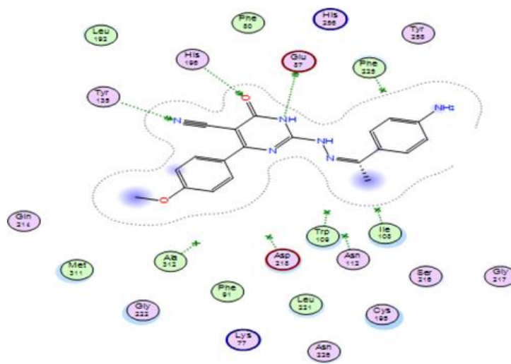
Figure 30. Mapping surface showing compound 236c occupying the active pocket of T.S 2D. T.S., thymidylate synthase. Reproduced from Ref.; 181 Copyright 2019; Wiley.
