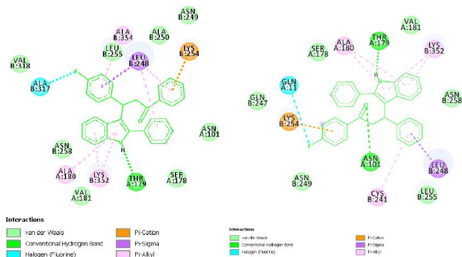
Figure 4. 2D interaction maps of compounds 17c and 17j with tubulin receptor. Reproduced with permission from Ref.; 23 Copyright 2019; Wiley.
