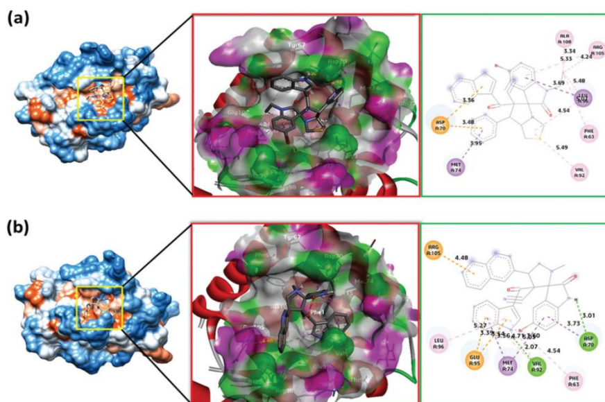
Figure 7. (a) Docking pose of 24u with BCL-2 receptor, (b) docking pose of 24w with BCL-2 receptor. Reproduced from Ref.; 34 Copyright 2022; Royal Society of Chemistry.
