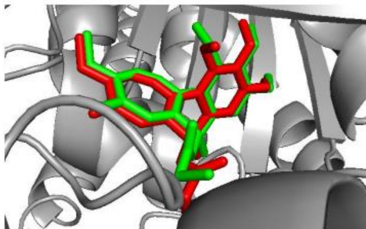
Figure 5. Crystallographic conformation (red) and docking conformation (green) of colchicine into the tubulin receptor.. Reproduced with permission from Ref.; 23 Copyright 2019; Wiley.
