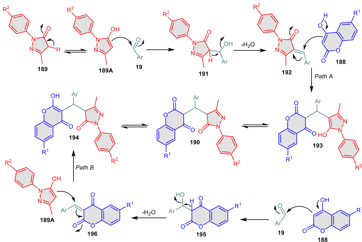
Scheme 43. Mechanism for the formation of 3-substituted chroman-2,4-diones 190 .
