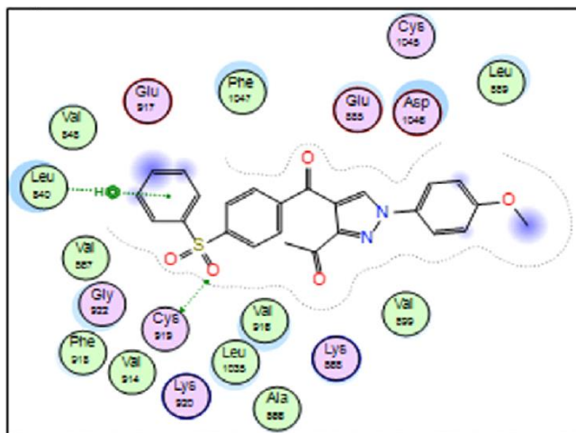
Figure 8. Compound 34a docked onto the active site of VEGFR-2 kinase in 2D. Reproduced with permission from Ref. 43 Copyright 2022; Elsevier.
