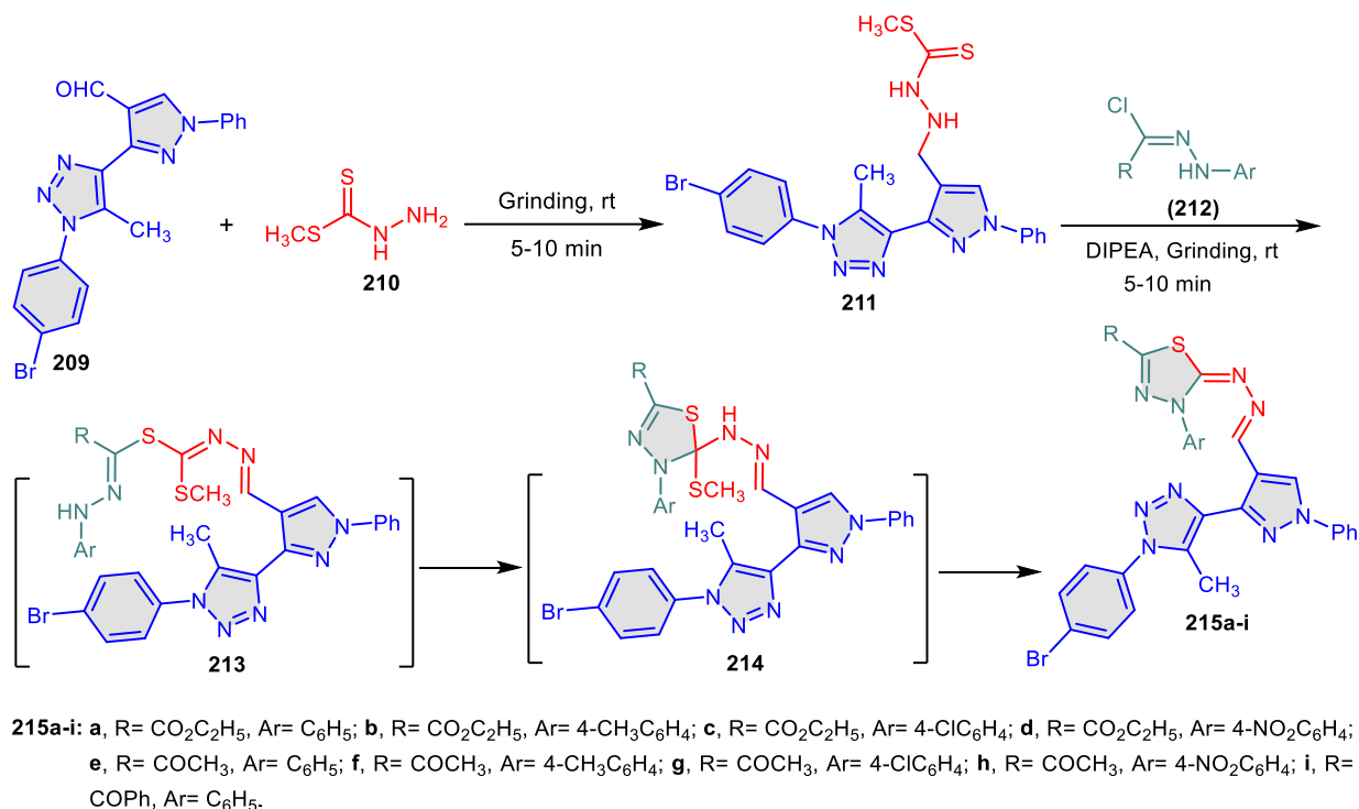
Scheme 47. Synthesis of hybrid 5-(substituted 1,2,3-triazole-4-yl)-1,3,4-thiadiazole derivatives 215a-i .
