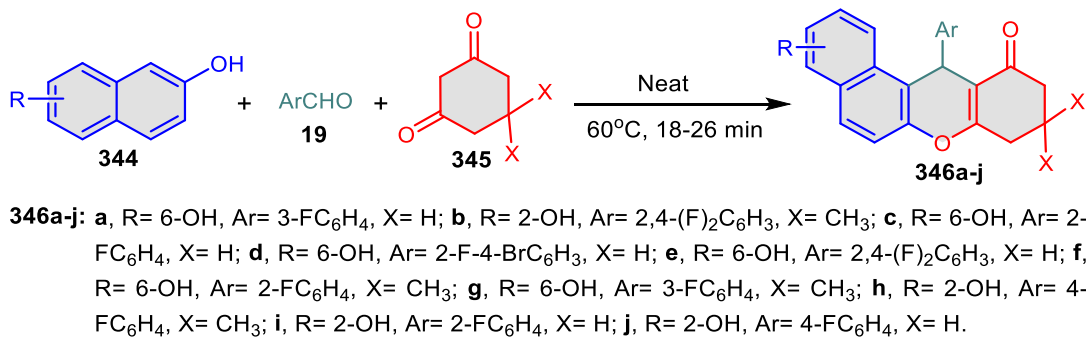
Scheme 80. Synthesis of substituted benzo[ a ][xanthen-11-(2 H )-ones 346a-j .
