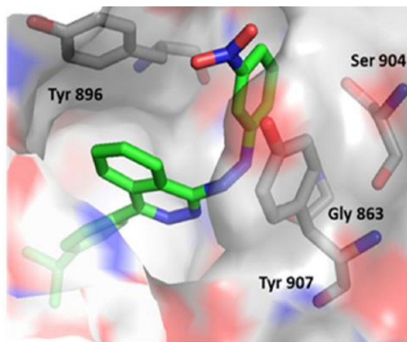
Figure 20. Surface representation of compound 123c bound to PARP-1 (PDB code: 7aad) active site. Reproduced with permission from Ref.; 99 Copyright 2024; Taylor & Francis.
