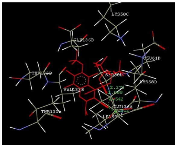
Figure 21. Binding interaction of compound 159b . Reproduced with permission from Ref., 134 Copyright 2019; Springer.
