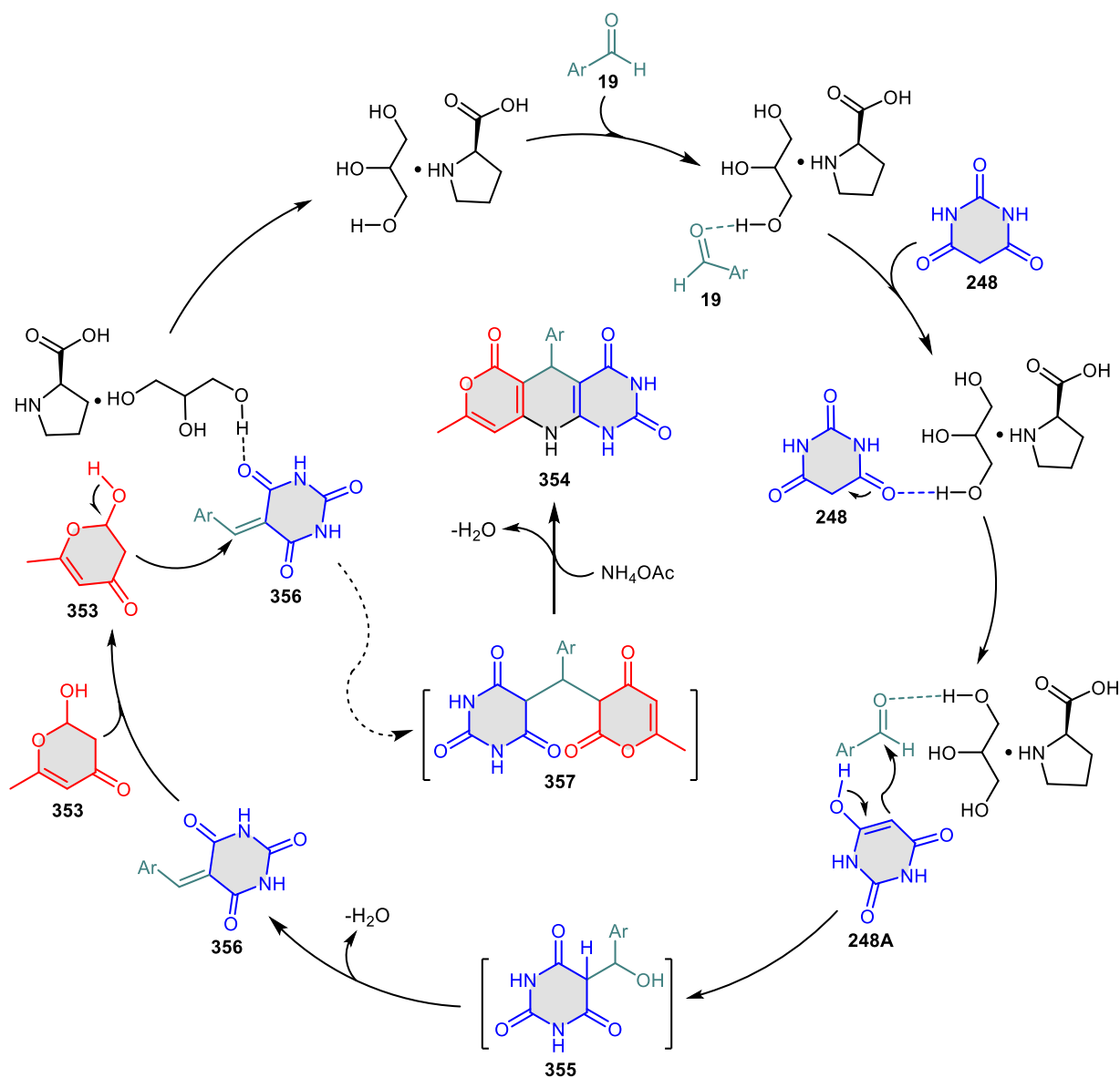
Scheme 84. Mechanistic pathway of pyrido-pyrimidines 354 .
