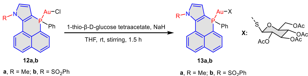
Scheme 3. Synthesis of pyrrole-phosphaphenalene gold complexes bearing thio-sugar substituent 13a,b .
