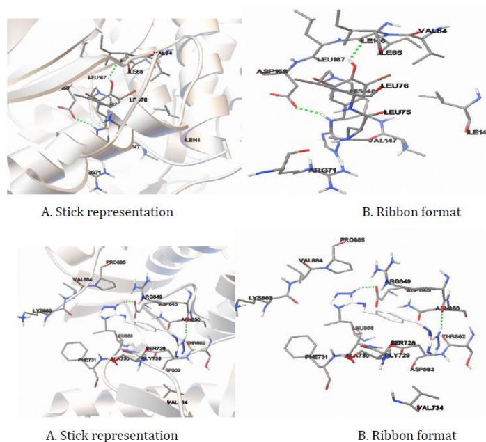
Figure 13. Orientation and position for compounds 84 and 85 with protein residue. Reproduced with permission from Ref.; 76 Copyright 2014; SPC.
