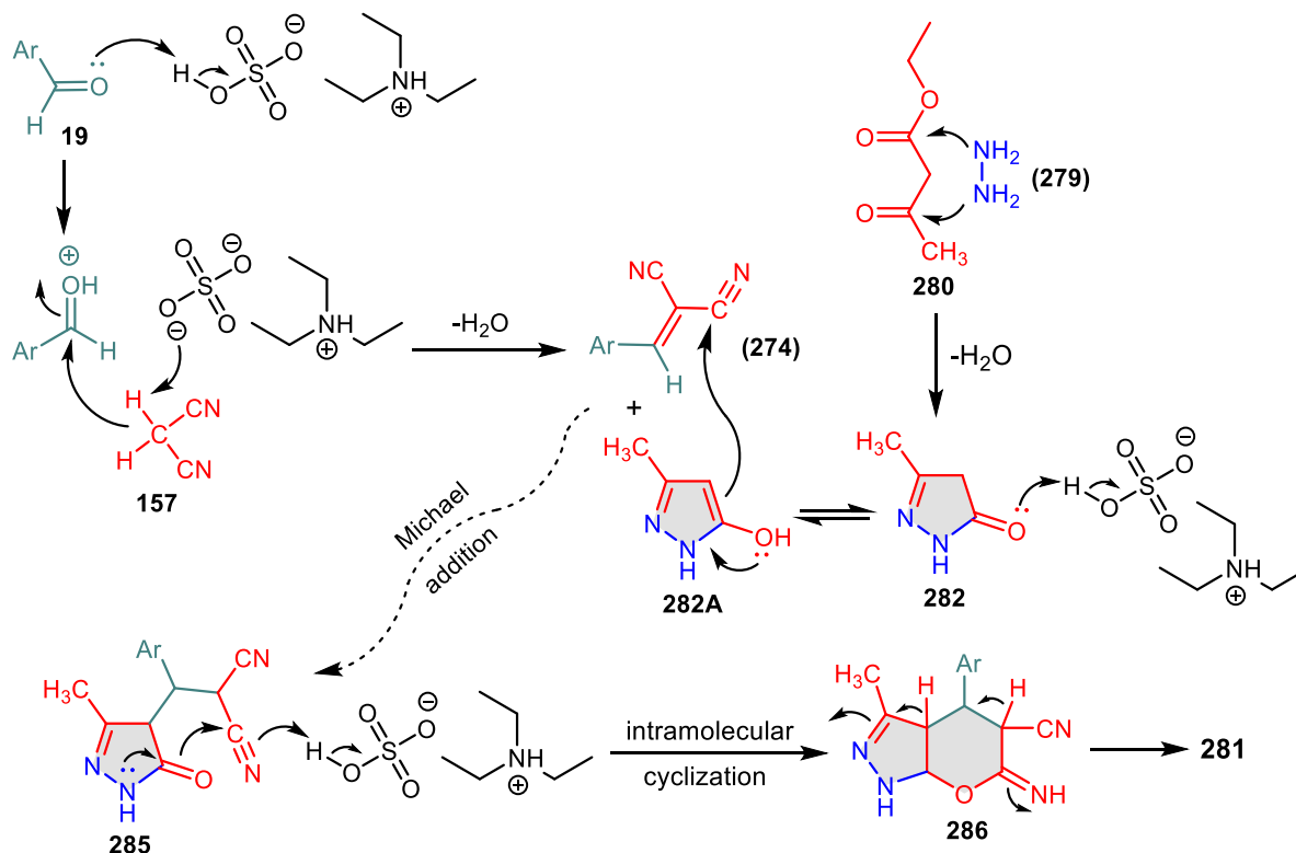
Scheme 64. Mechanism describing the formation of dihydropyrano[2,3- c ]pyrazoles 281 .
