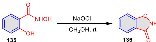
Scheme 32. Synthesis of 1,2-benzisoxazole-3-one ( 136 ).
