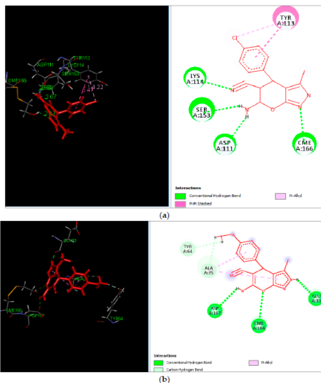
Figure 33. Binding poses and molecular interactions of (a) compound 281a and (b) compound 281b into the active site of tubulin. Reproduced from Ref.; 226 Copyright 2017; MDPI.
