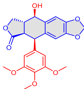
Figure 34. Structure of anti-cancer drug podophyllotoxin.
