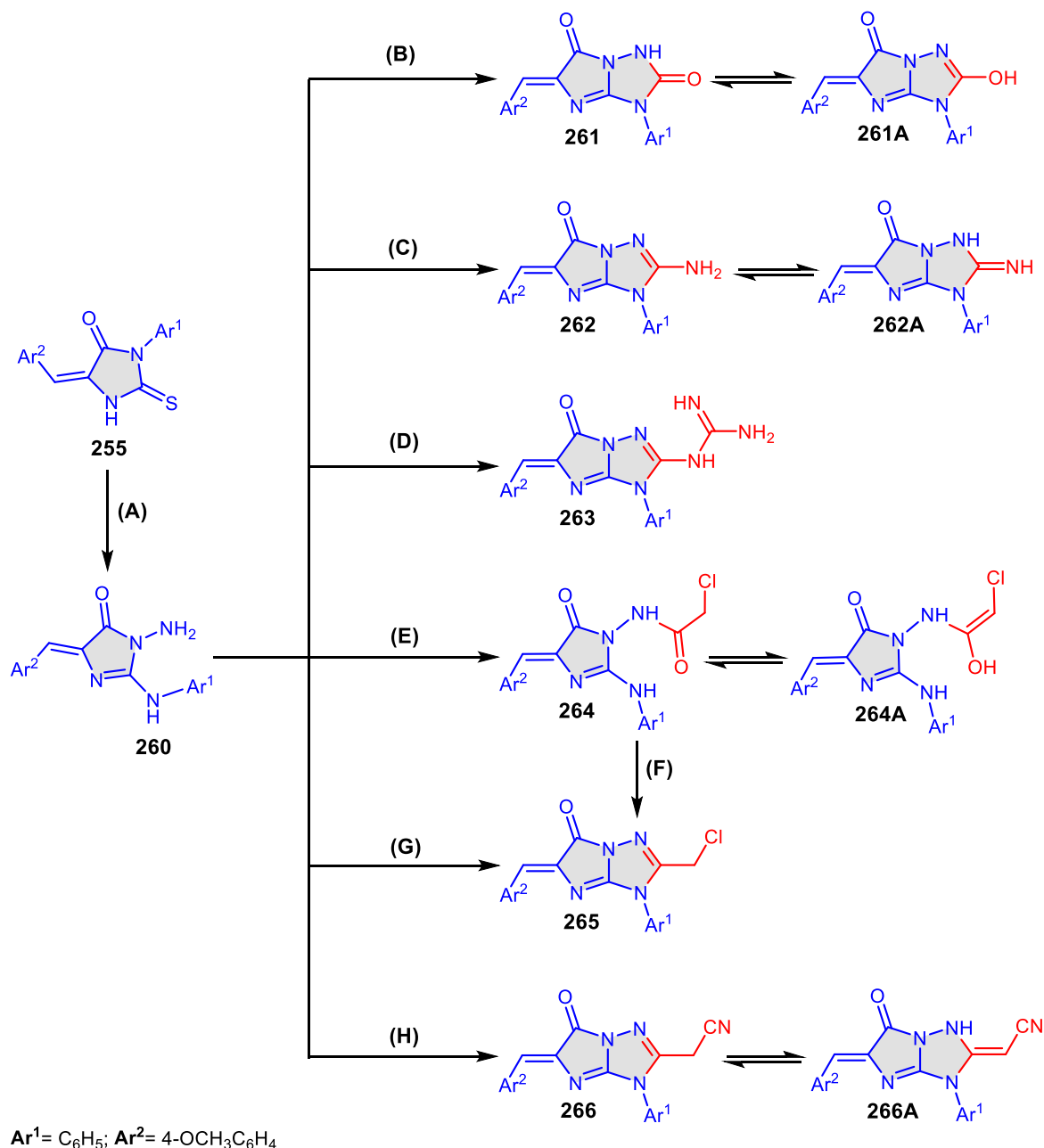
Scheme 57. Synthesis of compounds 260-266 . Reagents and conditions: A) hydrazine hydrate, ethanol, reflux ( 260 ); B) ethyl chloroformate, fusion ( 261 ); C) cyanamide, fusion ( 262 ); D) cyanoguanidine, fusion ( 263 ); E) chloroacetyl chloride, dioxane, reflux ( 264 ); F) fusion ( 265 ); G) chloroacetyl chloride, reflux ( 265 ); H) ethyl cyanoacetate, fusion ( 266 ).
