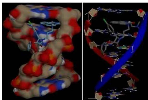
Figure 31. Molecular docking model of DNA with \beta -lactam 247 . Reproduced from Ref., 188 Copyright 2019; Wiley.
