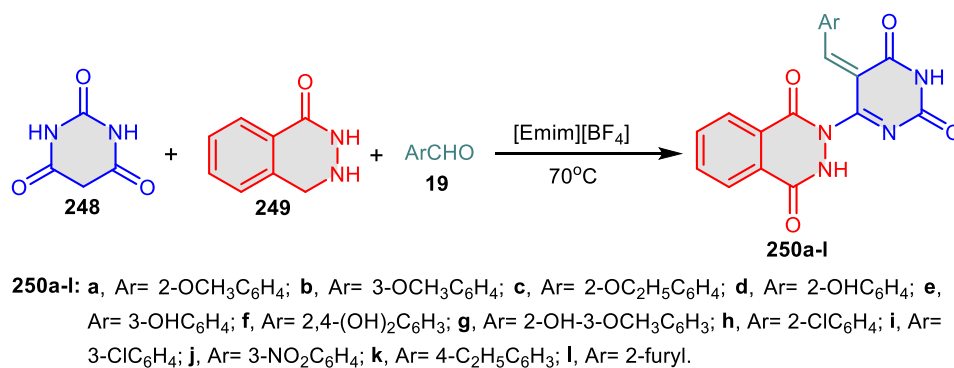
Scheme 54. Synthesis of tetrahydropyrimidin-4-yl-2,3-dihydrophthalazine-1,4-diones 250a-l .
