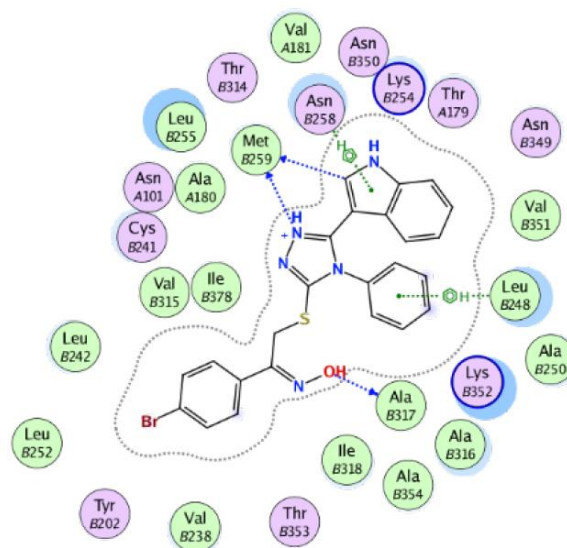
Figure 25. Ligplots at \alpha/\beta -tubulin colchicine binding site: 2D-docked model of 187i . Reproduced with permission from Ref.; 156 Copyright 2025; MDPI.
