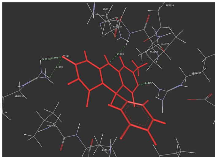
Figure 38. A significant interaction of molecule 354c with MPO. Reproduced from Ref., 284 Copyright 2022; Taylor & Francis.
