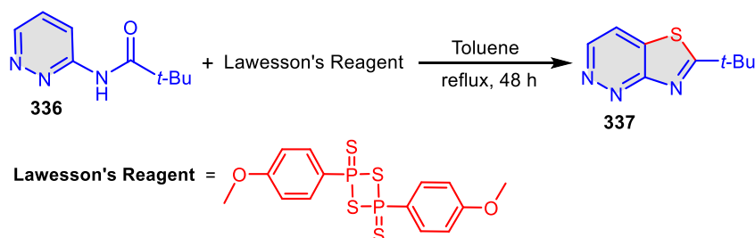
Scheme 77. Synthesis of thiazolo[4,5-c]pyridazine 337 .
