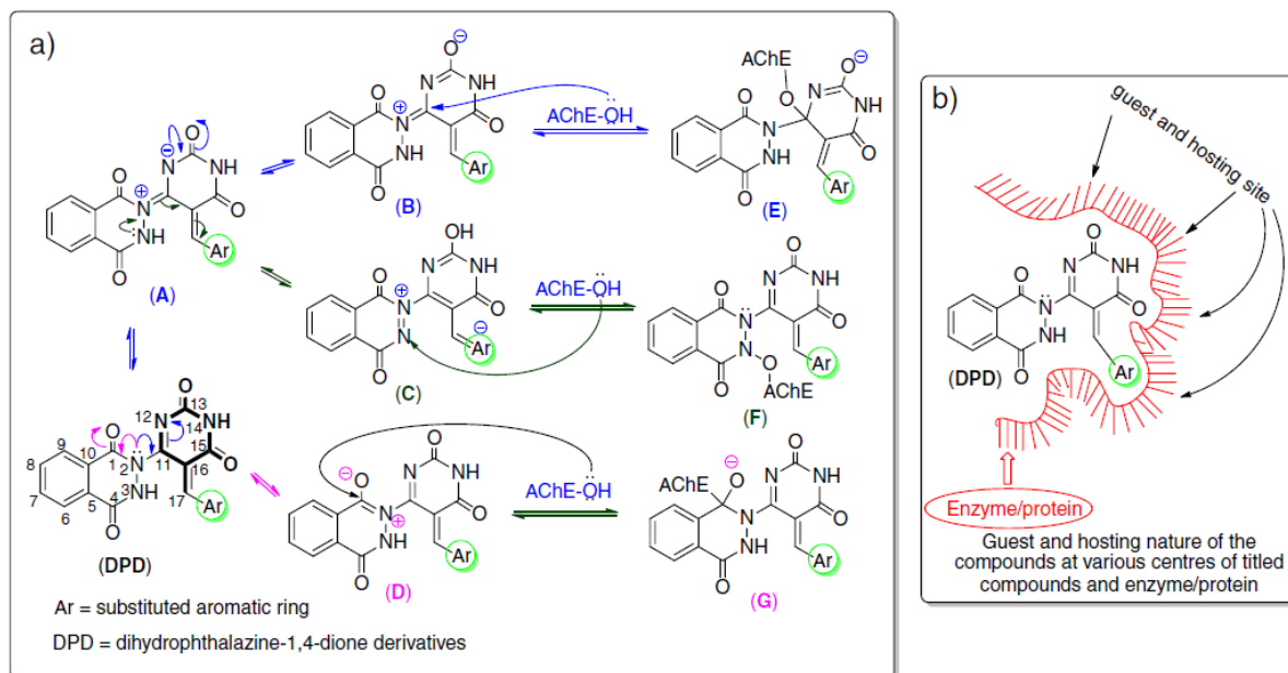
Figure 32. a) Schematic presentation of bio-active pharmacophore unit of dihydrophthalazine-1,4-dione derivatives, b) possible guest and hosting nature of the title compounds ( 250a–l ): mechanistic hypothetical presentation. Reproduced from Ref.; 193 Copyright 2018; Wiley.
