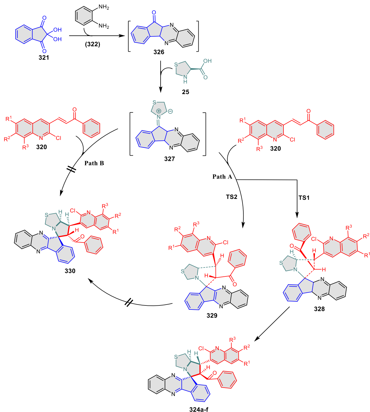
Scheme 75. A plausible mechanism for spiro-indeno[1,2- b ]quinoxaline-pyrrolothiazoles 324a-f .
