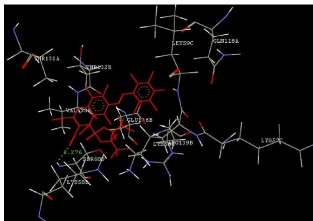
Figure 23. Binding interaction of compound 159l . Reproduced with permission from Ref., 134 Copyright 2019; Springer.
