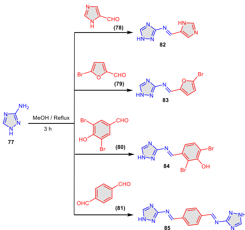
Scheme 19. Synthesis of the 1,2,4-triazole Schiff bases 82–85 .
