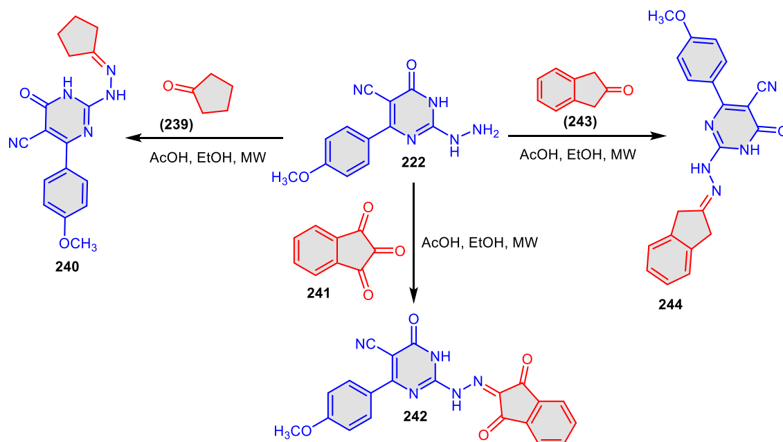
Scheme 52. Synthesis of pyrimidine derivatives 240 , 242 and 244 .
