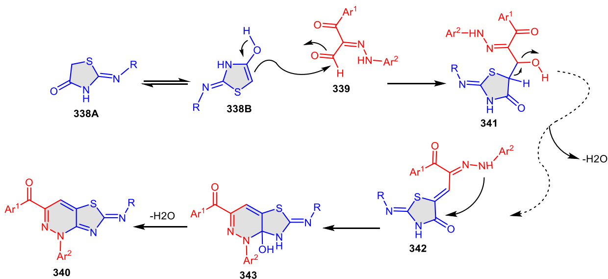
Scheme 79. A plausible mechanism for the formation of 340 .
