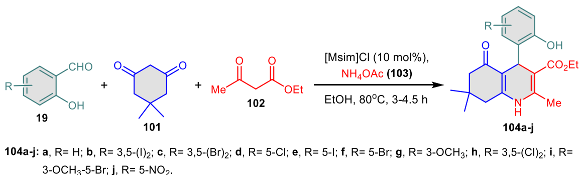
Scheme 23. Synthesis of polyhydroquinoline derivatives 104a-j .
