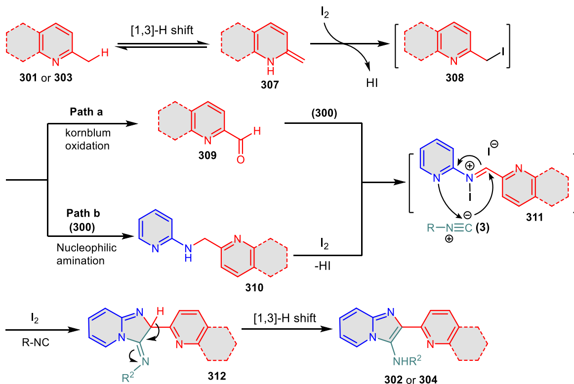
Scheme 71. Mechanism for the iodine-catalyzed oxidative condensation to produce 302 and 304 .
