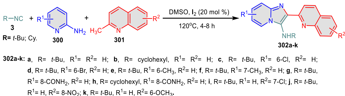
Scheme 68. Iodine-catalyzed reaction for the formation of diversity of 3-aminoimidazo[1,2- a ]pyridines 302a-k .
