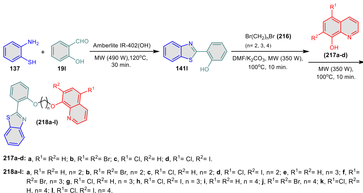
Scheme 48. Synthesis of novel benzothiazole–quinolines 218a-l .
