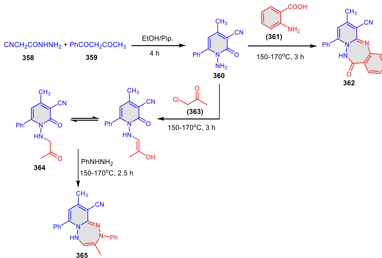
Scheme 85. Synthesis of 1,2,4-triazepine 362 and 1,2,4,5-tetrazepines 365 .
