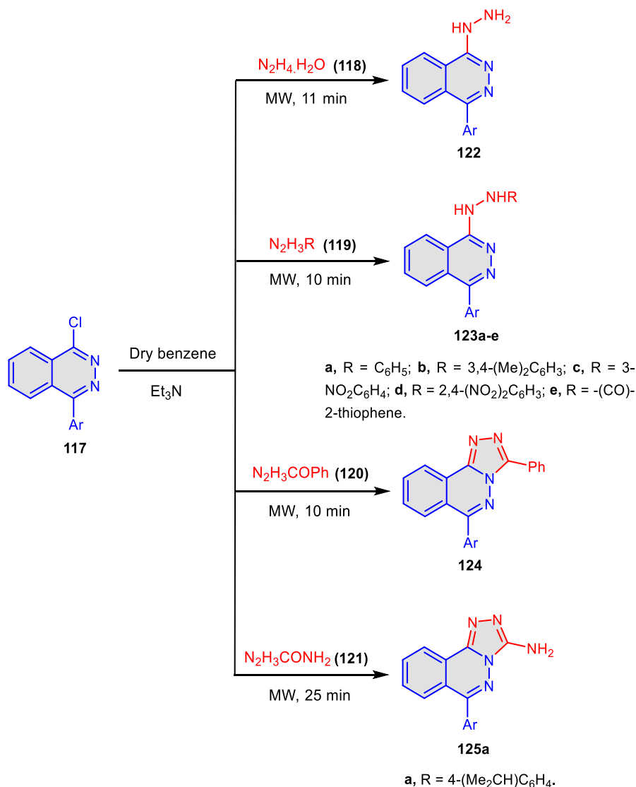
Scheme 29. Synthesis of diverse phthalazine derivatives 122-125 .
