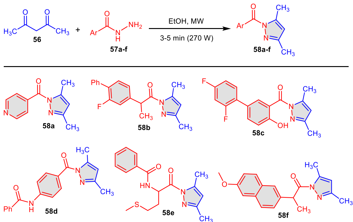
Scheme 14. Synthesis of 1-aryl-3,5-dimethyl-1H-pyrazoles 58a-f .
