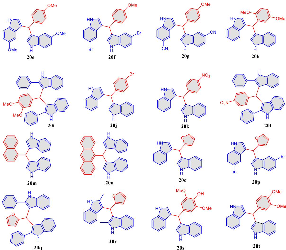
Scheme 5. Synthesis of indolomethanes 20a-t under neat conditions.
