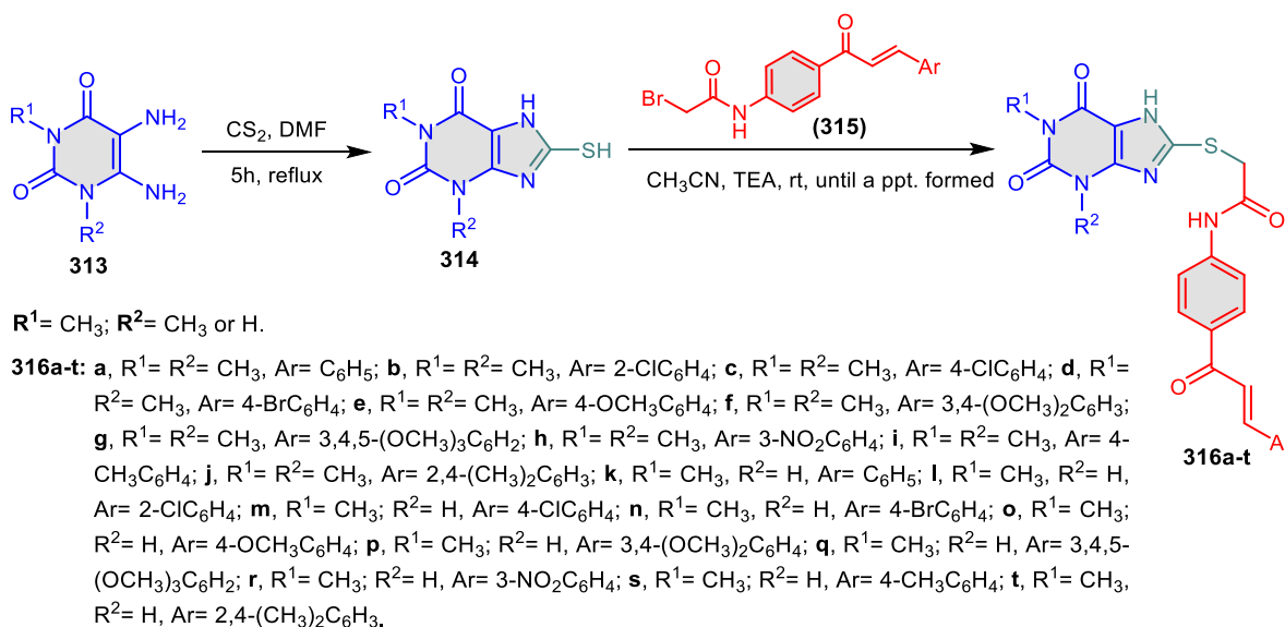
Scheme 72. Synthesis of hybrid chalcone substituted xanthines 316a-t .
