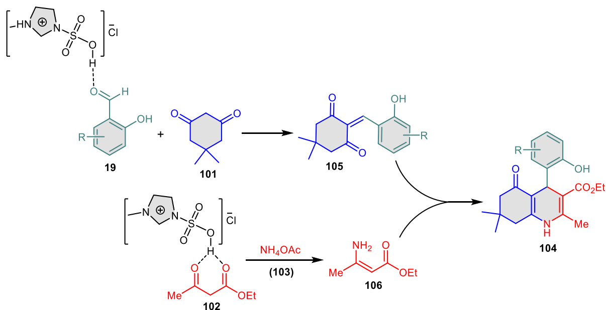
Scheme 24. A plausible mechanism for the synthesis of polyhydroquinolines 104 .
