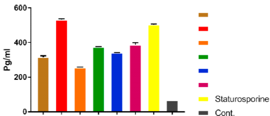
Figure 35. Caspase-3 for compounds 316b (brown), 316c (red), 316e (orange), 316f (green), 316h (blue), 316o (pink) and Staurosporine in (Panc-1). Reproduced with permission from Ref.; 243 Copyright 2019; Elsevier.
