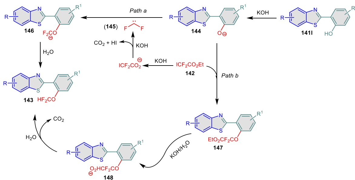
Scheme 35. A plausible mechanism for the difluoromethoxylation.
