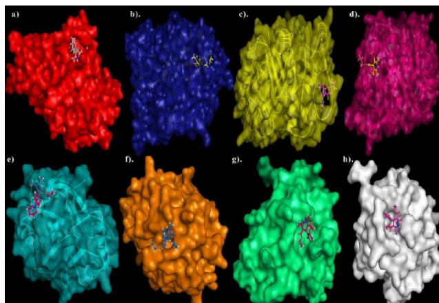
Figure 15. Docking interaction between synthesized compounds ligands 95b , 95f , 95h , and 96j and its proteins (3UT5 and 5TVQ) images produced from Pymol. a) 3UT5 with derivative 95b ; b) 3UT5 with derivative 95f ; c) 3UT5 with derivative 95h ; d) 3UT5 with derivative 96j ; e) 5TVQ with derivative 95b ; f) 5TVQ with derivative 95f ; g) 5TVQ with derivative 95h ; h) 5TVQ with derivative 96j . Reproduced from Ref., 83 Copyright 2022; Wiley.
