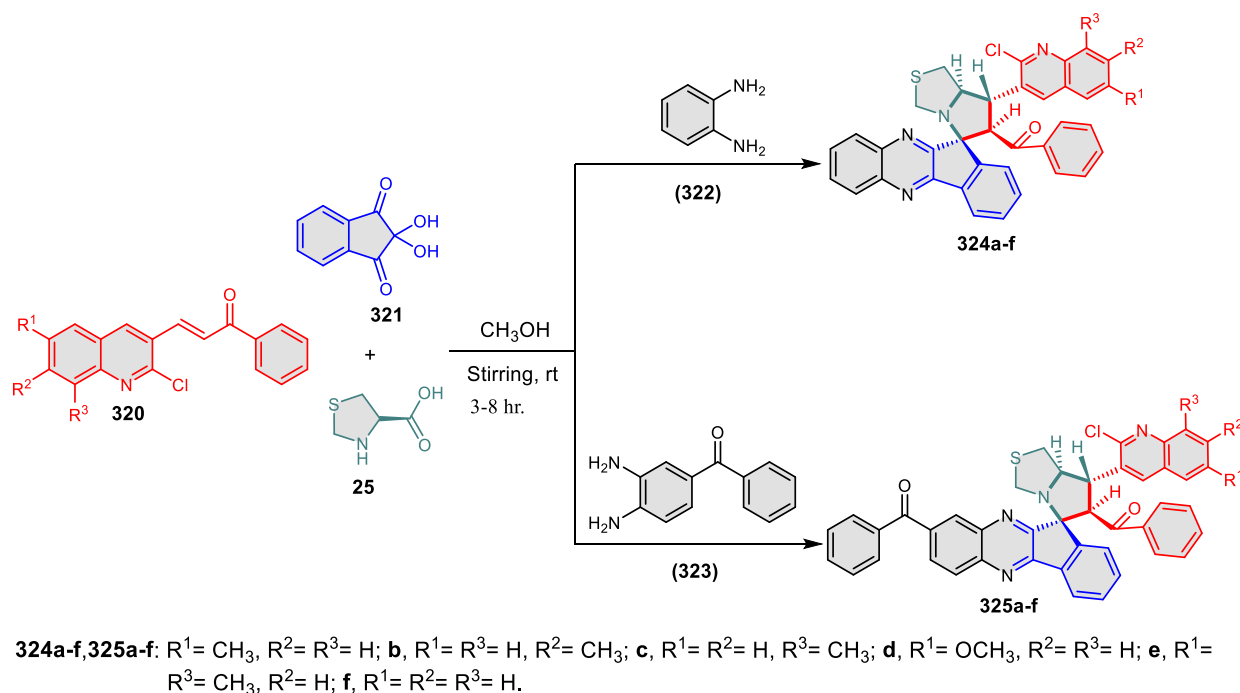
Scheme 74. One-pot four-component synthesis of spiro-indeno[1,2- b ]quinoxaline 324a-f and 325a-f .
