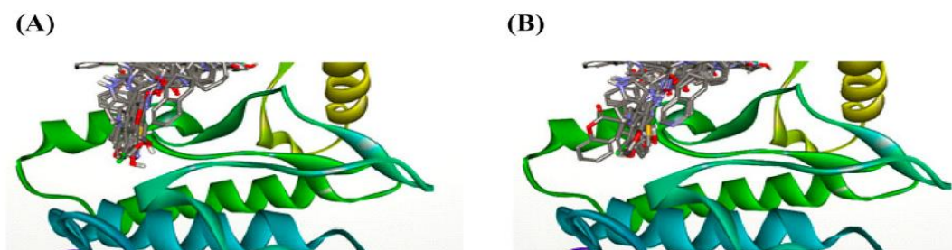
Figure 16. The ligands docked globally on the left (A) versus locally on the right (B). Reproduced with permission from Ref.; 87 Copyright 2020; Taylor & Francis.
