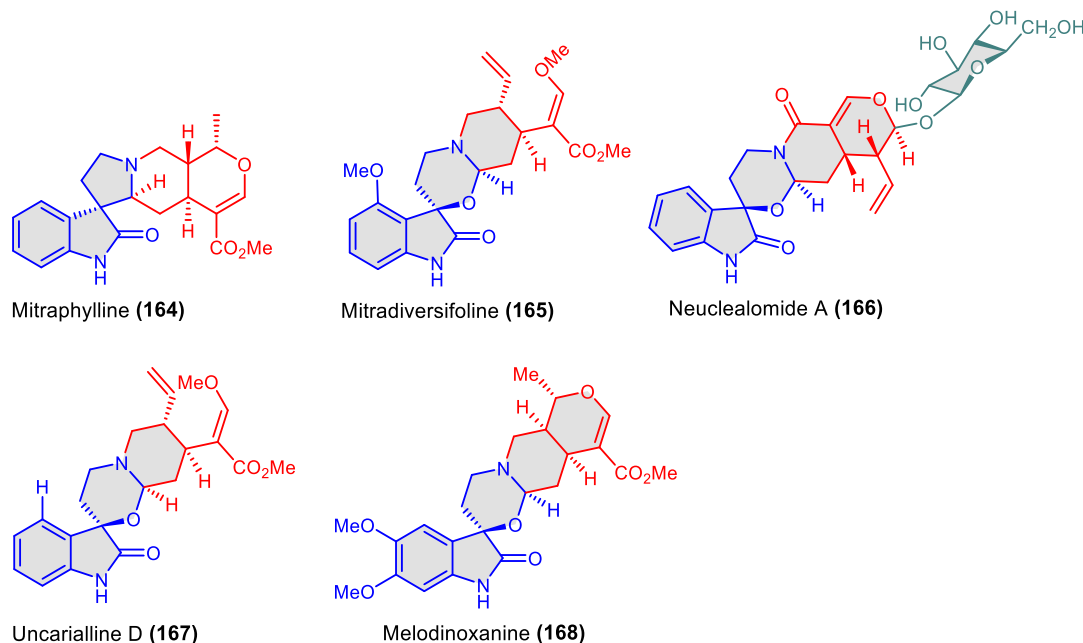
Figure 24. Structure of naturally occurring spiro-oxindoles 164-168 .
