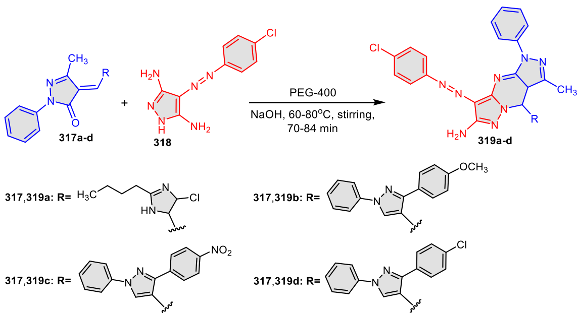
Scheme 73. Synthesis of pyrazolo[1,5- a ]pyrimidine derivatives 319a-d .
