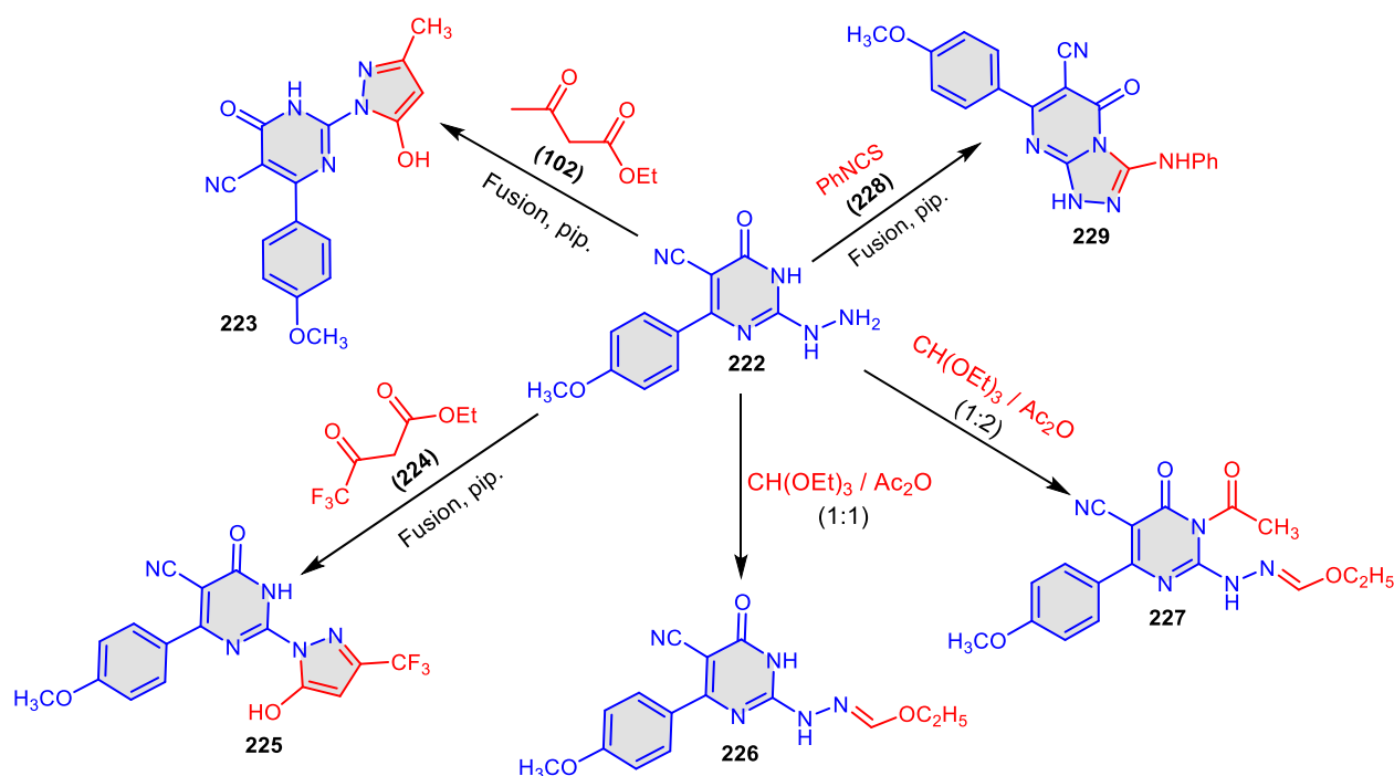
Scheme 50. Synthesis of pyrimidine derivatives 223 , 225 , 226 , 227 and 229 .
