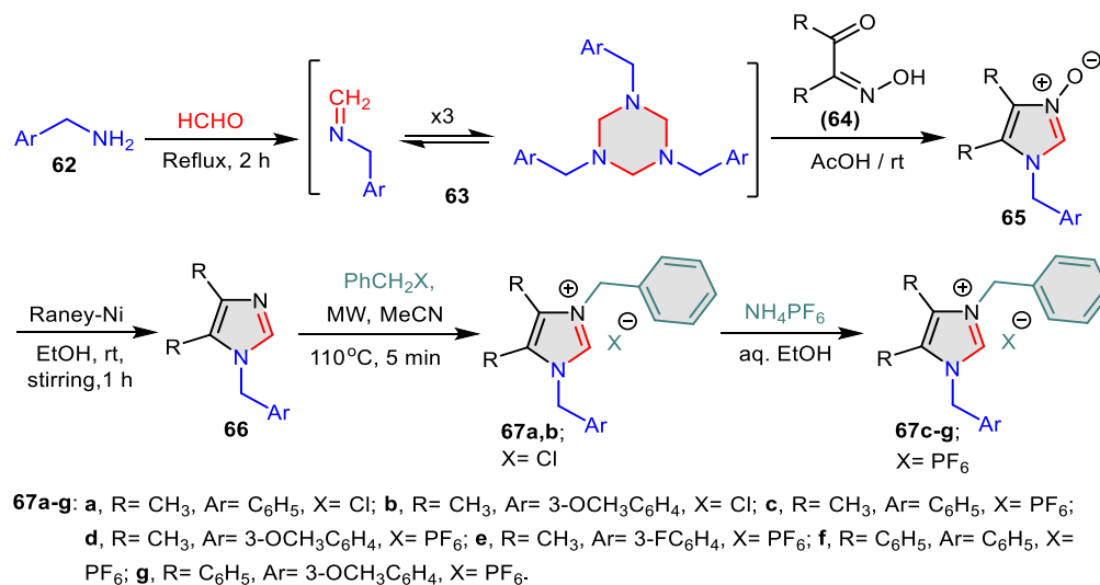
Scheme 16. Synthesis of lipidilene analogues 67a-g .
