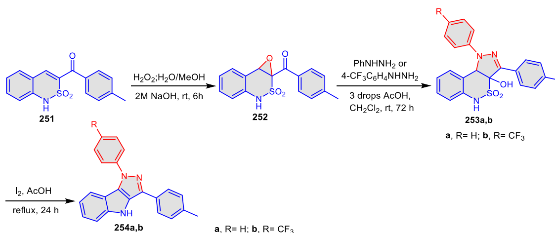
Scheme 55. Multi step reaction for the synthesis of pyrazolo[4,3- b ]indoles 254a,b .
