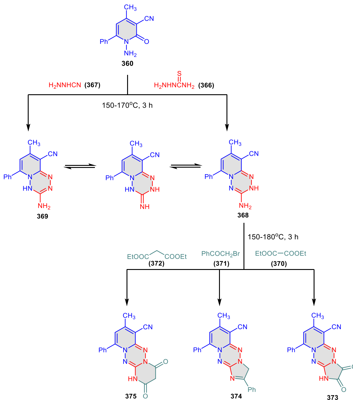
Scheme 86. Synthesis of 1,2,4,5-tetrazines 368 , 369 and 373-375 .
