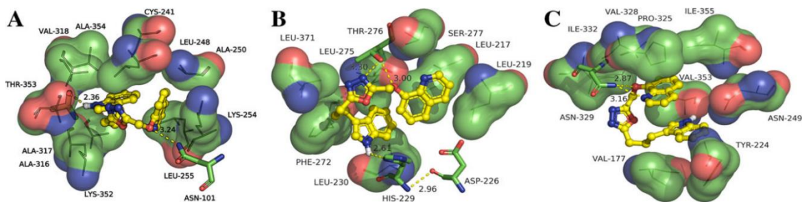
Figure 27. Computational docking models: 203d docked at A colchicine, B paclitaxel, and C vinblastine sites of tubulin. Reproduced from Ref.; 166 Copyright 2016; Springer.
