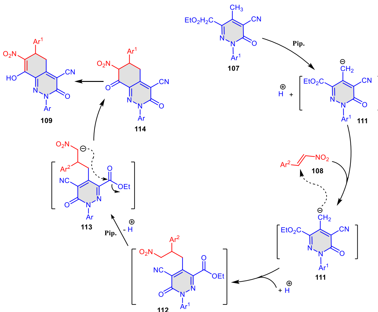
Scheme 26. Mechanism for the formation of polyfunctionally substituted cinnoline 109 .
