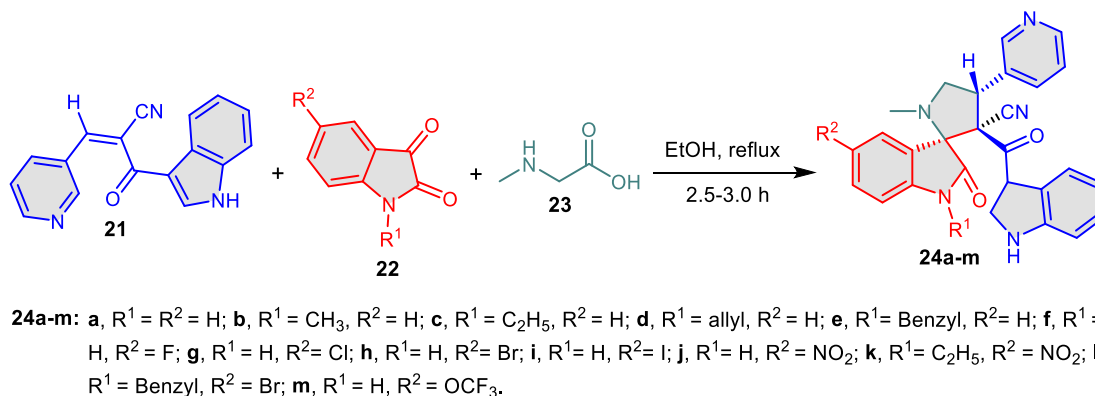
Scheme 6. Synthesis of spirooxindole–pyrrolidine derivatives 24a–m .
