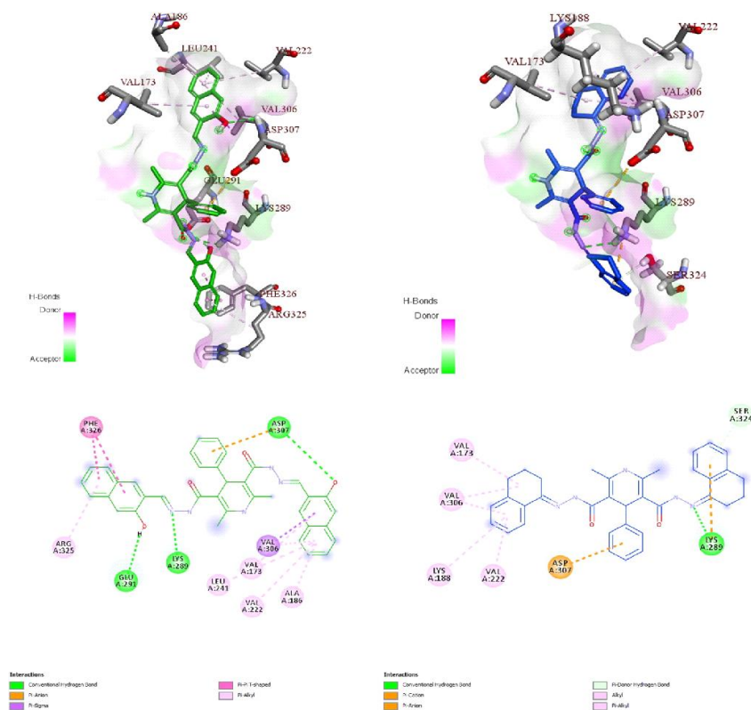
Figure 18. Compounds 99e and 100e interactions on the left and right sides respectively (2D over the bottom and 3D on the top). Reproduced with permission from Ref.; 87 Copyright 2020; Taylor & Francis.
