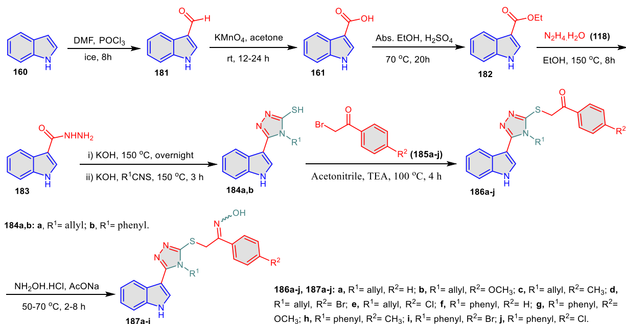
Scheme 41. Synthesis of indole-based 1,2,4-triazole hybrids 187a-j .
