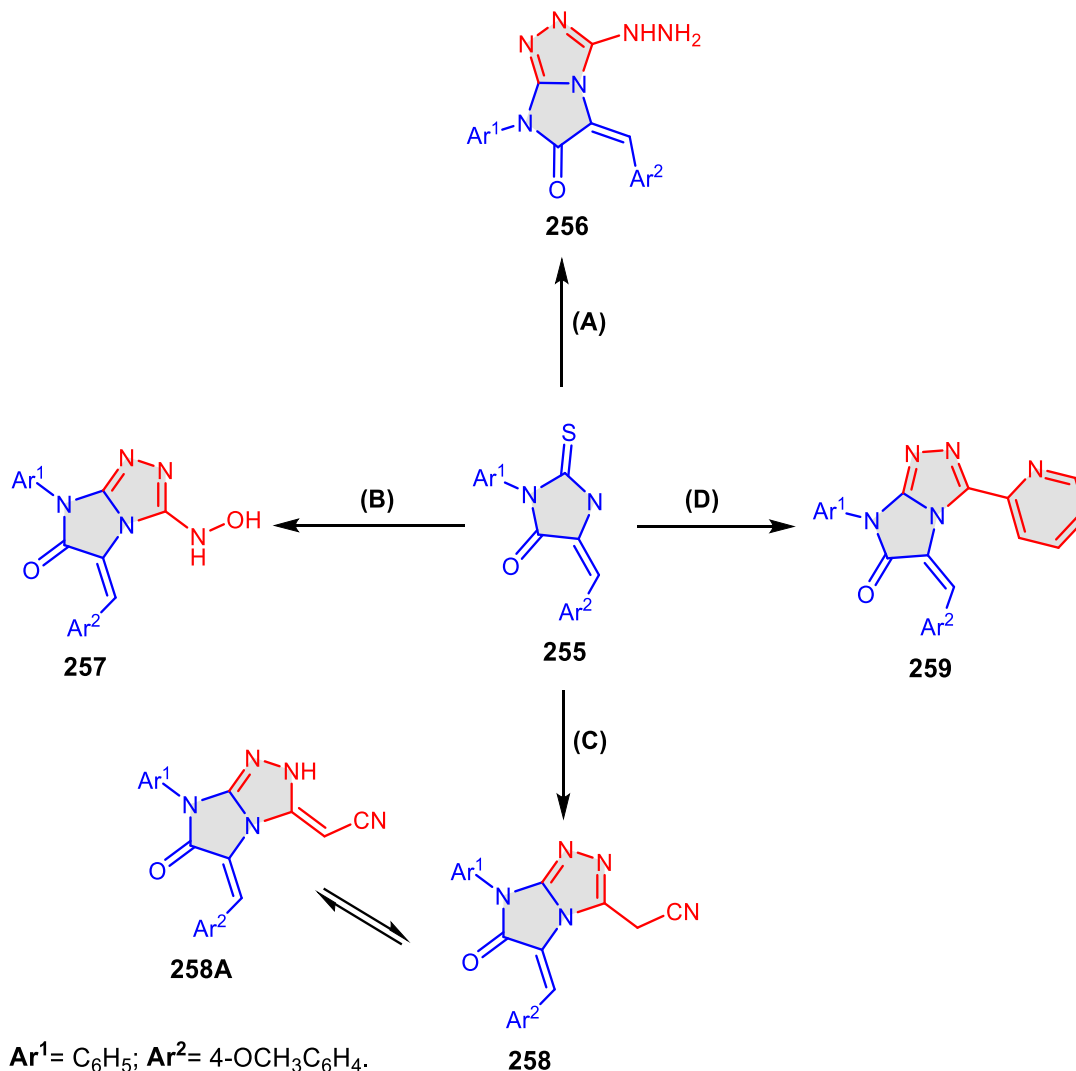
Scheme 56. Synthesis of compounds 256–259 . Reagents and conditions: A) thiocarbohydrazide, fusion ( 256 ); B) N -hydroxyhydrazinecarbo-thioamide hydrochloride, fusion ( 257 ); C) cyanoacetohydrazide, fusion ( 258 ); D) picolinohydrazide, fusion, 6 h, ( 259 ).
