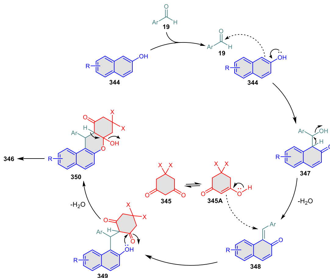
Scheme 81. A convenient mechanism for the formation of 346 .
