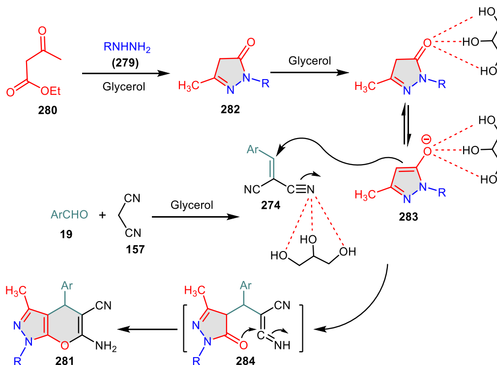
Scheme 62. Mechanism illustrate the formation of pyrano[2,3- c ]-pyrazoles 281 .
