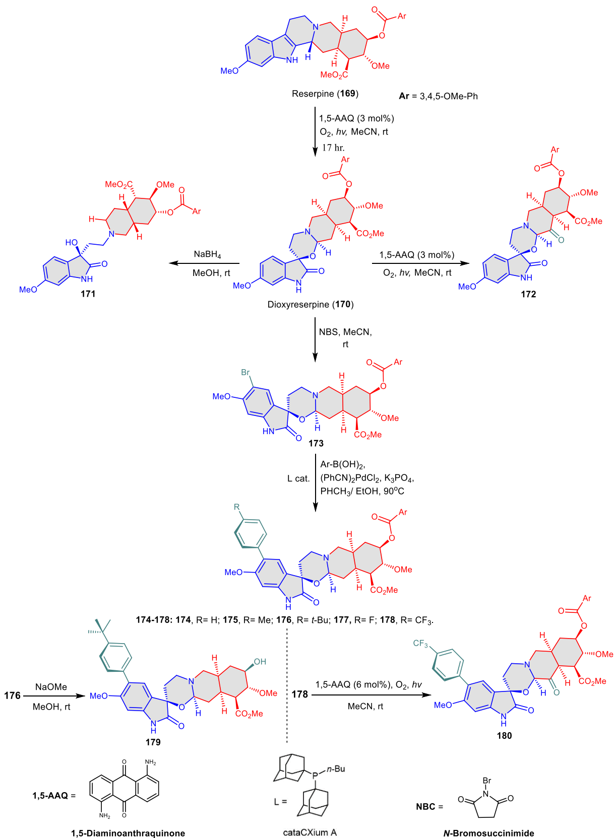
Scheme 40. Synthesis of dioxyreserpine ( 170 ), which transformed to analogous 171-180 via further functionalization.
