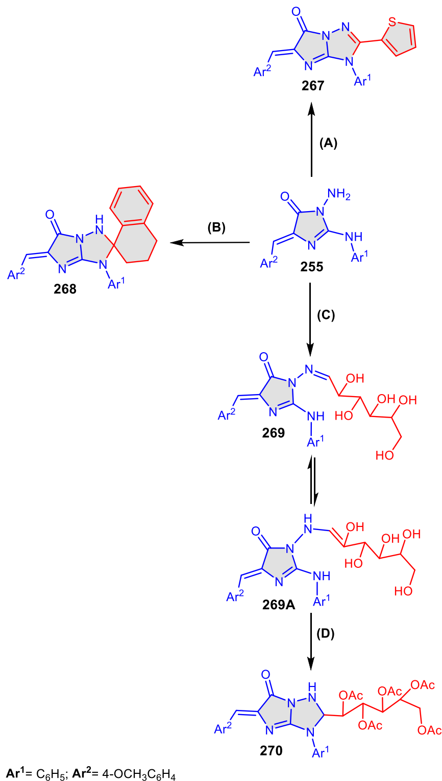
Scheme 58. Synthesis of compounds 267-271 . Reagents and conditions: A) thiophen-2-carbonyl chloride, pyridine, reflux ( 267 ); B) 1-tetralone, glacial acetic acid, reflux ( 268 ); C) glucose, glacial acetic acid, H 2 O, ethanol, reflux ( 269 ); D) acetic anhydride, reflux ( 270 ).
