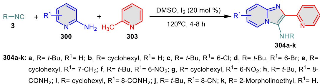
Scheme 69. Synthesis of various 3-aminoimidazo[1,2- a ]pyridines 304a-k .
