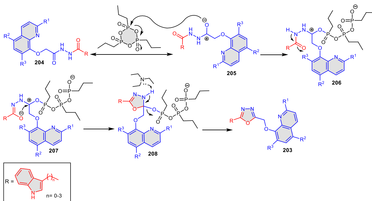
Scheme 46. Mechanism for the formation of hybrid quinoline-indole-oxadiazole molecules 203 .
