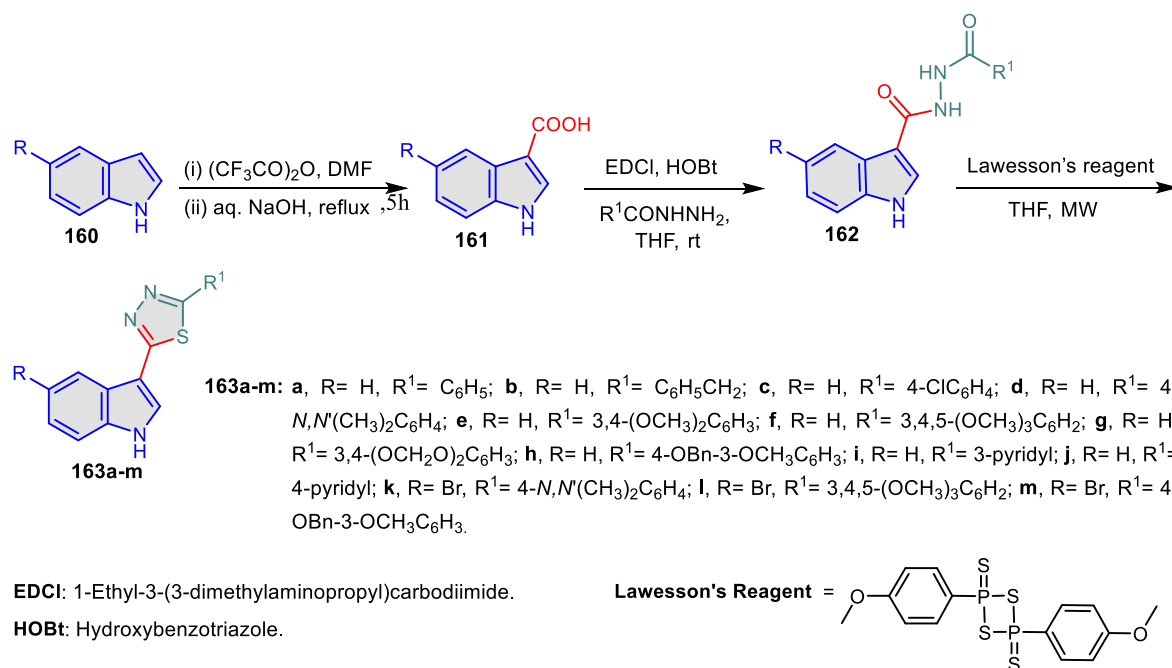
Scheme 39. Formation of 5-(3-indolyl)-1,3,4-thiadiazole derivatives 163a-m .
