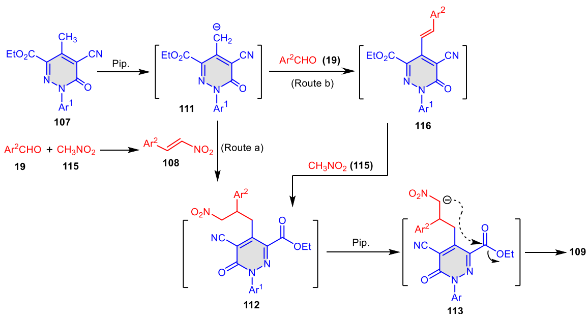
Scheme 28. Proposed mechanism for the formation cinnolines 109 of via multi-component reaction.
