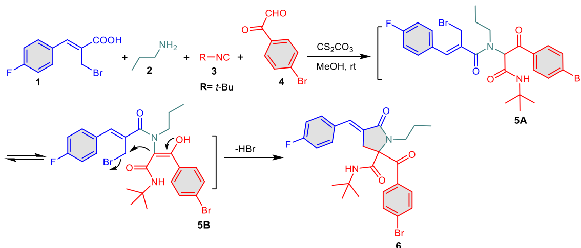
Scheme 1. Synthesis of ( E )-2-(4-bromobenzoyl)- N -( tert -butyl)-4-(4-fluorobenzylidene)-5-oxo-1-propylpyrrolidine-2-carboxamide ( 6 ).
