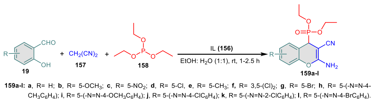
Scheme 38. Synthesis of substituted chromene derivatives 159a-l .
