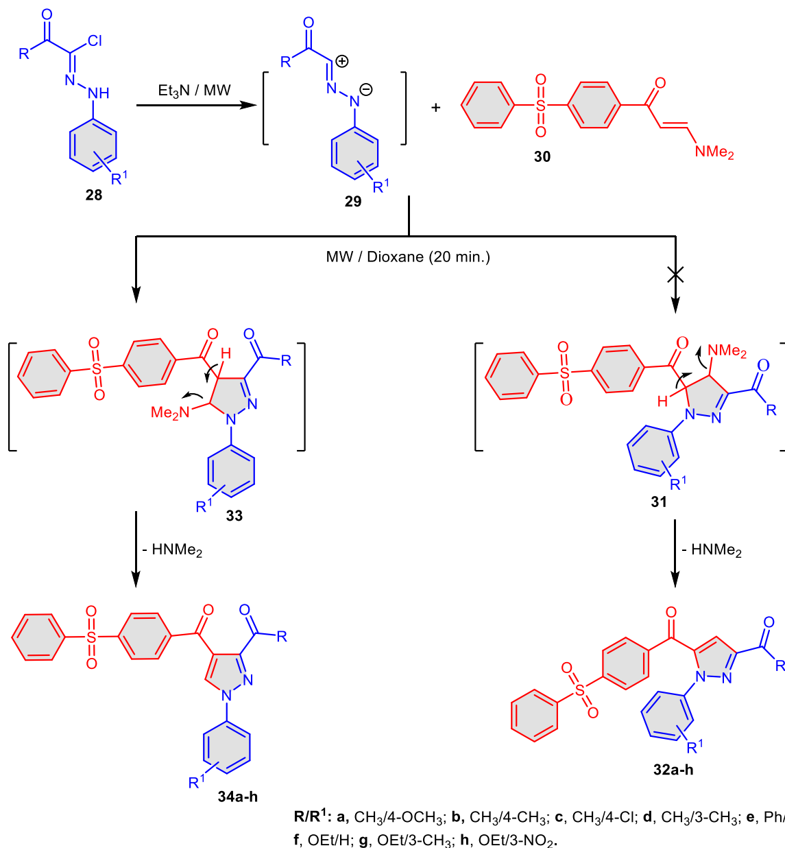
Scheme 10. Synthesis of pyrazoles 34a-h bearing phenylsulfone moiety.
