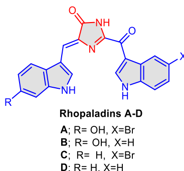
Figure 1. Structure of marine alkaloids rhopaladins A-D .
