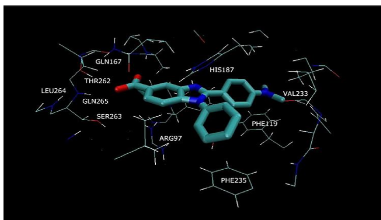
Figure 11. Molecular interactions between 71j and SIRT2. Reproduced with permission from Ref.; 70 Copyright 2014; Elsevier.
