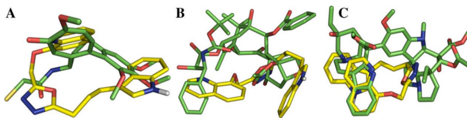
Figure 26. Models of tubulin-bound ligand 203d superimposed on A colchicine, B paclitaxel, and C vinblastine in their matching crystal structures. Carbon (yellow), oxygen (red), and nitrogen (dark blue) in Oxadiazole 203d ; carbon (green), nitrogen (blue), and oxygen (red) in CN2, TXL, and VLB. Reproduced from Ref.; 166 Copyright 2016; Springer.
