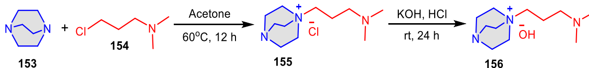
Scheme 37. Synthesis of dual basic ionic liquid 156 .
