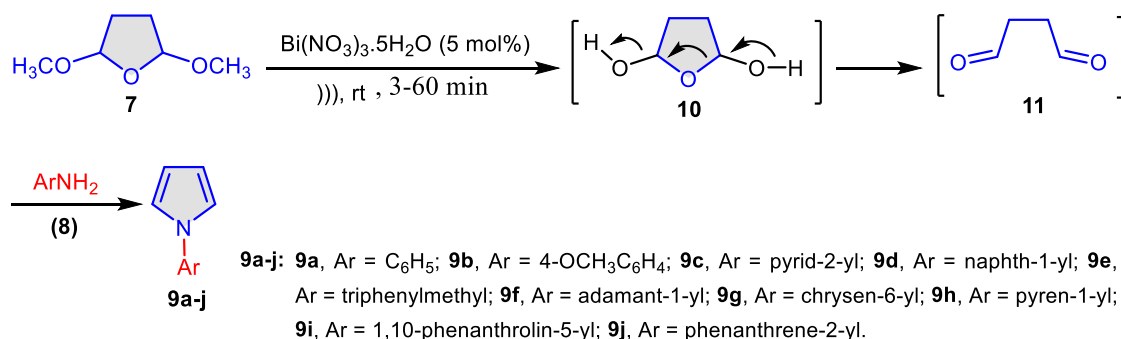
Scheme 2. Synthesis of N -substituted pyrroles 9a–j .
