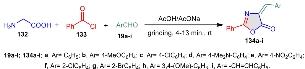
Scheme 31. Multicomponent synthesis of 4-arylidine-2-phenyl-5(4 H )-oxazolones 134a-i .
