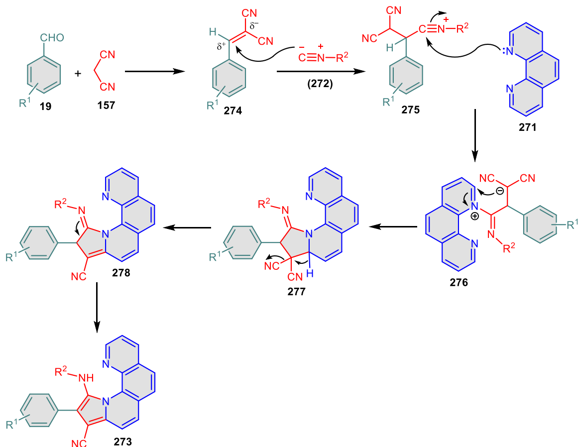
Scheme 60. A suggested mechanism for the formation pyrrolo[1,10]phenanthrolines 273 .
