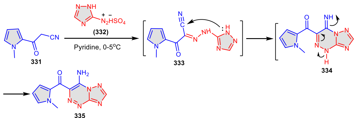
Scheme 76. Synthesis of triazolo[5,1-c][1,2,4]triazine 335 .
