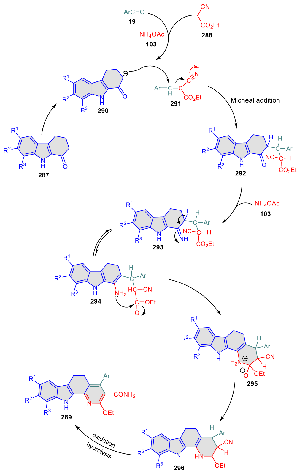
Scheme 66. A plausible mechanism to for the formation of 289 .
