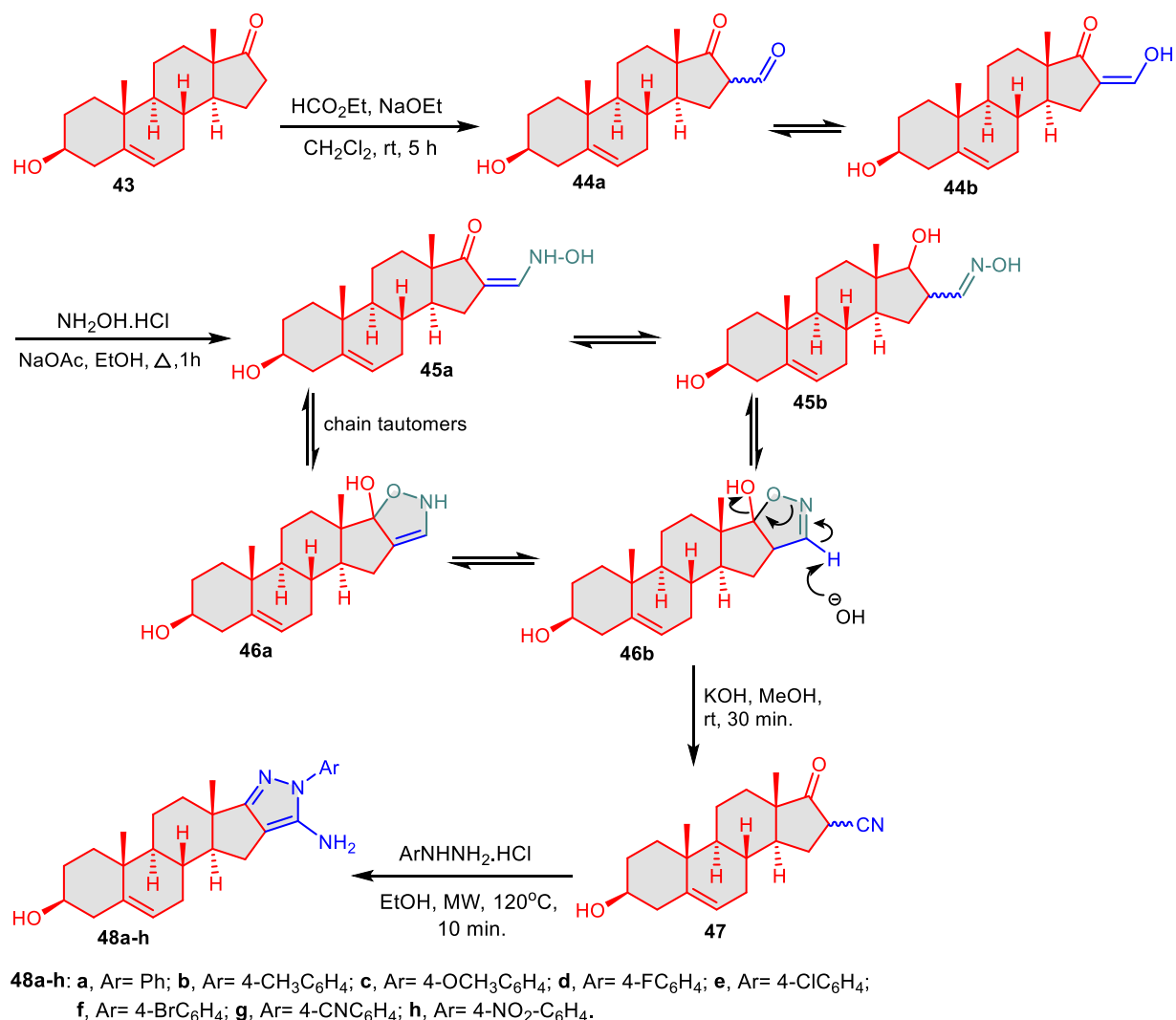
Scheme 11. Formation of 5-amino-1-arylpyrazoles 48a-h based on dehydroepiandrosterone (DHEA).
