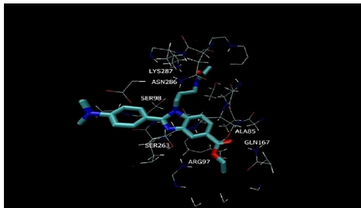
Figure 12. Molecular interactions between 71b and SIRT2. Reproduced with permission from Ref.; 70 Copyright 2014; Elsevier.
