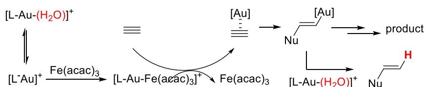
Scheme 2. Conceptual development of Au/Fe cooperative catalysis for redirecting vinyl-gold intermediates from protodeauration to bond construction.
