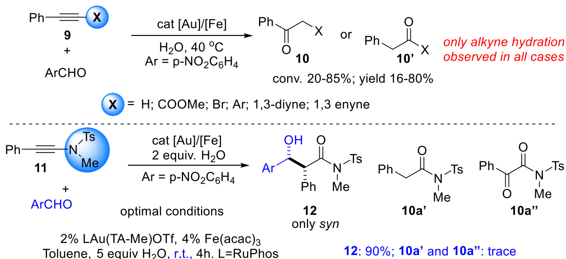
Scheme 3. Extending vinyl-gold nucleophilicity beyond carbonyl-directed substrates.
