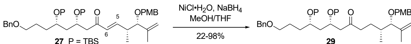
Scheme 12. Conjugate reduction of enone 27 .
