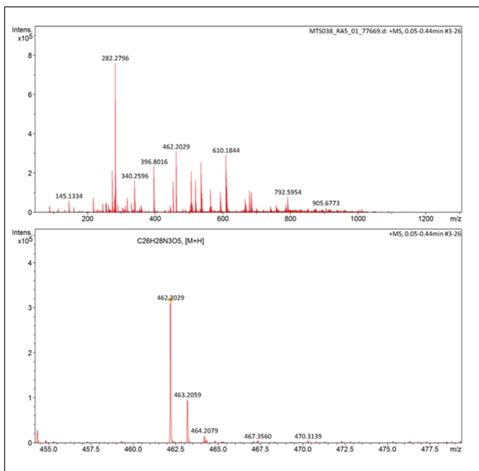
Figure S33. HRMS spectra of ( E )- N -(4-(3-(benzyloxy)-2-methyl-4-oxopyridin-1(4 H )-yl)butyl)-3-(4-nitrophenyl)acrylamide ( 6k ).
