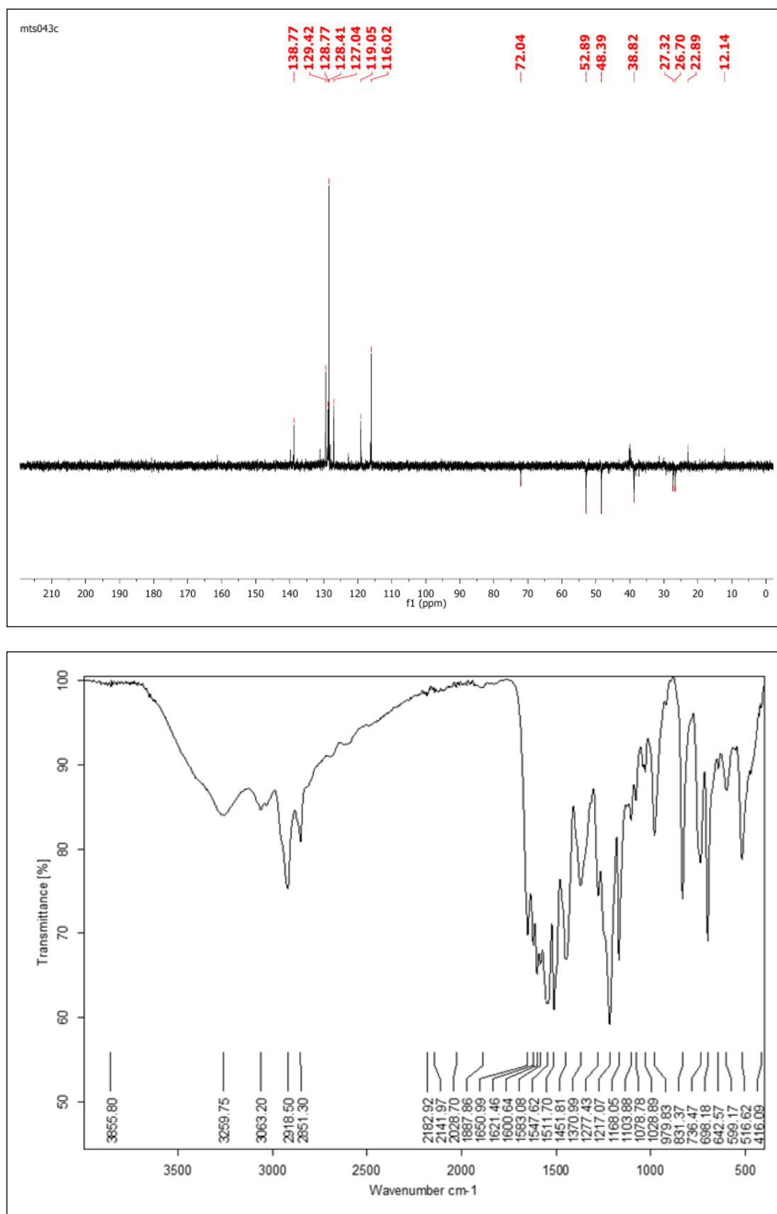
Figure S38. DEPT-135 and IR spectra of ( E )- N -(4-(3-(benzyloxy)-2-methyl-4-oxopyridin-1(4 H )-yl)butyl)-3-(4-hydroxyphenyl)acrylamide ( 6m ).
