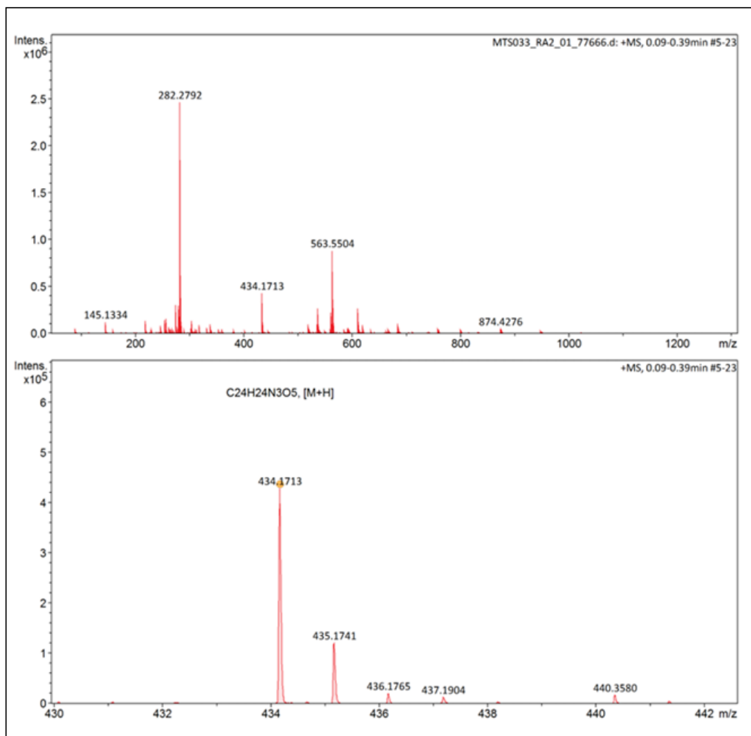
Figure S9. HRMS spectra of (E)-N-(2-(3-(benzyloxy)-2-methyl-4-oxopyridin-1(4H)-yl)ethyl)-3-(4-nitrophenyl)acrylamide ( 6c ).
