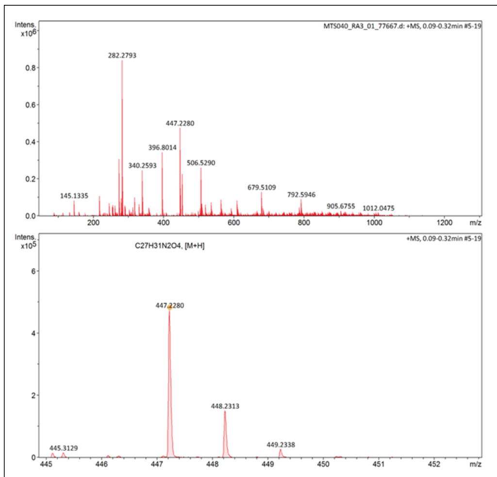
Figure S30. HRMS spectra of ( E )- N -(4-(3-(benzyloxy)-2-methyl-4-oxopyridin-1(4 H )-yl)butyl)-3-(4-methoxyphenyl)acrylamide ( 6j ).
