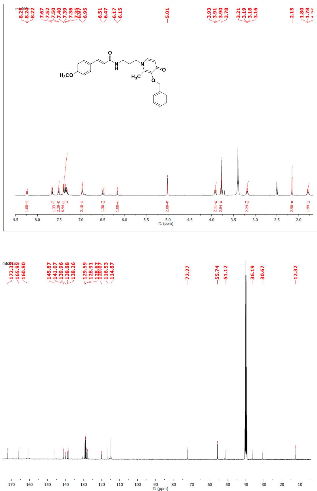
Figure S16. 1 H and 13 C spectra of (E) - N -(3-(3-(benzyloxy)-2-methyl-4-oxopyridin-1(4 H )-yl)propyl)-3-(4-methoxyphenyl)acrylamide ( 6f ).
