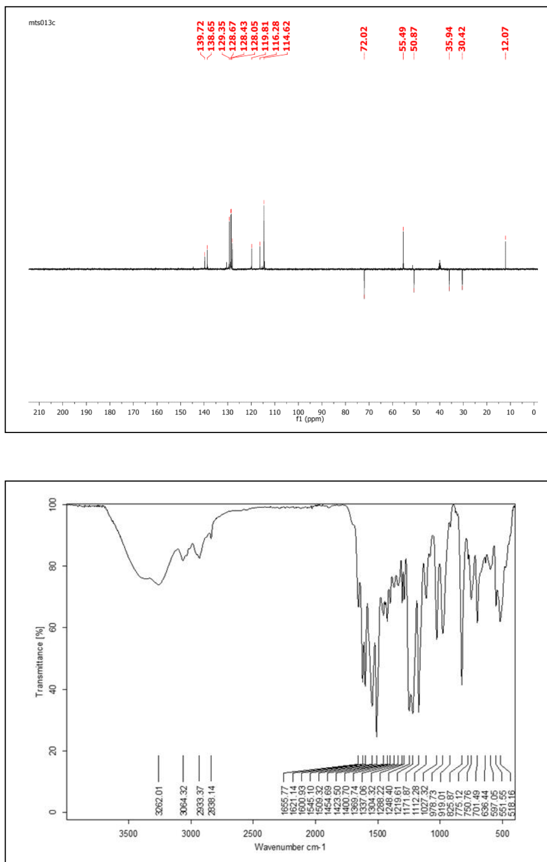
Figure S17. DEPT-135 and IR spectra of ( E )- N -(3-(3-(benzyloxy)-2-methyl-4-oxopyridin-1(4 H )-yl)propyl)-3-(4-methoxyphenyl)acrylamide ( 6f ).
