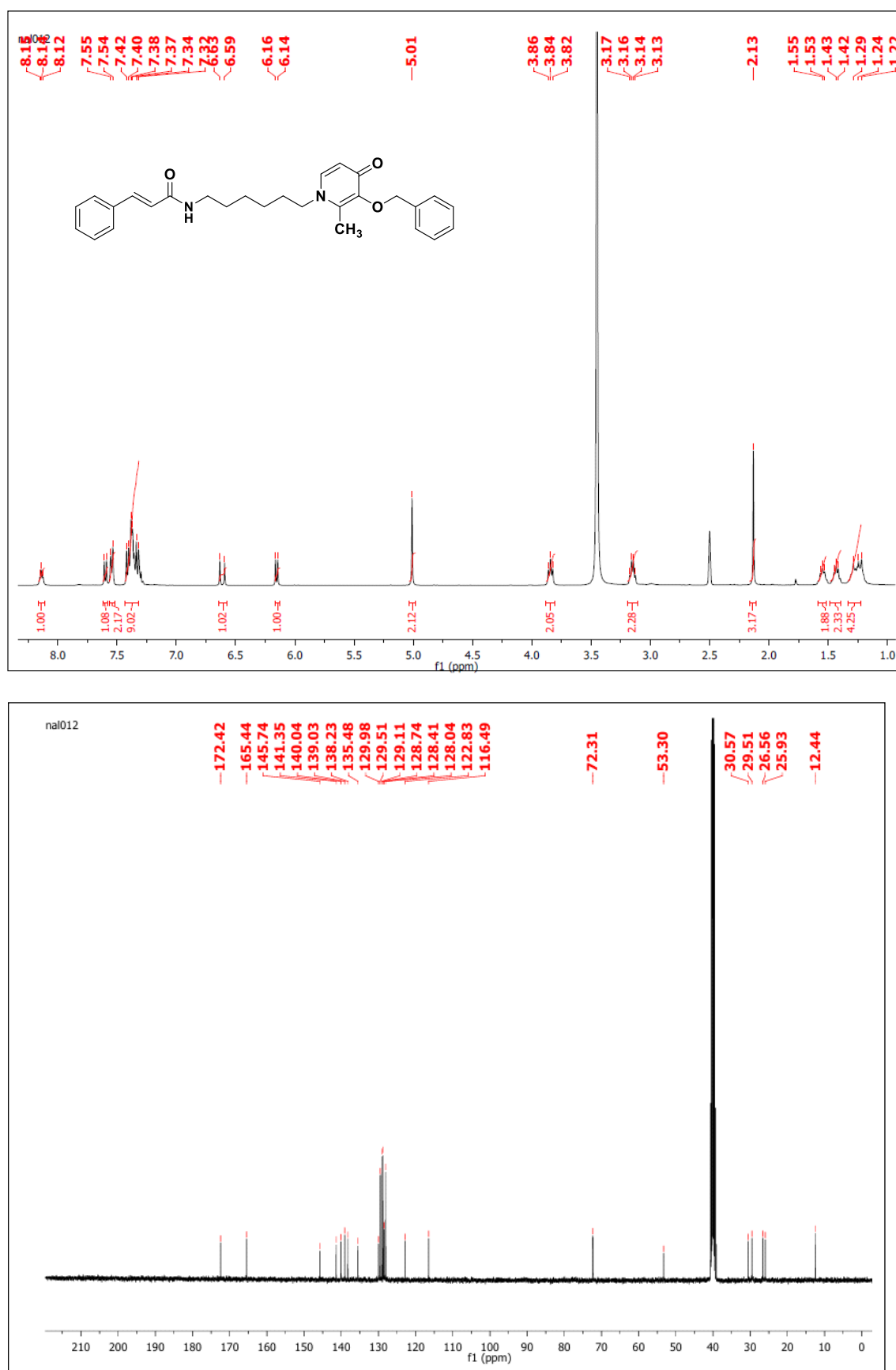
Figure S40. 1 H and 13 C spectra of N -(6-(3-(benzyloxy)-2-methyl-4-oxopyridin-1(4H)-yl)hexyl)cinnamamide ( 6n ).
