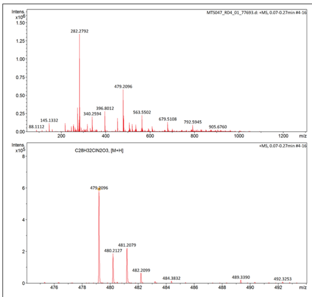
Figure S51. HRMS spectra of ( E )- N -(6-(3-(benzyloxy)-2-methyl-4-oxopyridin-1(4 H )-yl) hexyl)-3-(4-chlorophenyl)acrylamide ( 6q ).
