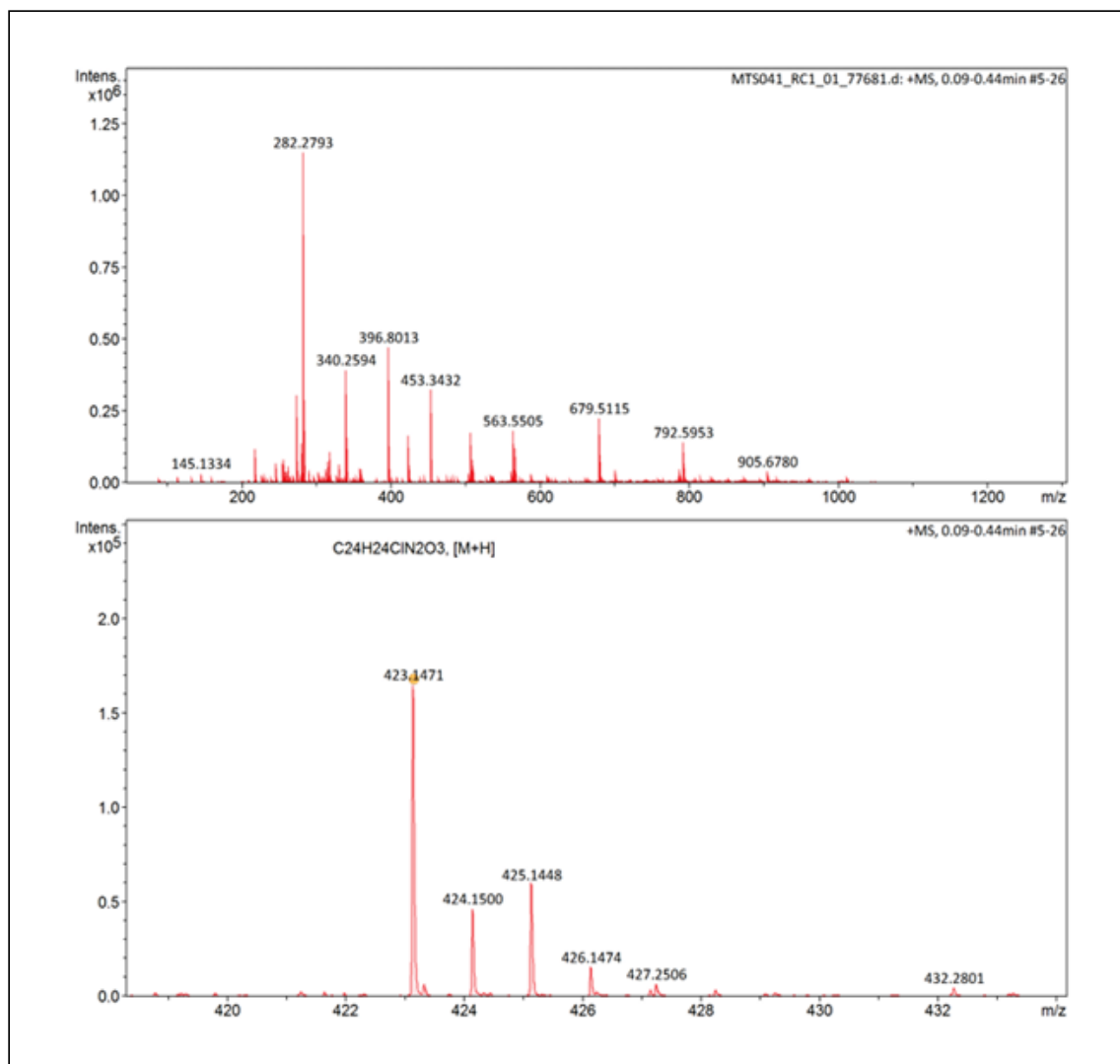
Figure S12. HRMS spectra of ( E )- N -(2-(3-(benzyloxy)-2-methyl-4-oxopyridin-1(4 H )-yl)ethyl)-3-(4-chlorophenyl)acrylamide ( 6d ).
