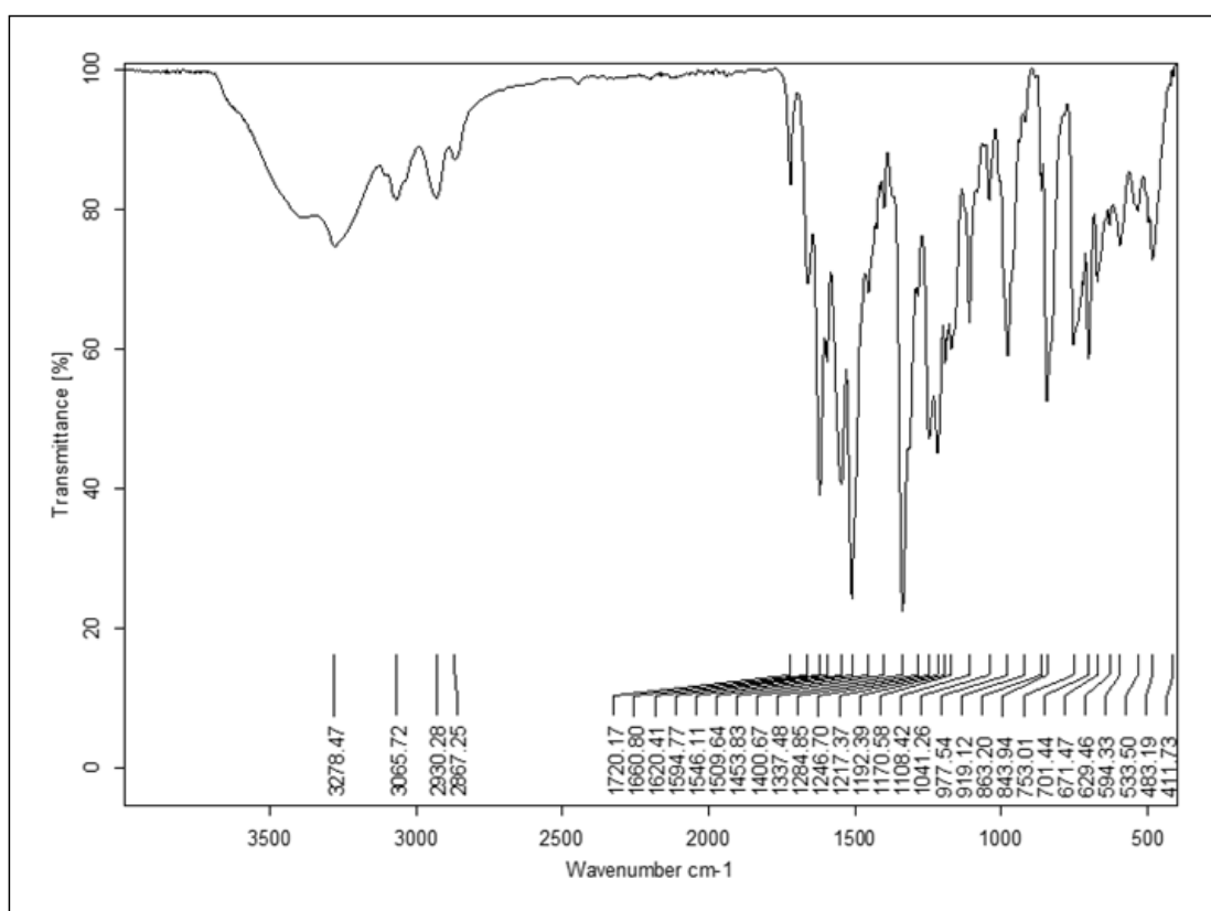
Figure S32. DEPT-135 and IR spectra of ( E )- N -(4-(3-(benzyloxy)-2-methyl-4-oxopyridin-1(4 H )-yl)butyl)-3-(4-nitrophenyl)acrylamide ( 6k ).
