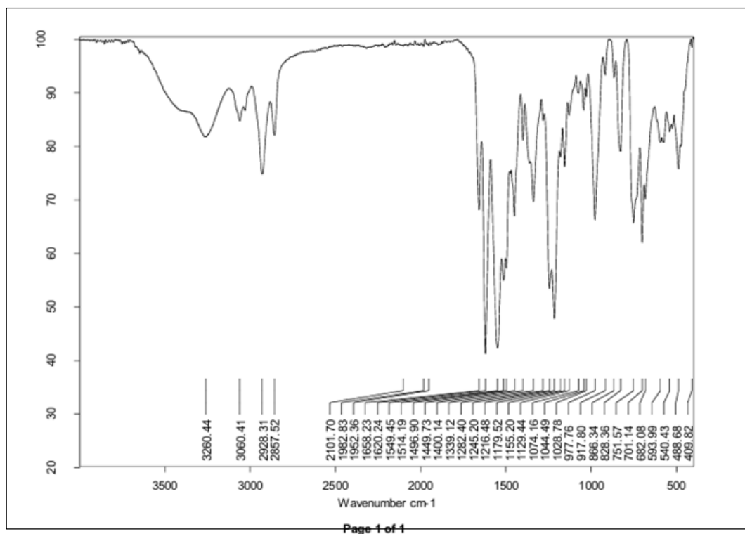
Figure S41. DEPT-135 and IR spectra of N -(6-(3-(benzyloxy)-2-methyl-4-oxopyridin-1(4 H )-yl)-hexyl)cinnamamide ( 6n ).
