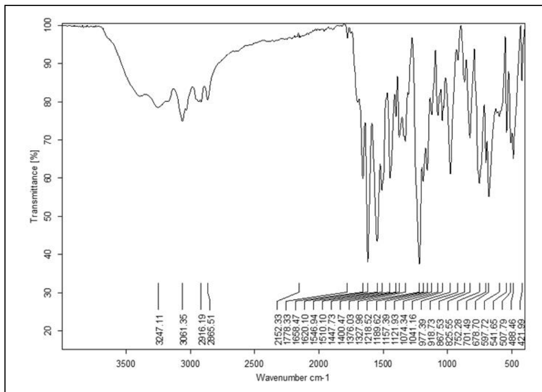
Figure S26. DEPT-135 and IR spectra of N -(4-(3-(benzyloxy)-2-methyl-4-oxopyridin-1(4 H )-yl)-butyl)cinnamamide ( 6i ).
