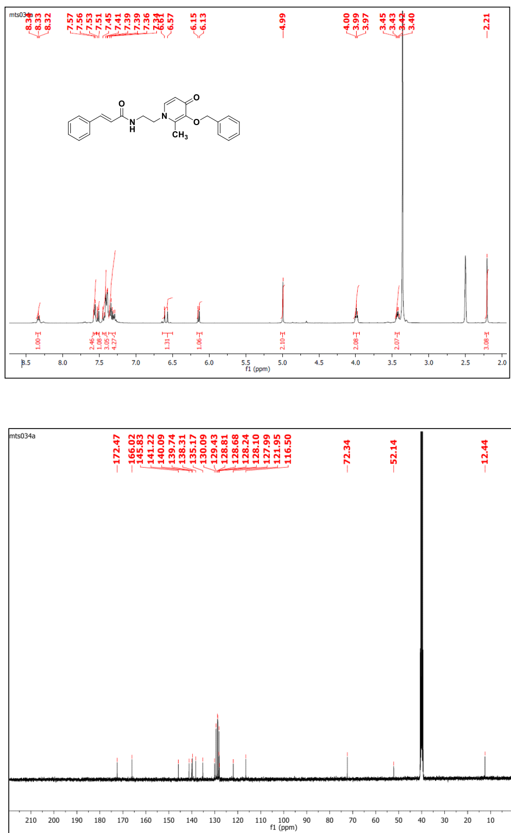
Figure S1. 1 H and 13 C spectra of N-(2-(3-(benzyloxy)-2-methyl-4-oxopyridin-1(4H)-yl)-ethyl)cinnamide ( 6a )
