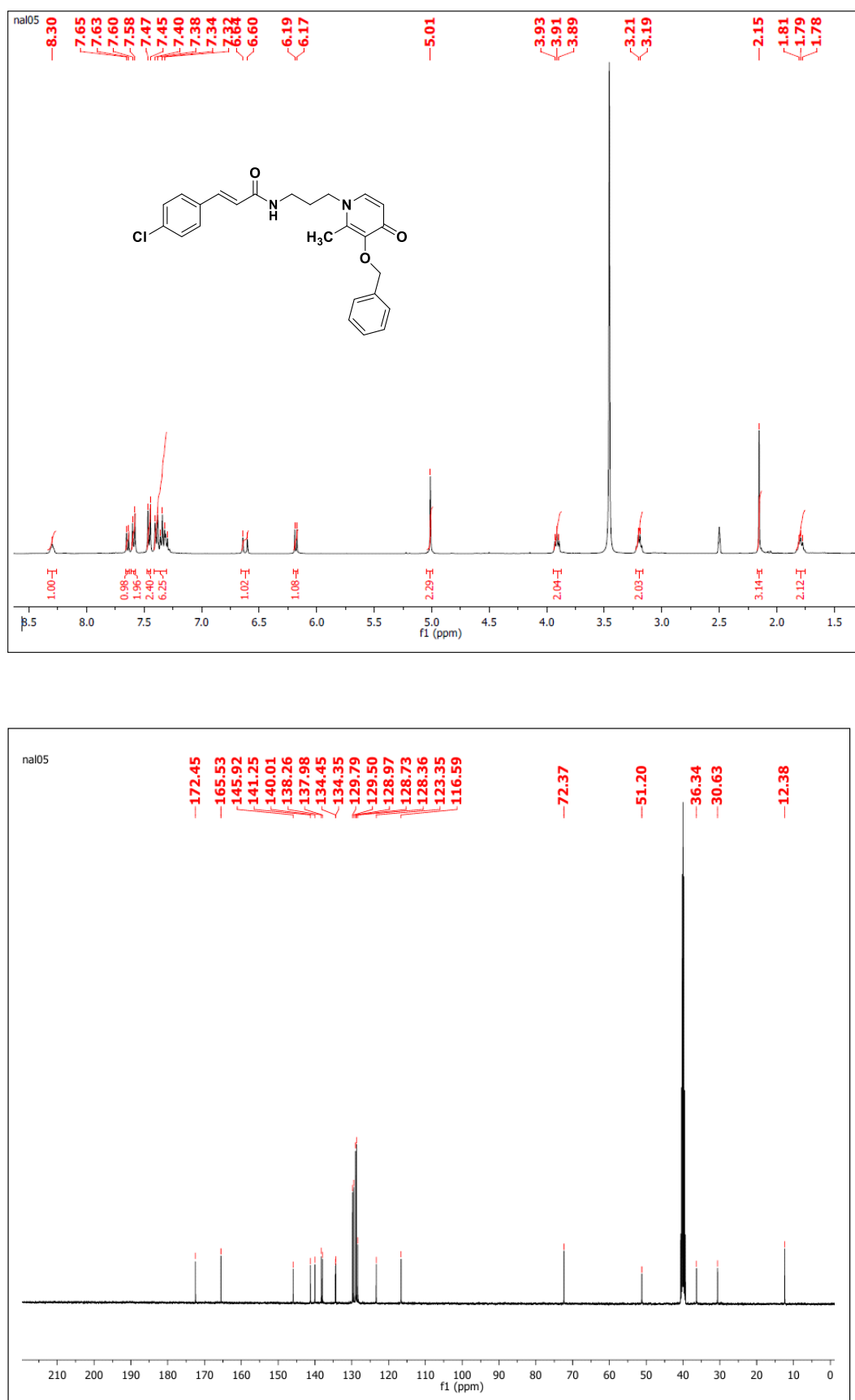
Figure S22. 1 H and 13 C spectra of ( E )- N -(3-(3-(benzyloxy)-2-methyl-4-oxopyridin-1(4 H )-yl)propyl)-3-(4-chlorophenyl)acrylamide ( 6h ).
