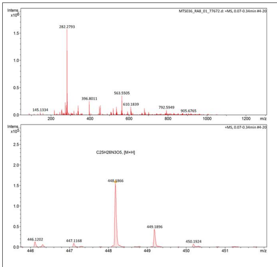
Figure S21. HRMS spectra of (E) - N -(3-(3-(benzyloxy)-2-methyl-4-oxopyridin-1(4H)-yl)propyl)-3-(4-nitrophenyl)acrylamide ( 6g ).
