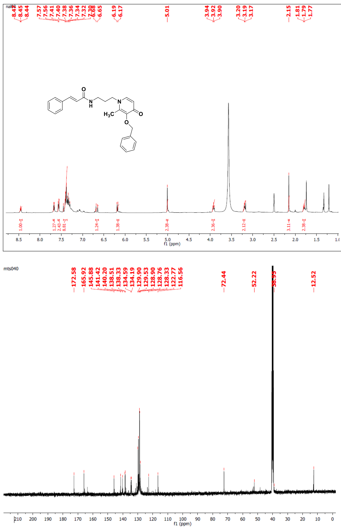
Figure S13. ^1\text{H} and ^{13}\text{C} spectra of N -(3-(3-(benzyloxy)-2-methyl-4-oxopyridin-1(4 H )-yl)propyl)cinnamamide ( 6e ).
