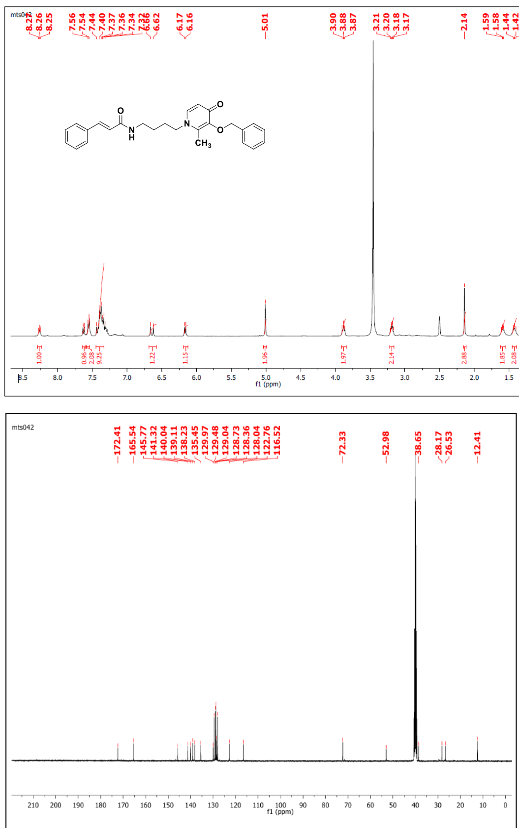
Figure S25. 1 H and 13 C spectra of N -(4-(3-(benzyloxy)-2-methyl-4-oxopyridin-1(4 H )-yl)butyl)cinnamamide ( 6i ).
