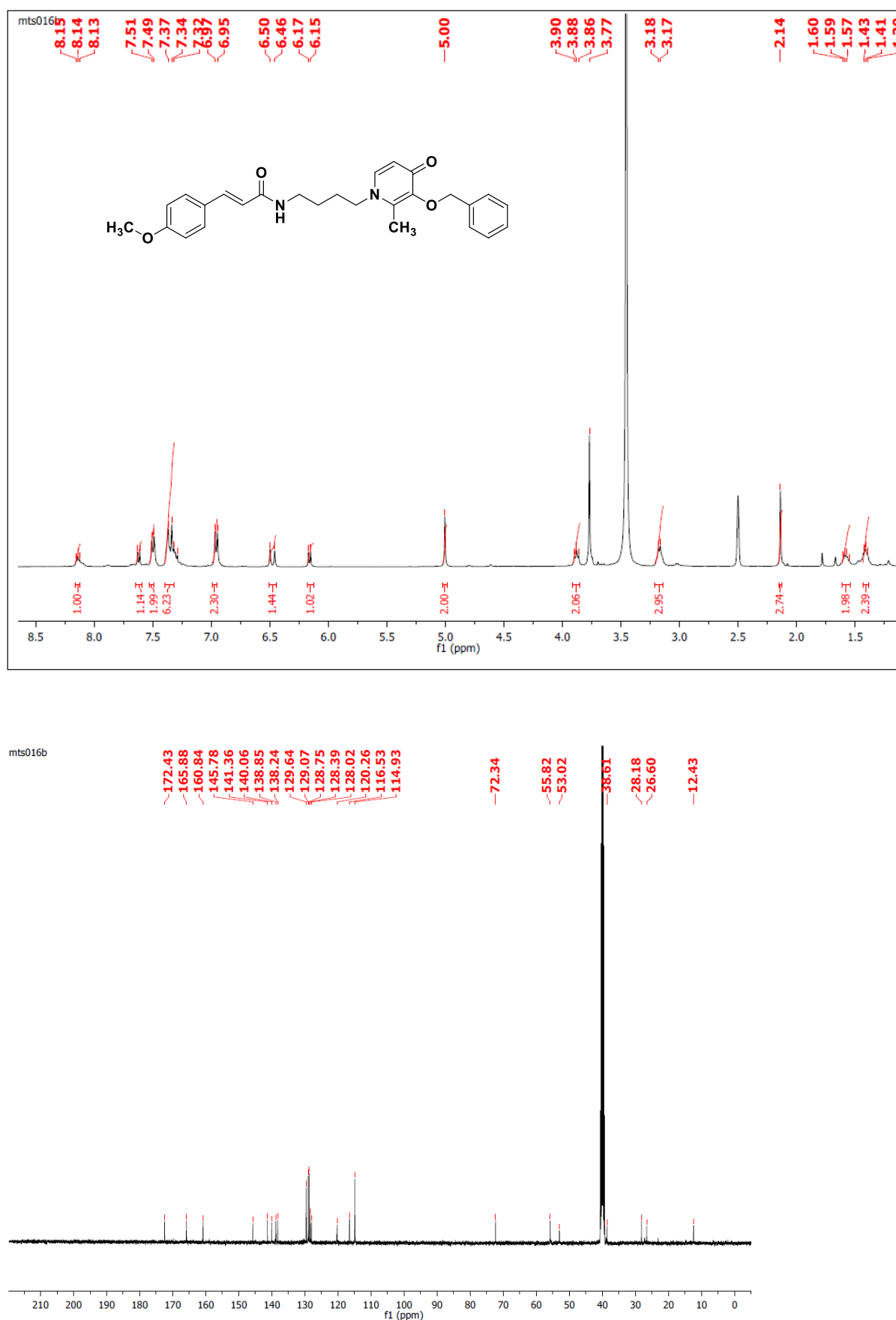
Figure S28. 1 H and 13 C spectra of (E)-N-(4-(3-(benzyloxy)-2-methyl-4-oxopyridin-1(4H)-yl)butyl)-3-(4-methoxyphenyl)acrylamide (6j) .
