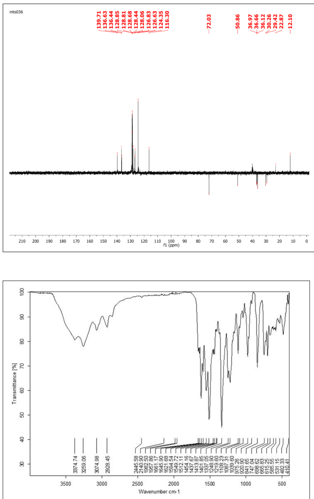
Figure S20. DEPT-135 and IR spectra of ( E )- N -(3-(3-(benzyloxy)-2-methyl-4-oxopyridin-1(4H)-yl)propyl)-3-(4-nitrophenyl)acrylamide ( 6g ).
