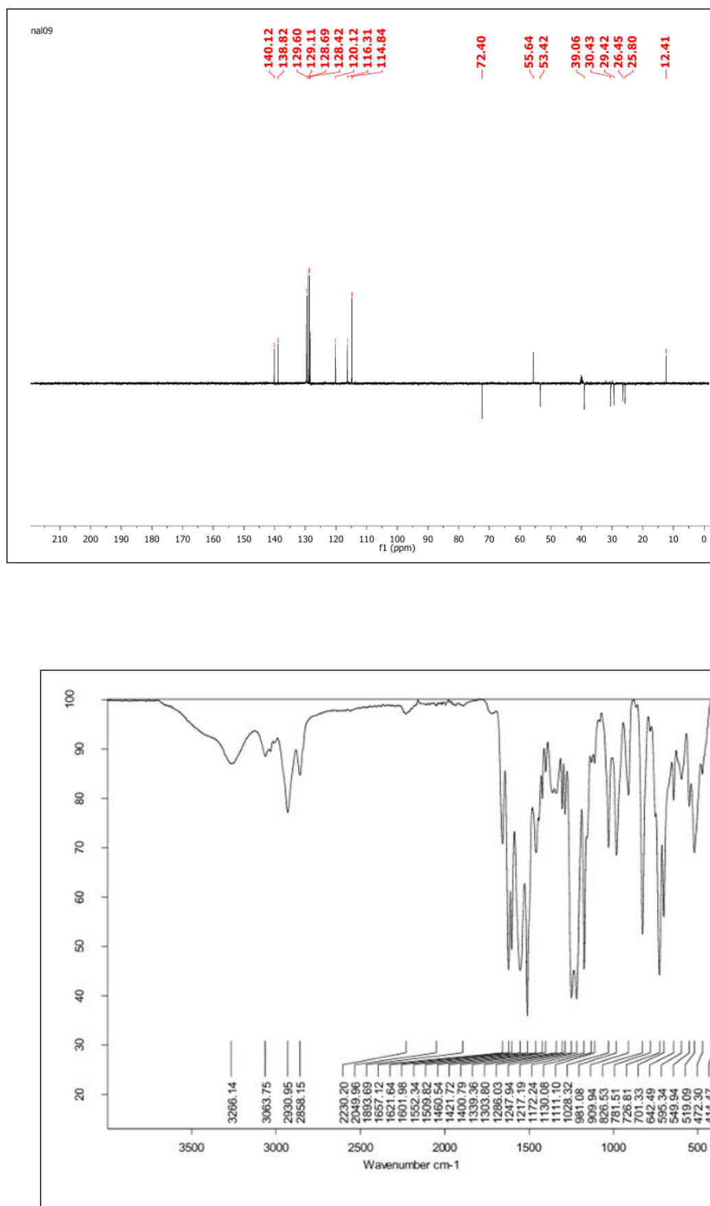
Figure S44. DEPT-135 and IR spectra of ( E )- N -(6-(3-(benzyloxy)-2-methyl-4-oxopyridin-1(4 H )-yl)hexyl)-3-(4-methoxyphenyl)acrylamide ( 6o ).
