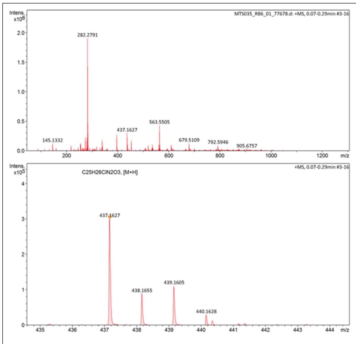
Figure S24. HRMS spectra of ( E )- N -(3-(3-(benzyloxy)-2-methyl-4-oxopyridin-1(4 H )-yl)propyl)-3-(4-chlorophenyl)acrylamide ( 6h ).
