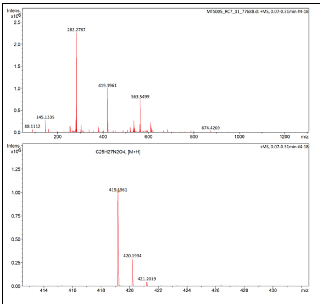
Figure S6. HRMS spectra of (E)-N-(2-(3-(benzyloxy)-2-methyl-4-oxopyridin-1(4H)-yl)ethyl)-3-(4-methoxyphenyl)acrylamide ( 6b ).
