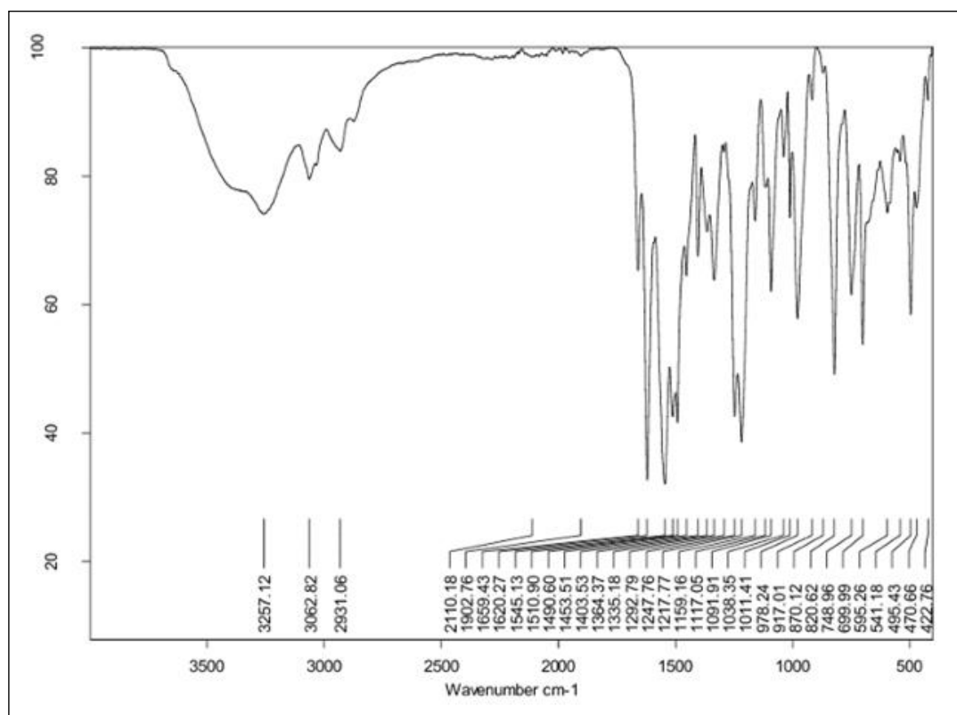
Figure S23. DEPT-135 and IR spectra of ( E )- N -(3-(3-(benzyloxy)-2-methyl-4-oxopyridin-1(4 H )-yl)propyl)-3-(4-chlorophenyl)acrylamide ( 6h ).
