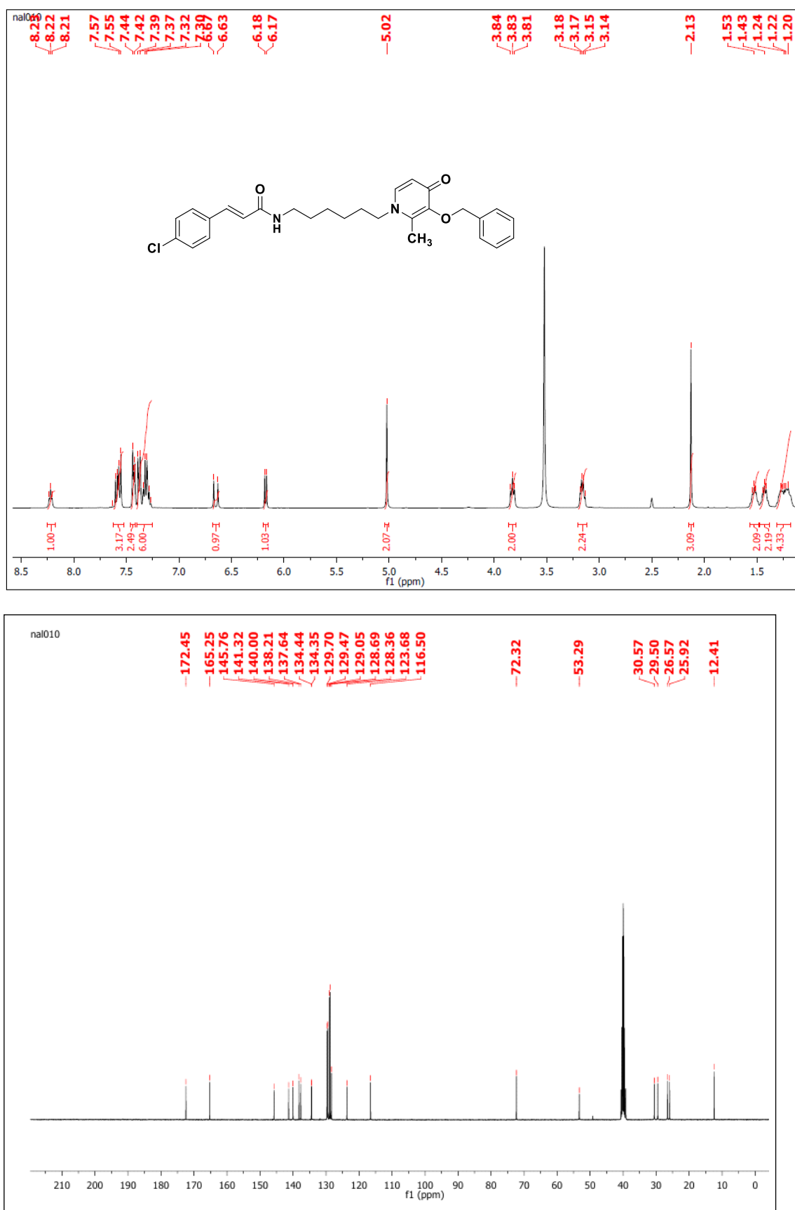
Figure S49. 1 H and 13 C spectra of (E) - N -(6-(3-(benzyloxy)-2-methyl-4-oxopyridin-1(4 H )-yl) hexyl)-3-(4-chlorophenyl)acrylamide ( 6q ).
