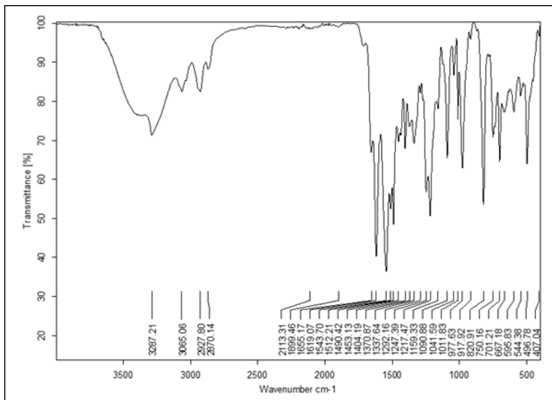
Figure S35. DEPT-135 and IR spectra of ( E )- N -(4-(3-(benzyloxy)-2-methyl-4-oxopyridin-1(4 H )-yl)butyl)-3-(4-chlorophenyl)acrylamide ( 6l ).
