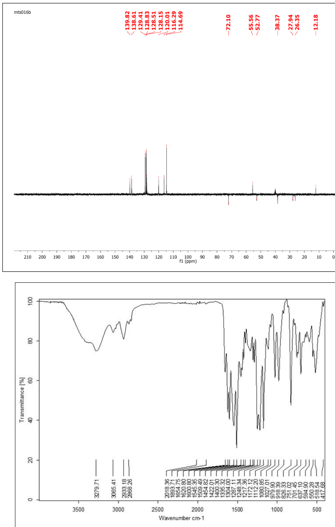
Figure S29. DEPT-135 and IR spectra of ( E )- N -(4-(3-(benzyloxy)-2-methyl-4-oxopyridin-1(4 H )-yl)butyl)-3-(4-methoxyphenyl)acrylamide ( 6j ).
