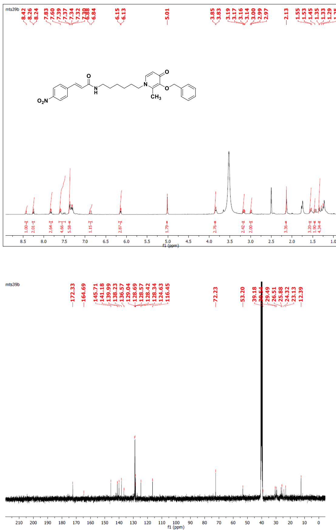
Figure S46. 1 H and 13 C spectra of (E) - N -(6-(3-(benzyloxy)-2-methyl-4-oxopyridin-1(4 H )-yl)hexyl)-3-(4-nitrophenyl)acrylamide ( 6p ).
