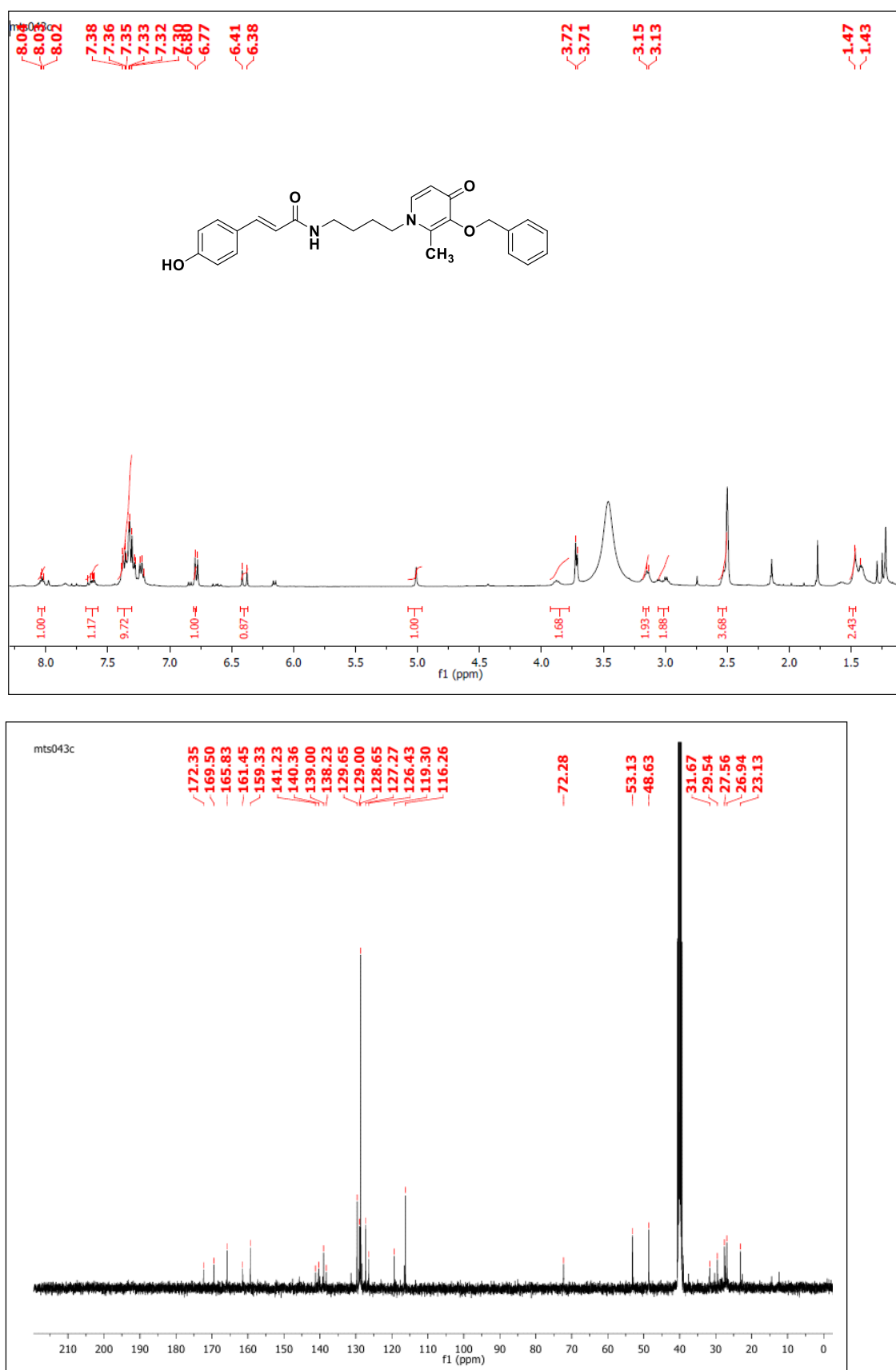
Figure S37. 1 H and 13 C spectra of (E)-N-(4-(3-(benzyloxy)-2-methyl-4-oxopyridin-1(4H)-yl)butyl)-3-(4-hydroxyphenyl)acrylamide (6m) .
