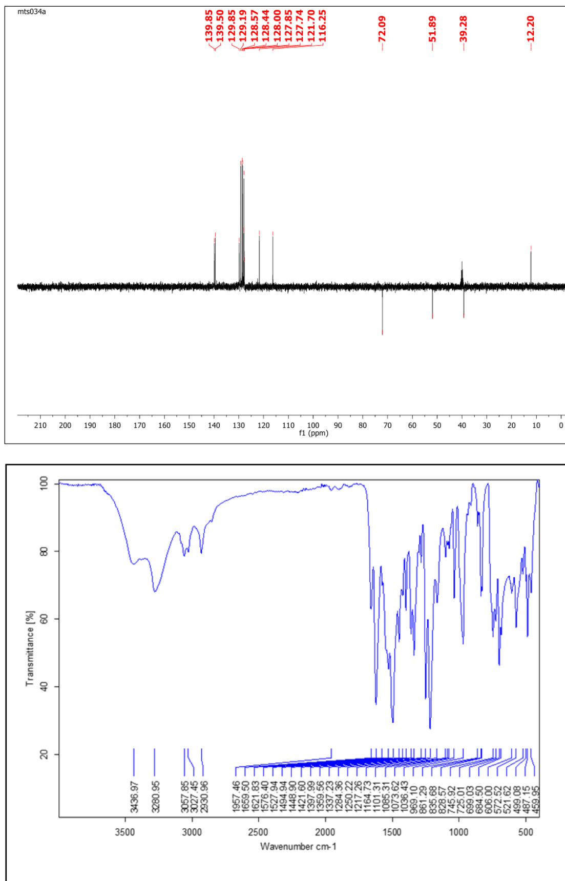
Figure S2. DEPT-135 and IR spectra of N-(2-(3-(benzyloxy)-2-methyl-4-oxopyridin-1(4H)-yl)-ethyl)cinnamamide ( 6a ).
