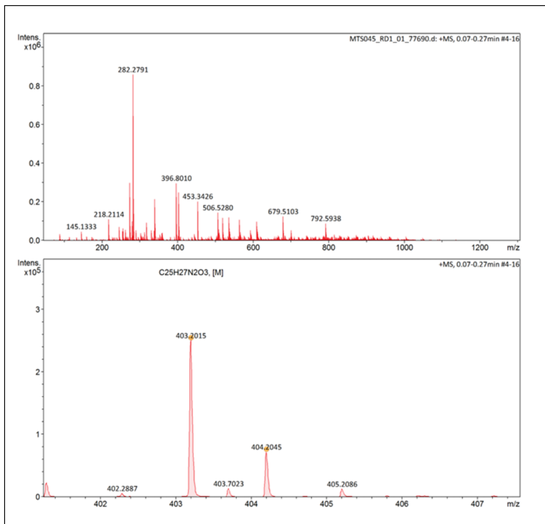
Figure S15. HRMS spectra of N -(3-(3-(benzyloxy)-2-methyl-4-oxopyridin-1(4 H )-yl)propyl)cinnamamide ( 6e ).
