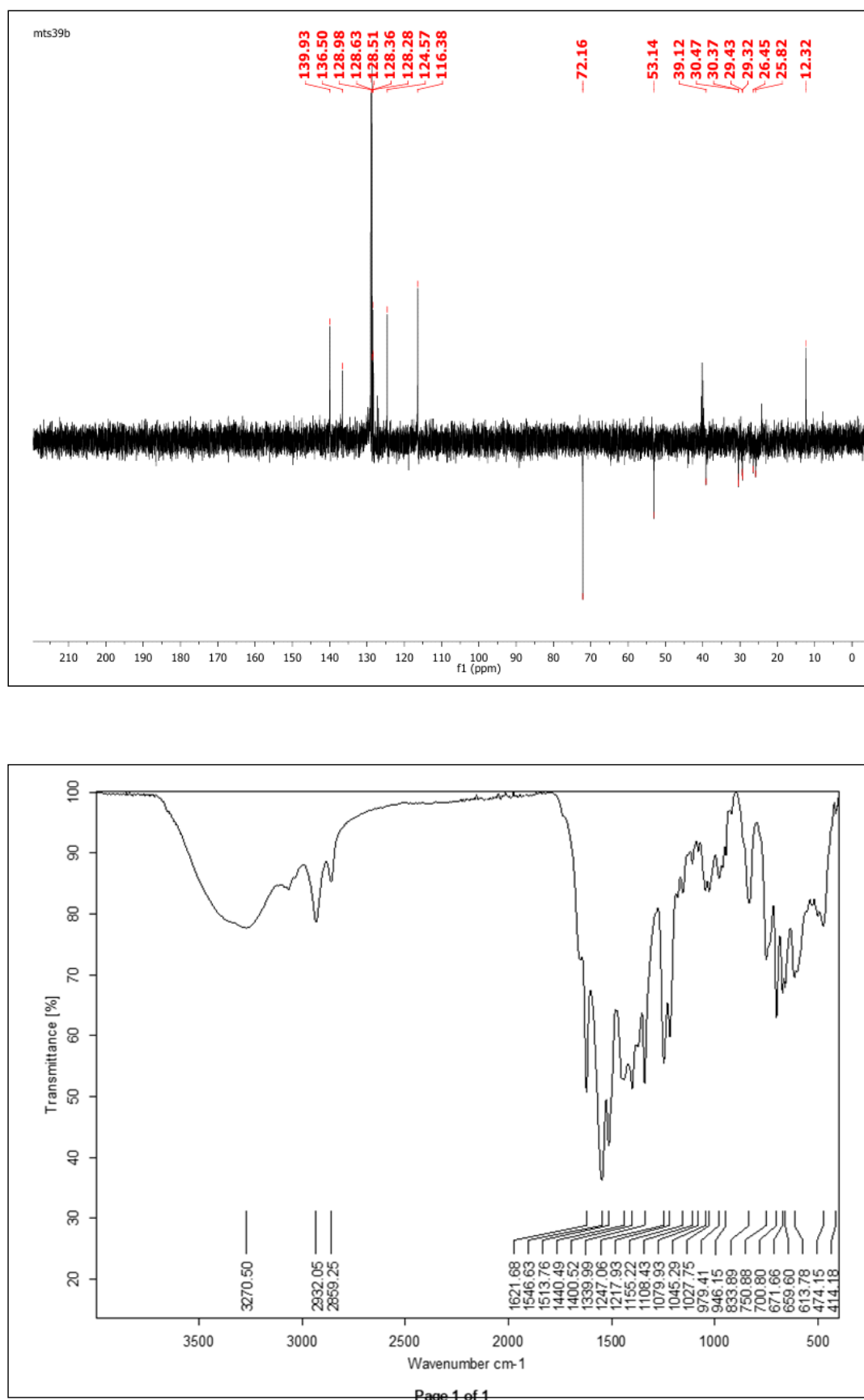
Figure S47. DEPT-135 and IR spectra of ( E )- N -(6-(3-(benzyloxy)-2-methyl-4-oxopyridin-1(4 H )-yl)hexyl)-3-(4-nitrophenyl)acrylamide ( 6p ).
