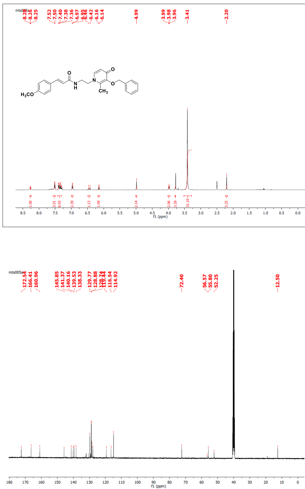
Figure S4. 1 H and 13 C spectra of (E)-N-(2-(3-(benzyloxy)-2-methyl-4-oxopyridin-1(4H)-yl)ethyl)-3-(4-methoxyphenyl)acrylamide ( 6b ).
