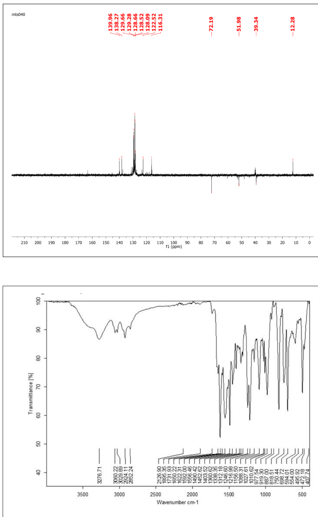
Figure S11. DEPT-135 and IR spectra of ( E )- N -(2-(3-(benzyloxy)-2-methyl-4-oxopyridin-1(4 H )-yl)ethyl)-3-(4-chlorophenyl)acrylamide ( 6d ).
