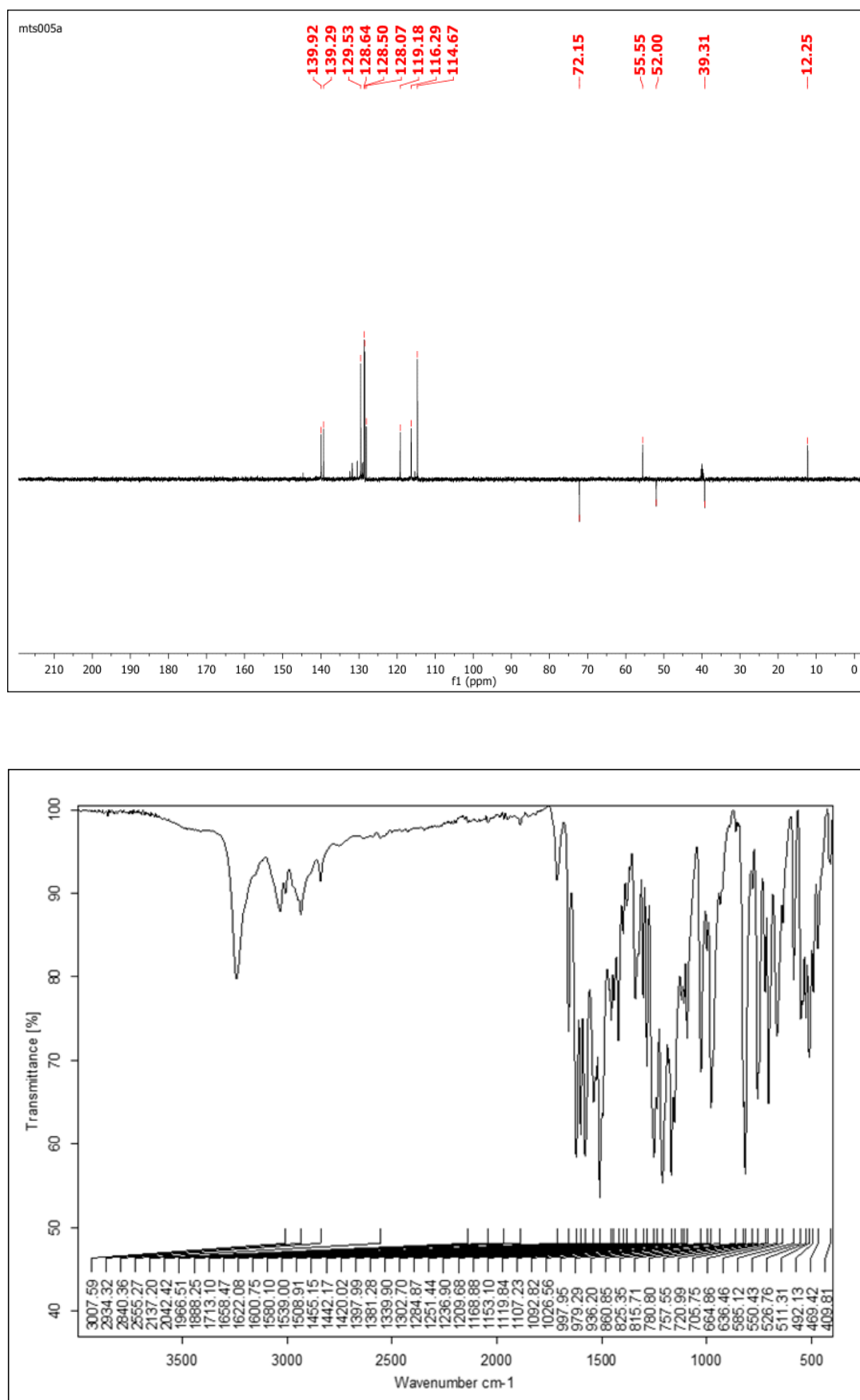
Figure S5. DEPT-135 and IR spectra of (E)-N-(2-(3-(benzyloxy)-2-methyl-4-oxopyridin-1(4H)-yl)ethyl)-3-(4-methoxyphenyl)acrylamide ( 6b ).
