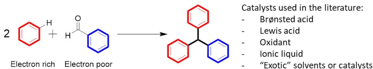
Figure 2. Friedel-Crafts reaction and Baeyer condensation toward triphenylmethane bearing electron-rich arenes.
