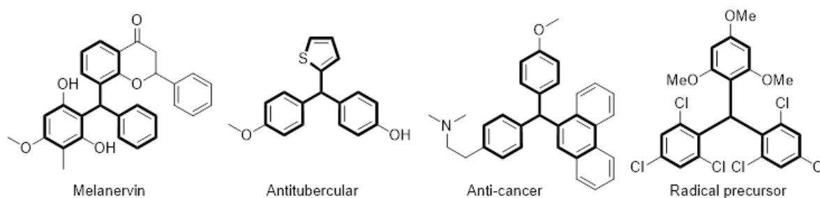
Figure 1. Examples of natural and synthetic biologically active triarylmethanes, and building blocks containing triarylmethyl moieties.
