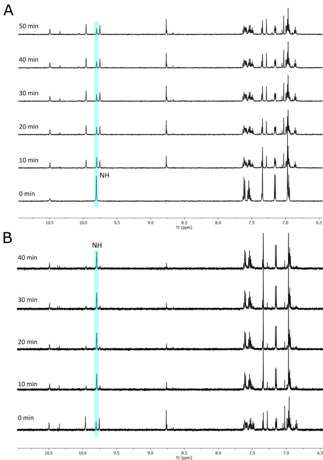
Figure 3. Real-time ^1\text{H} NMR spectroscopic monitoring with in situ irradiation of (A) the forward Z,Z - E,Z isomerization of 5a upon irradiation at \lambda = 520 \text{ nm} and (B) the follow-up backward E,Z - Z,Z isomerization of 5a upon irradiation at \lambda = 625 \text{ nm} ( c = 3 \text{ mM} ) in \text{DMSO-}d_6 . The characteristic signals of the NH groups are highlighted in blue.
