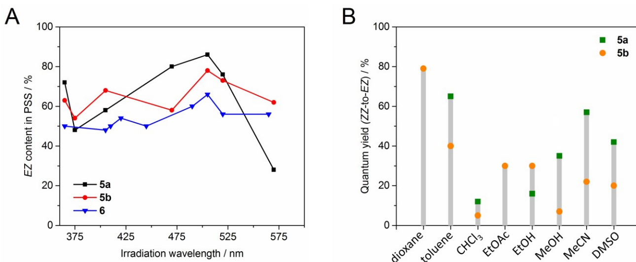
Figure 4. (A) Composition of photostationary states (conversion (%) of starting isomer) of 5a and 5b obtained upon irradiation at different wavelengths in DMSO ( c = 30 \mu M, the data for compound 6 are taken from ref. 15 and plotted on the same graph for better comparison) and (B) dependence of the Z,Z – E,Z photoisomerization quantum yields of 5a and 5b ( \lambda_{\text{ex}} = 505 nm) on the solvent, the solvents are arranged in order of increasing dielectric constant values from left to right, the quantum yields for 5a in dioxane and EtOAc were not determined.
