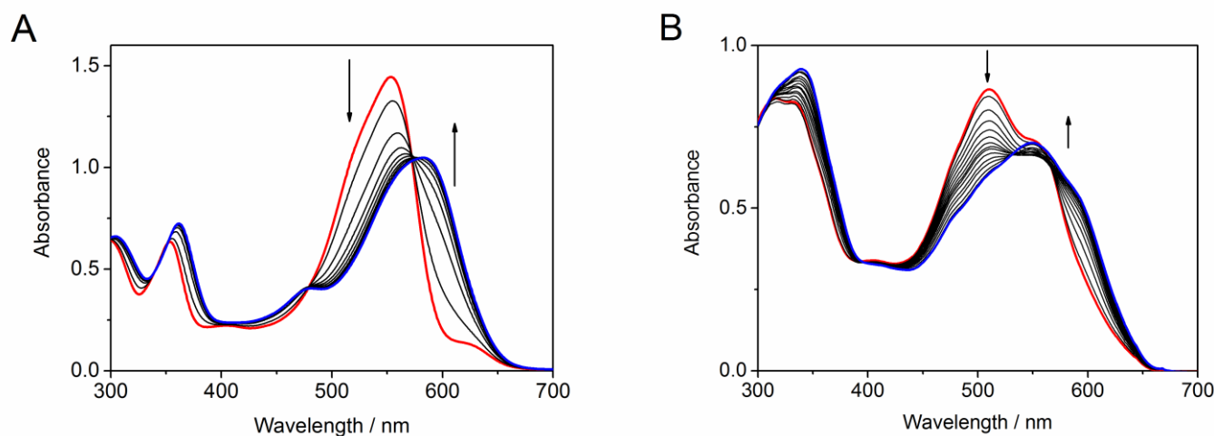
Figure 2. Changes of the absorption of (A) 5a and (B) 5b during irradiation with cyan light ( \lambda_{\text{ex}} = 505 nm), c = 30 \mu\text{M} in DMSO, arrows indicate the development of the absorption bands with increasing irradiation time.
