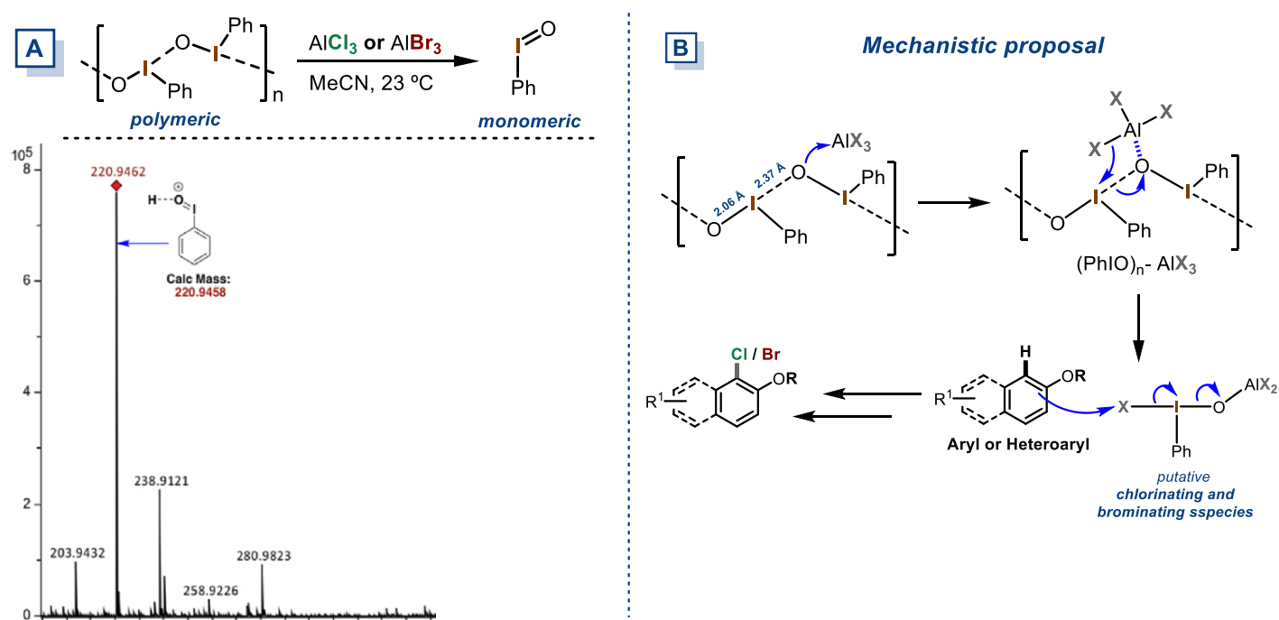
Scheme 7. A) Depolymerization of (\text{PhIO})_n by interaction with \text{AlX}_3 ( \text{X} = \text{Cl}, \text{Br} ) for the HRMS molecular peak identification of PhIO monomer. B) Mechanistic proposal for the chlorination and bromination of naphthols using the system (\text{PhIO})_n\text{-AlX}_3 .
