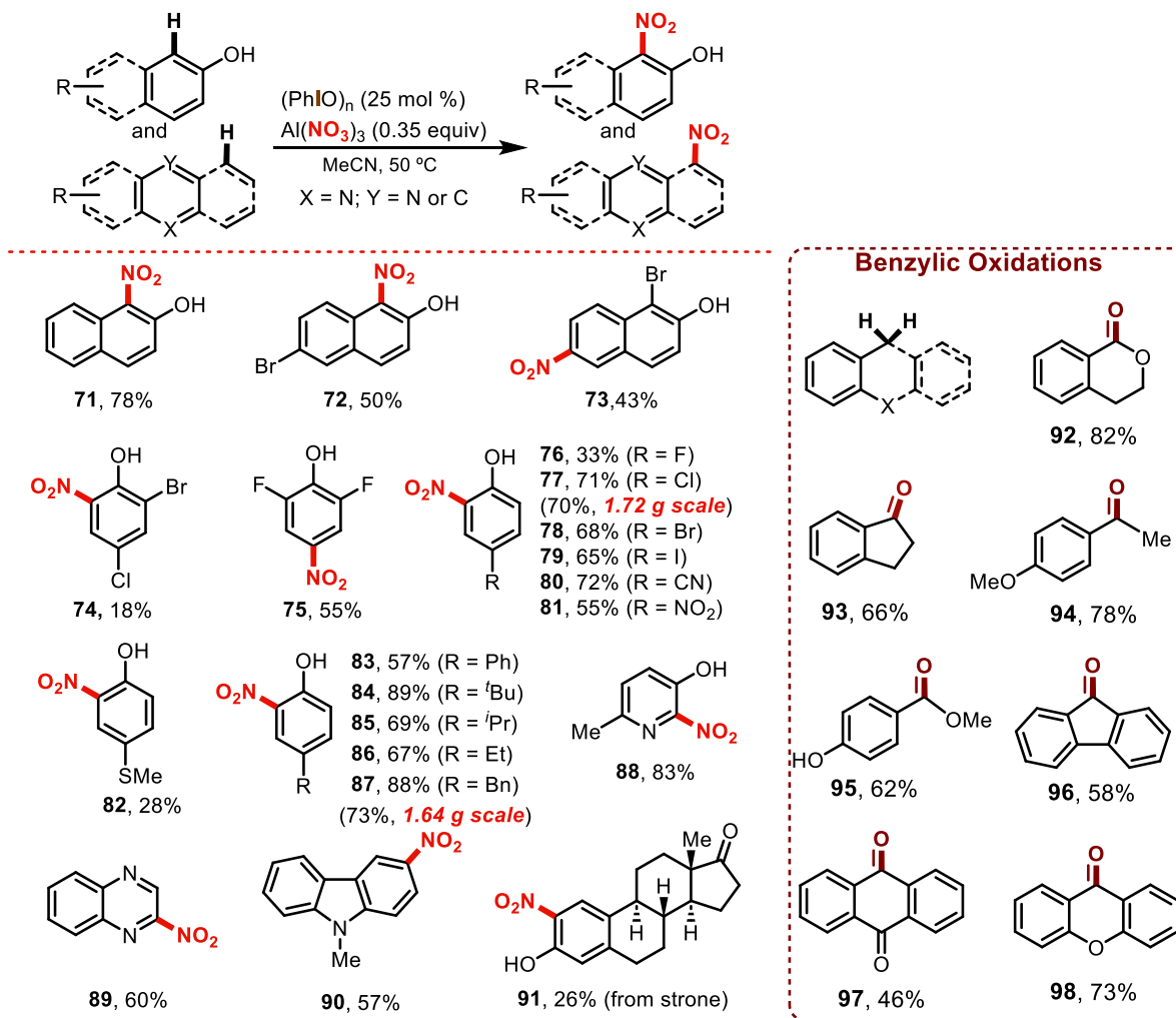
Scheme 17. Scope of the (\text{PhIO})_n\text{-Al}(\text{NO}_3)_3 catalyzed aromatic nitration of N -H free anilines.
