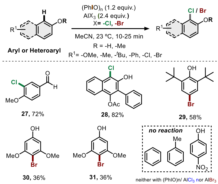
Scheme 6. Representative scope of the (\text{PhIO})_n / \text{-AlCl}_3, \text{-AlBr}_3 mediated oxidative aromatic chlorination and bromination of phenols.
