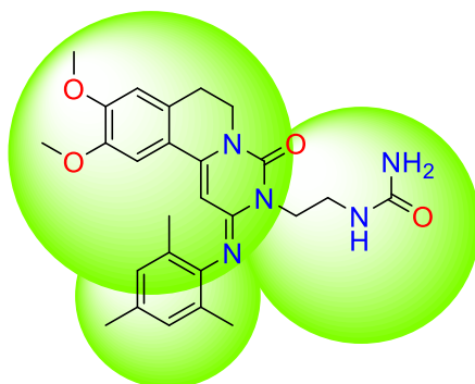
Figure 1. Chemical structure of Ensifentrine.
