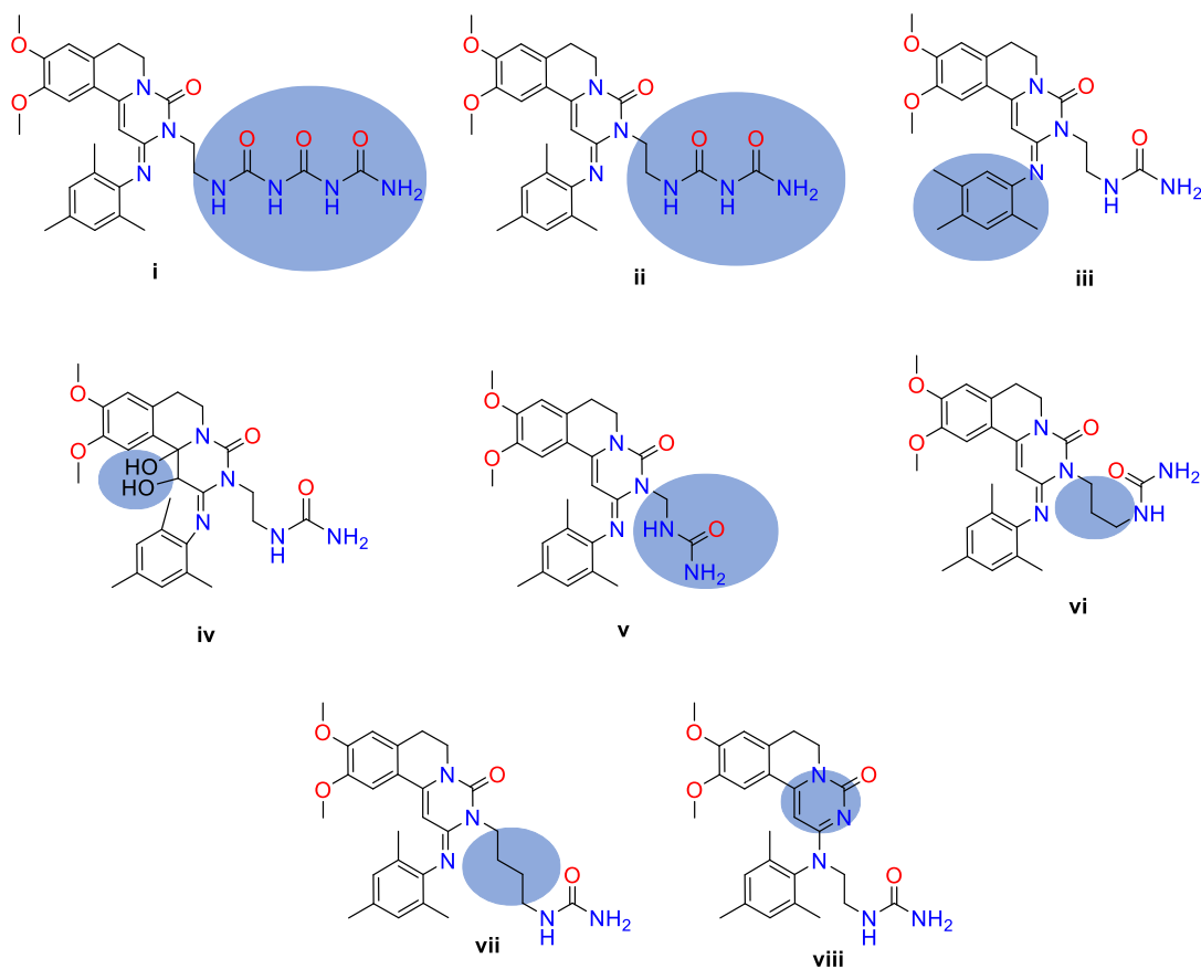
Figure 2. Chemical structures of Ensisfentrine impurities as described in the literature.
