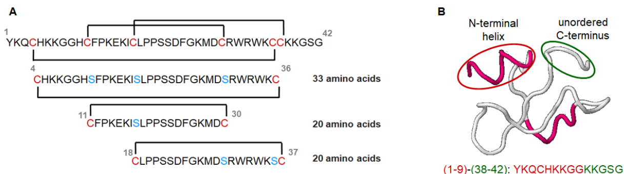
Figure 2: (A) Structural dissection of crotamine showing its peptide fragments linked via disulfide bonds, with non-bridging cysteine residues substituted by serine. (B) 3D structure of crotamine highlighting the close spatial proximity of the N- and C-termini, resulting from its folded conformation.
