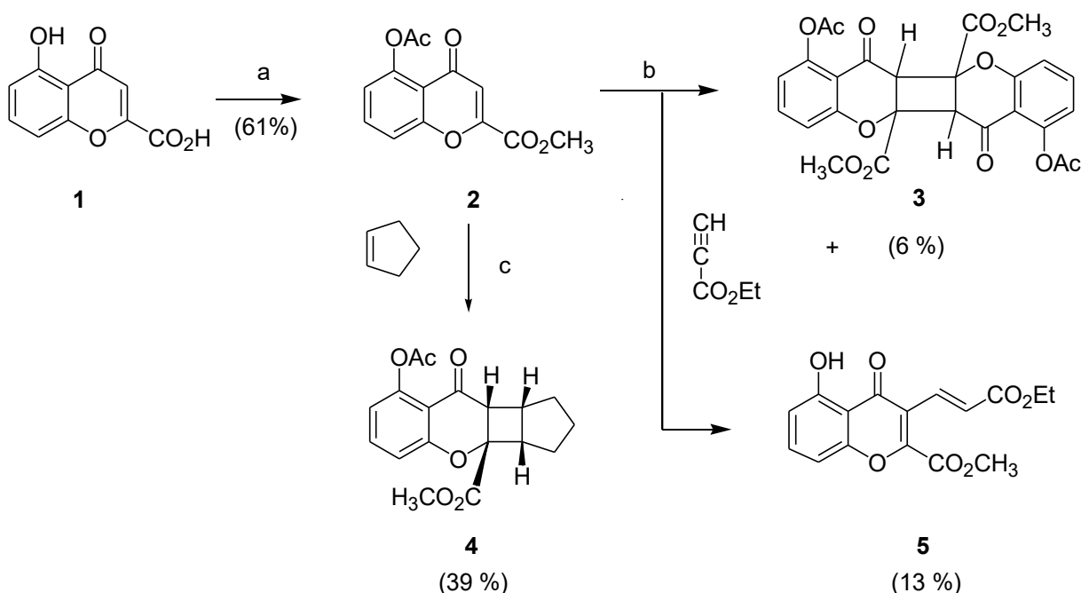
Scheme 1. [2+2] cycloadditions of chromenone 2 to cyclopentene and ethyl propiolate. (a)(i) MeOH, H 2 SO 4 , reflux, 4 h (80%); (ii) Ac 2 O, DMAP, pyridine, CH 2 Cl 2 , rt, 4 h (76%). (b) Rayonet, 313 nm, benzene, rt, 44 h. (c) Rayonet, 313 nm, MeOH, -10 °C, 14 h.
