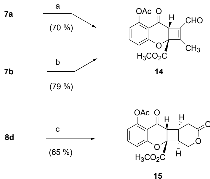
Scheme 6. Reactions of 7a , 7b and 8d for elucidation of their constitutions. (a) HClO 4 [60%, catalytic amount (2 mol %)], MeCN, H 2 O, rt, 30 min (70%). (b) MnO 2 , CH 2 Cl 2 , rt, 4 h (79%). (c) Pd/C (10%), H 2 , MeOH, rt, 1.5 h (65%).
