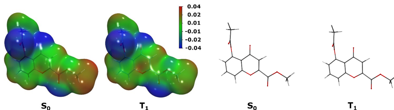
Figure 1. Electrostatic potentials (units in a.u.) mapped on a 0.001 a. u. electron density iso-surface and geometries of S_0 and T_1 of 2 .
