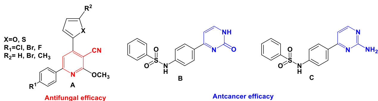
Figure 1. Various biologically active derivatives of pyridine and pyrimidine.
