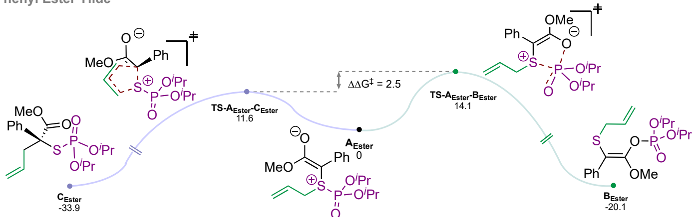
Scheme 4. Free energy reaction profile (kcal/mol) for the S-to-O phosphoryl migration vs Doyle-Kirmse step using the free ylide A Keto and A Ester as model substrate at the M06-2X/6-311++G ** , smd(CH 2 Cl 2 ) level of theory.
