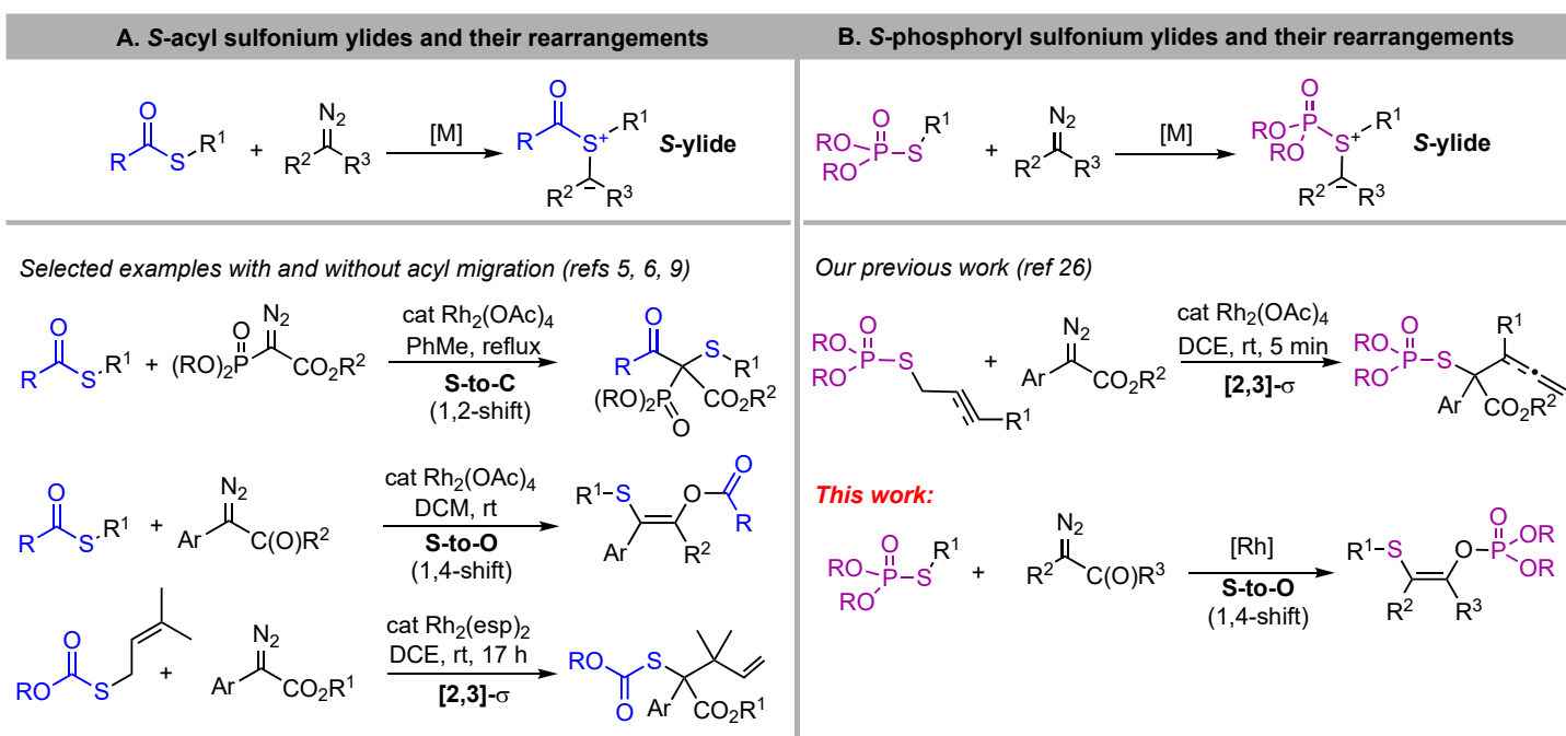
Scheme 1. Rearrangements involving S -acyl and S -phosphoryl sulfonium ylides.
