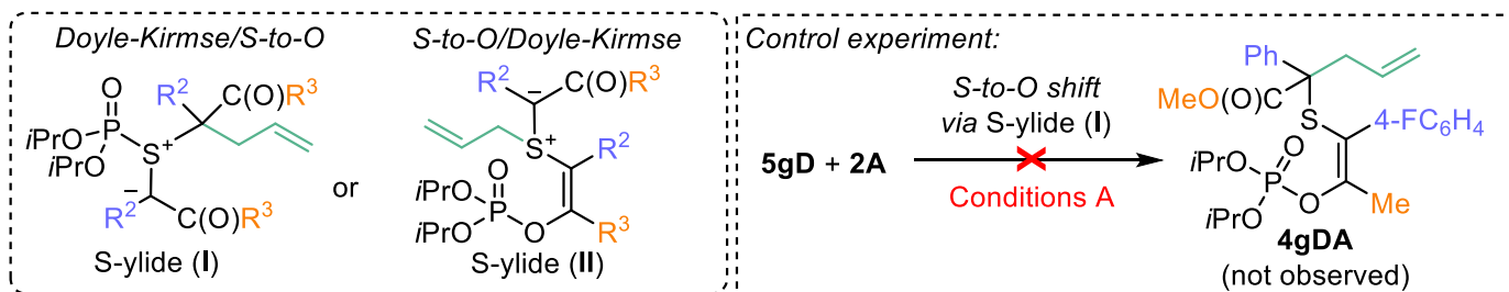
Scheme 3. S-to-O phosphoryl migration vs Doyle-Kirmse rearrangement.
