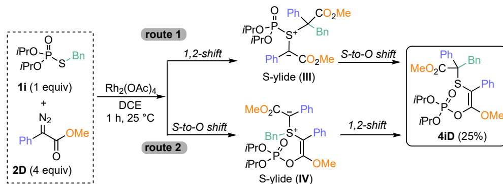
Scheme 5. Possibles routes to 4iD : S -to- O phosphoryl migration vs 1,2-shift (Stevens rearrangement).
