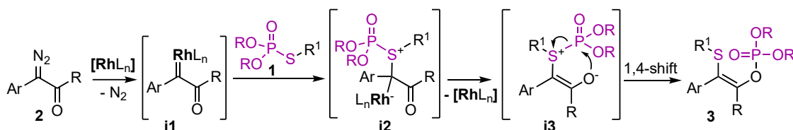
Scheme 2. Proposed mechanism of the reaction with S -to- O phosphoryl transfer.
