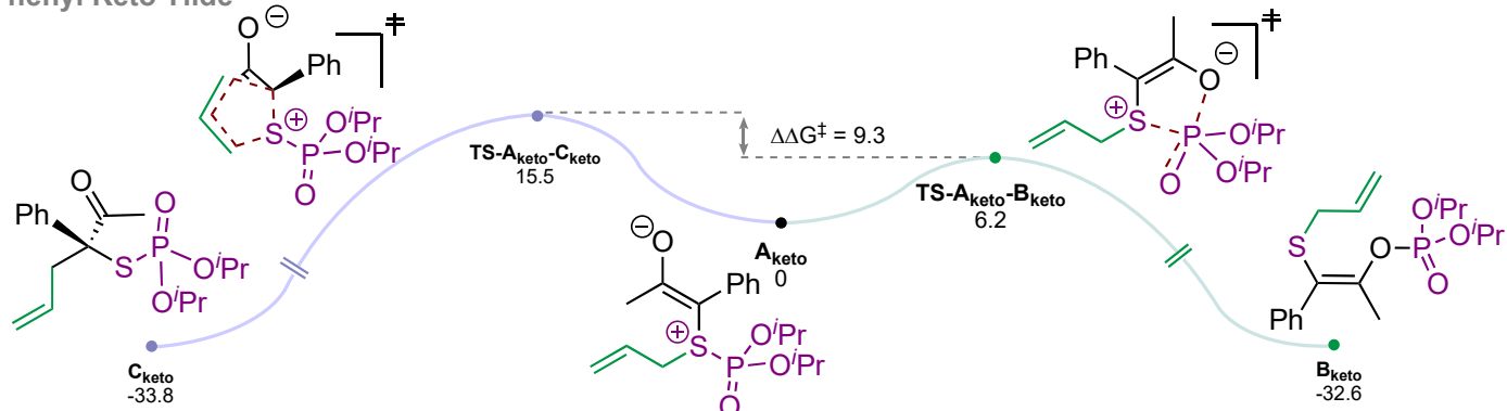
Scheme 3. S-to-O phosphoryl migration vs Doyle-Kirmse rearrangement.
