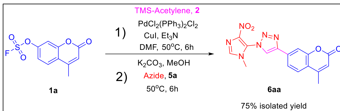
Scheme 3. One-pot synthesis of 6aa .
