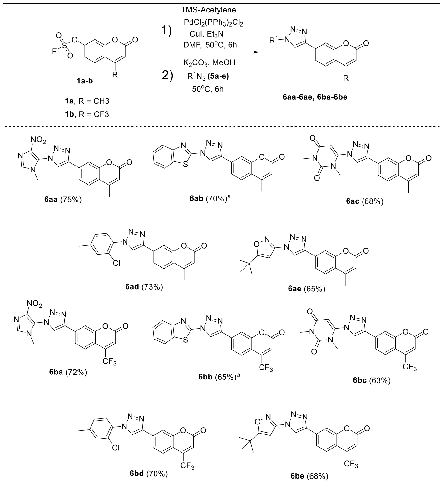
Scheme 4. Substrate scope of the optimized methodology.
