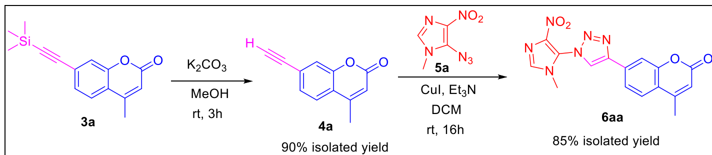
Scheme 2. Deprotection of TMS group and subsequent CuAAC reaction.
