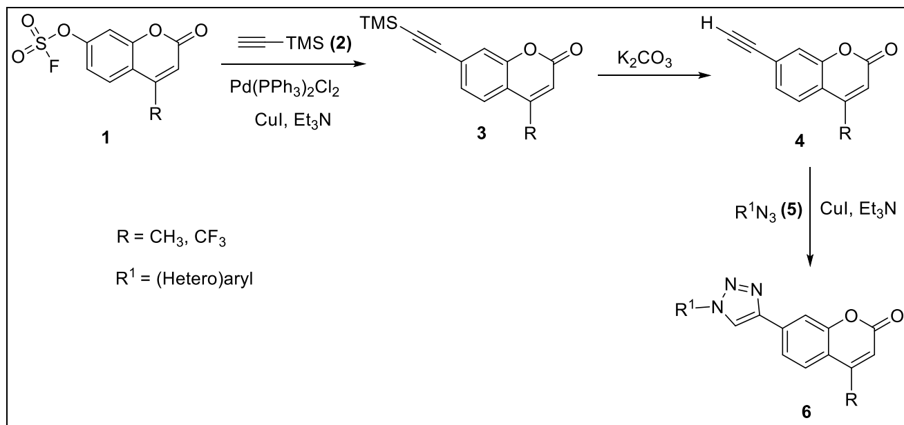
Scheme 1. Initial optimization plan for synthesizing coumarins linked to 1,2,3-triazoles 6 .
