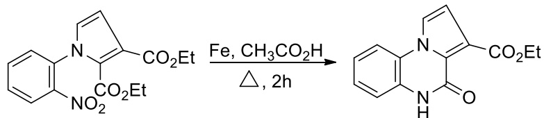
Scheme 1. Previously described synthesis of 4-oxopyrrolo[1,2- a ]quinoxaline-3-carboxylates 21
