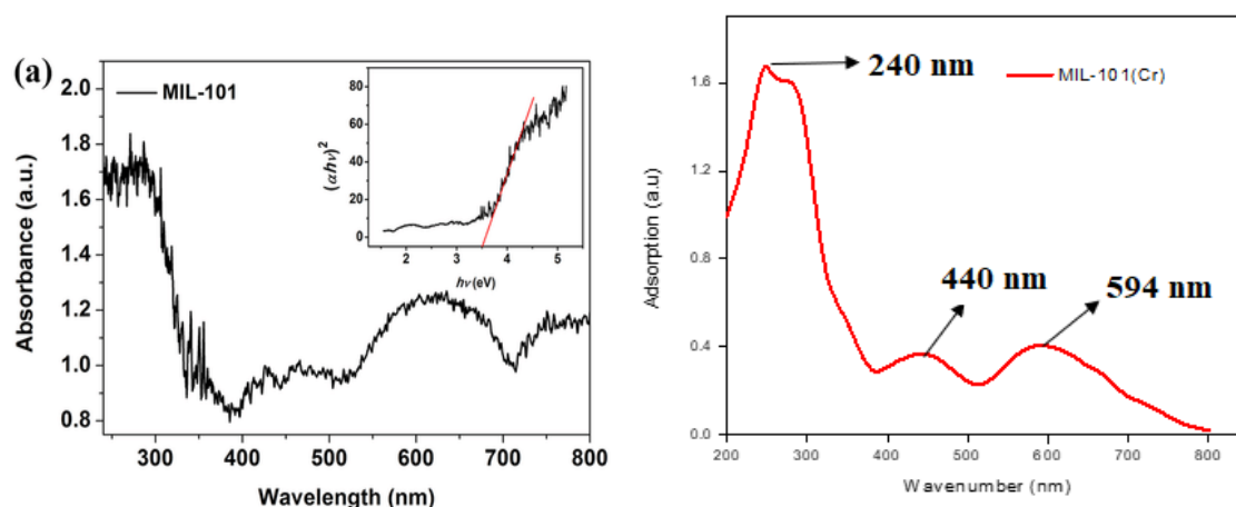
Figure 1. a) UV spectra of reported MIL-101(Cr), b) UV spectra of synthesized MIL-101(Cr).
