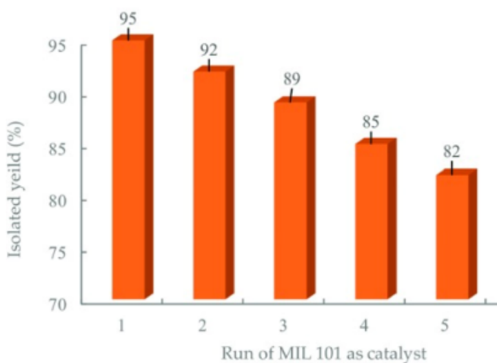
Figure 4. Reusability of the MIL-101(Cr) catalyst for five cycles.
