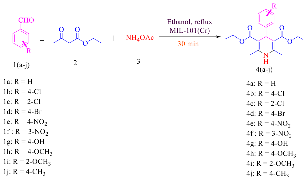
Scheme 1. Synthesis of 1,4-dihydropyridine using MIL-101(Cr) catalyst.
