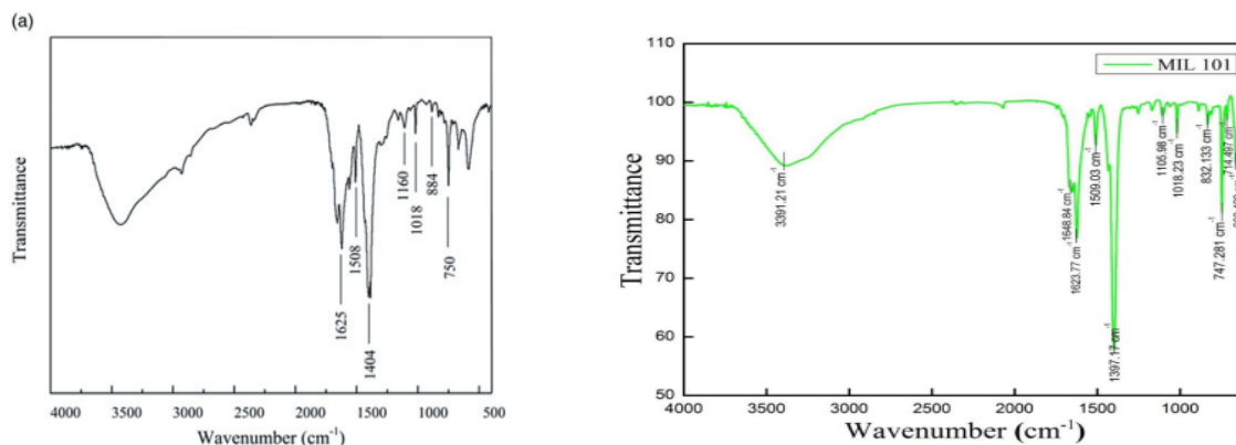
Figure 2. a) FTIR spectra of Reported MIL-101(Cr), b) FTIR spectra of synthesized MIL-101(Cr).
