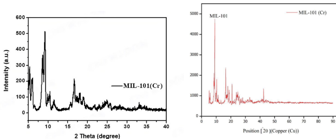
Figure 3. (a) XRD pattern of reported MIL-1(Cr) (b) XRD pattern of synthesized MIL-1(Cr).
