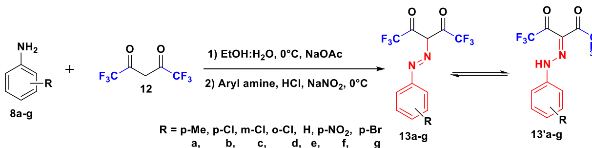
Scheme 1. Synthesis of 1,1,1,5,5,5-hexafluoro-3-arylazopentane-2,4-dione ( 13 ).
