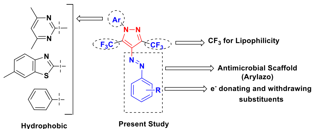
Figure 2. Design of novel pyrazole derivatives.
