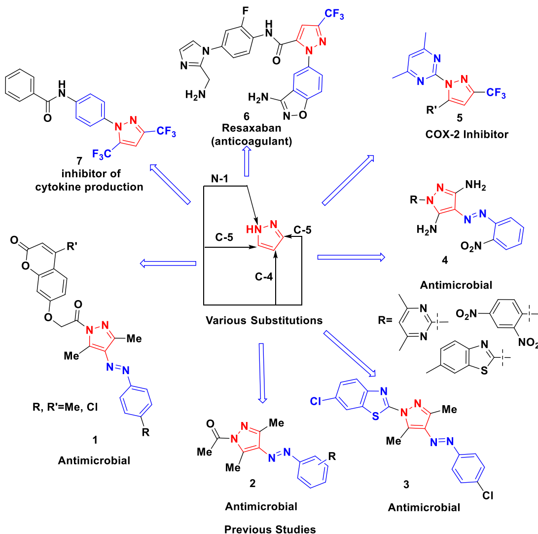
Figure 1. Reported modifications on pyrazole moiety for biological activities.
