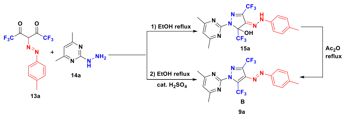
Scheme 2. Synthesis of 4,5-dihydro-1H-pyrazole 15a and pyrazole 9a .
