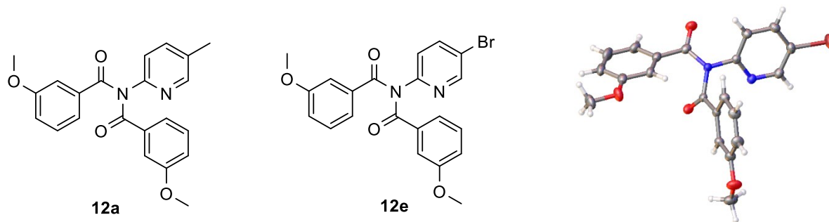
Figure 4. Diacylated compounds 12a and 12e and the ORTEP diagram (50% probability ellipsoids) of major disordered component (85%) of the single-crystal X-ray structure of compound 12e .
