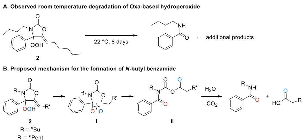
Scheme 1. (A) Room temperature degradation of 2 and (B) the proposed mechanism for this degradation.
