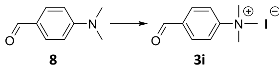
Scheme 3 Synthesis of 4-formyl- N,N,N -trimethylanilinium iodide (3i).
