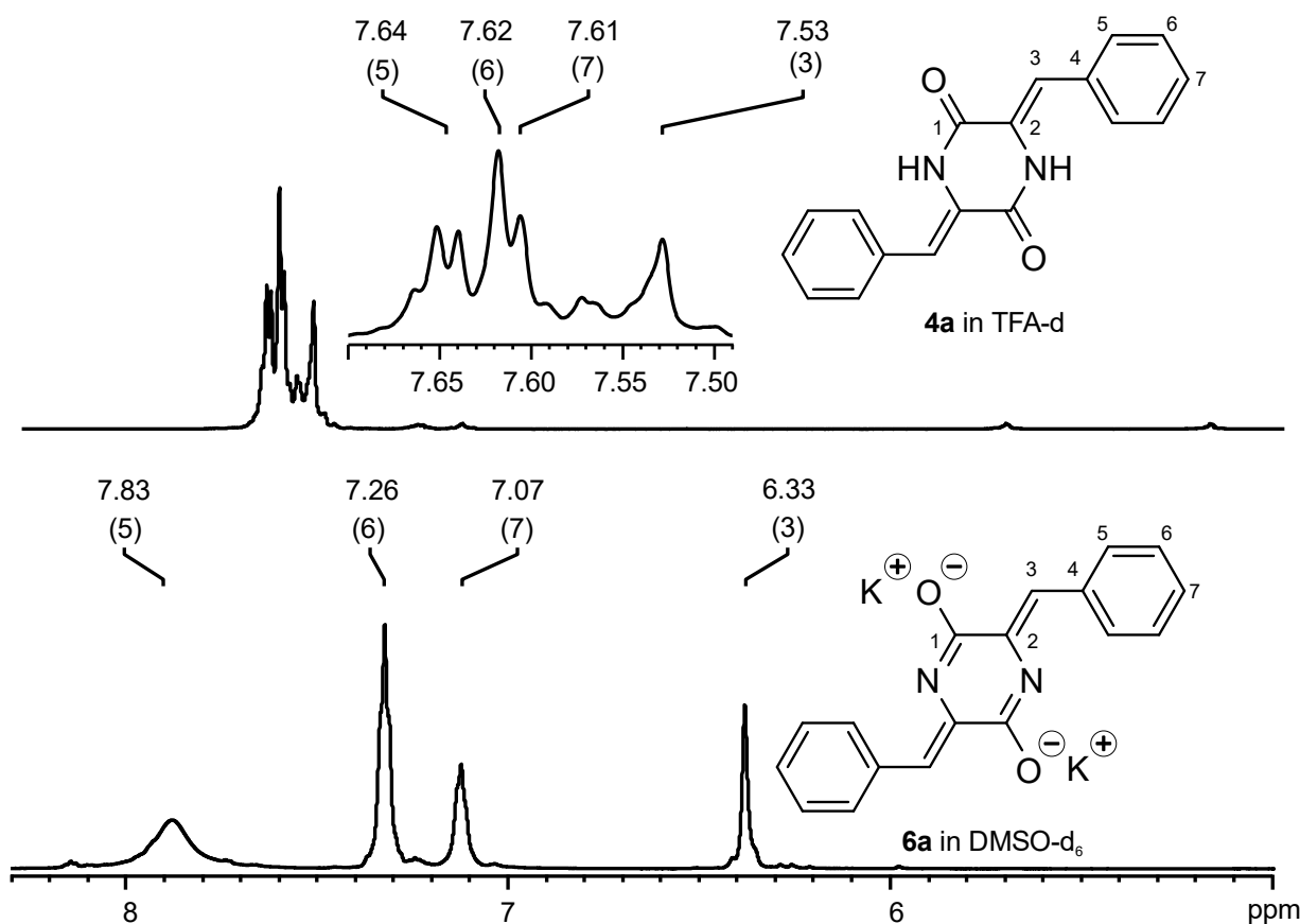
Figure 5. a. Overlaid FTIR of 4a and 6a , clearly illustrate the disappearance of the amide carbonyl stretch to the and formation of imidate ketimine stretch. b. Overlaid ^1\text{H} NMR of 4a in TFA- d and 6a in DMSO- d_6 .
