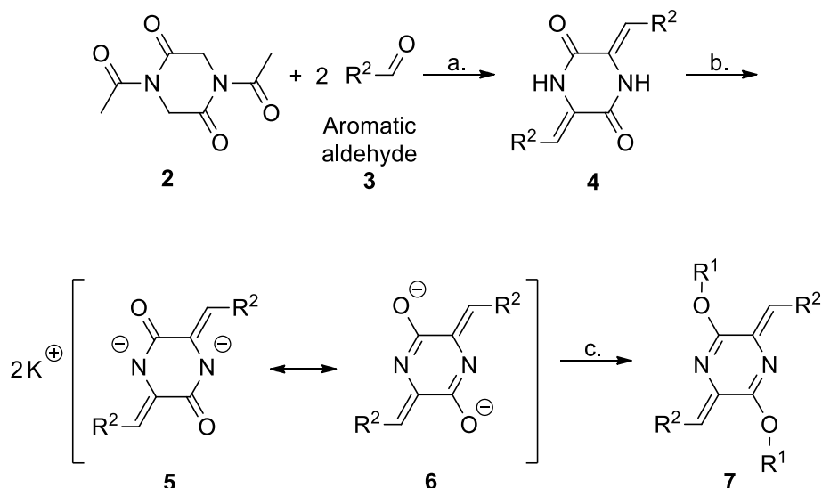
Scheme 1. Synthesis route of p -azaquinodimethanes, 7 , from 1,4-diacetylpiperazine-2,5-dione, 2 , published by Liu, et al. 24 a. TEA, DMF, N 2 , 120°C, overnight. b. K 2 CO 3 , DMF. c. bromoalkane, N 2 , 100°C, 2 h.
