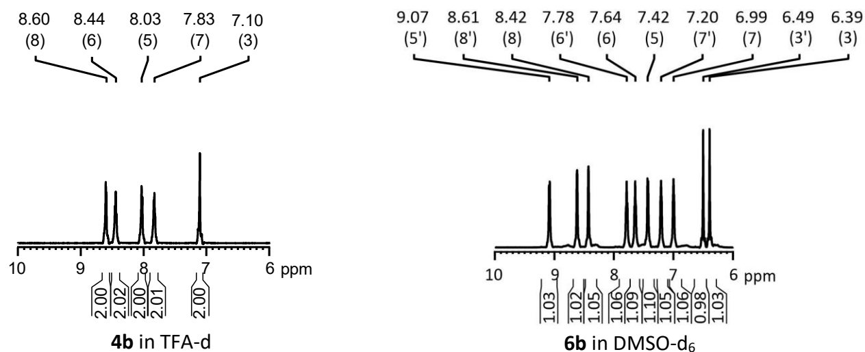
Figure 6 ^1\text{H} NMR of 4b in TFA- d and 6b in DMSO- d_6 ,
