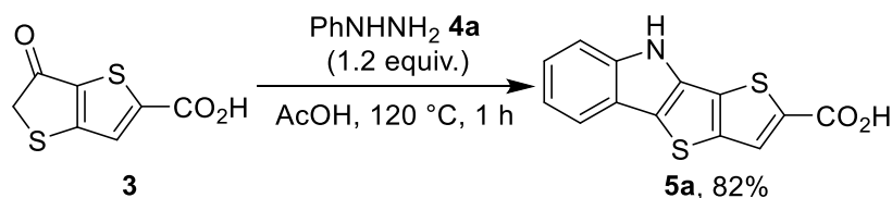
Scheme 4. The synthesis of TTI-2-carboxylic acid 5a .
