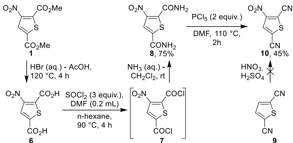
Scheme 5. The synthesis of 3-nitrothiophene-2,5-dicarbonitrile ( 10 ).
