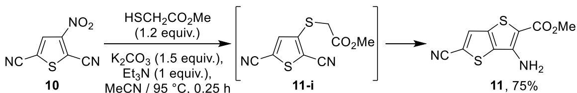
Scheme 6. The synthesis of amino-substituted thieno[3,2- b ]thiophene derivative 11 .
