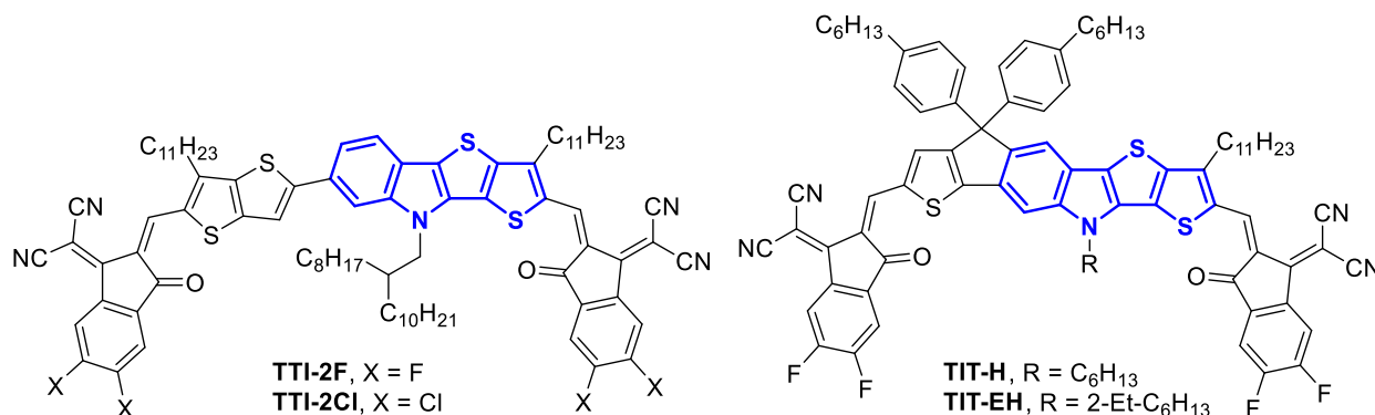
Figure 2. TTI-based non-fullerene acceptor materials.
