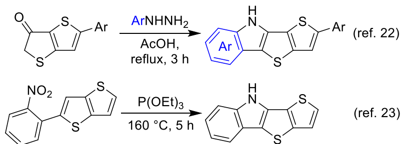
Scheme 1. The known methods for the construction of TTI molecules.
