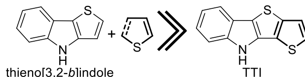
Figure 1. The structure of thieno[3,2- b ]indole and thieno[2',3':4,5]thieno[3,2- b ]indole.
