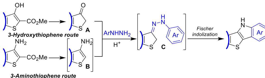
Scheme 2. Fischer indolization based routes to thieno[3,2- b ]indole framework.
