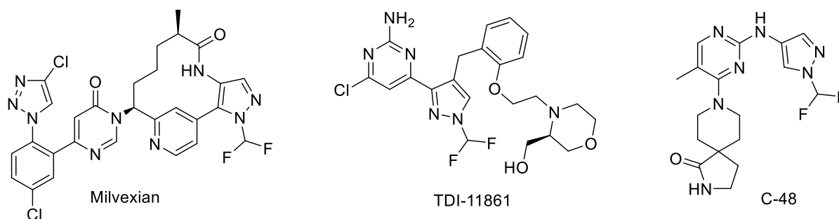
Figure 1. Difluoromethylated pyrazole derivatives.
