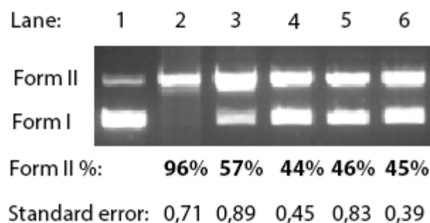
Figure 7. pDNA photocleavage with UV-A irradiation (365nm) for 1h. From left to right: control DNA, neat, irradiated (lane 1); lanes 2-6: DNA solution at 500μM with esters 9a , 5a , 5c , 5d and 5b , respectively.
