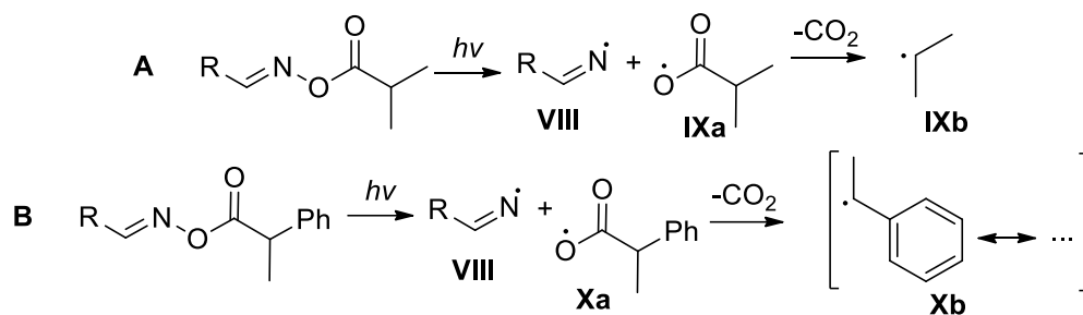
Figure 3. The isobutanoyl and the 2-phenylpropanoyl groups.
