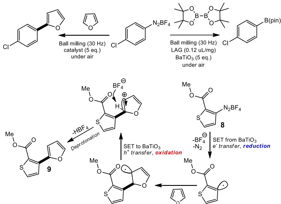
Scheme 4. General reaction of the mechanochemical arylation and borylation reactions. Gram-scale mechanochemical arylation of an aryl diazonium salt yielding a heterobiaryl using \text{BaTiO}_3 and ball milling.
