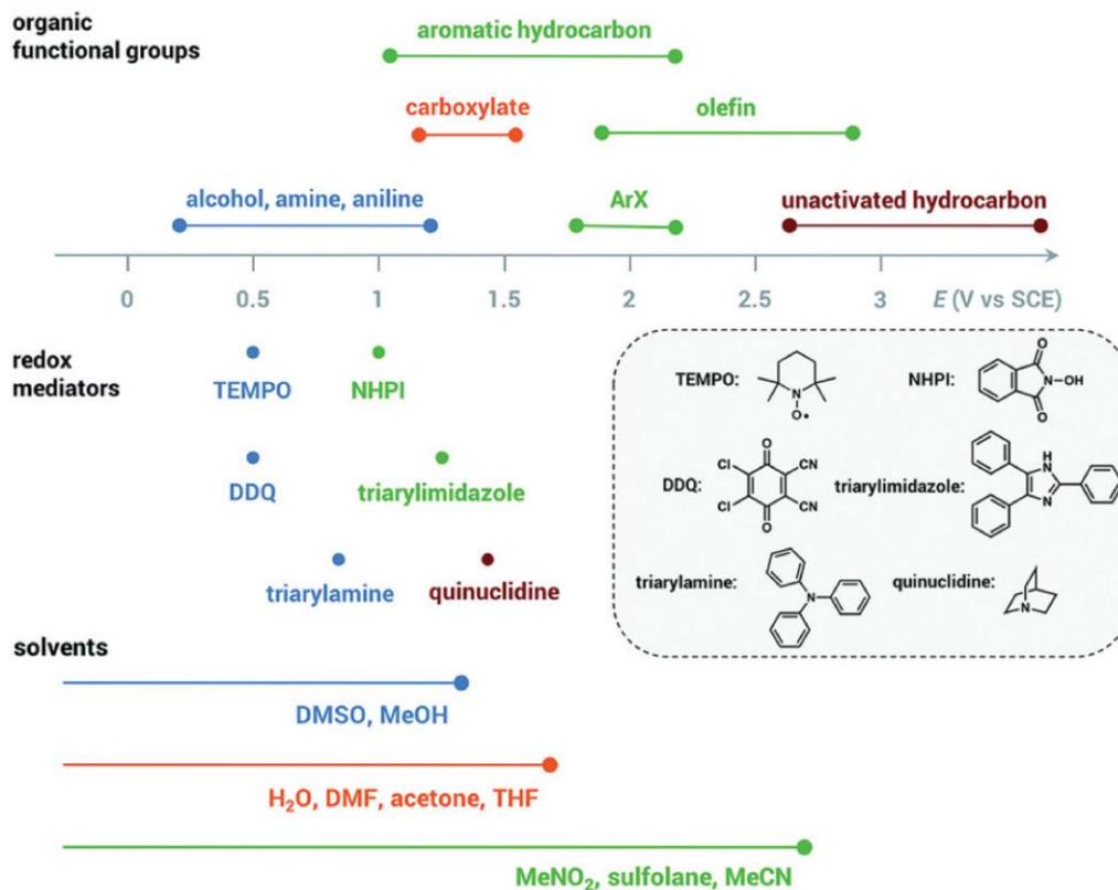
Figure 4. The oxidation potentials of some organic functional groups, redox mediators, and solvents. Reproduced from Ref. 56 with permission. Copyright 2020 Royal Society of Chemistry.
