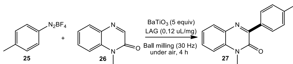
Scheme 11. General reaction of the synthesis of 2-arylquinoxalines via aryldiazonium salts.
