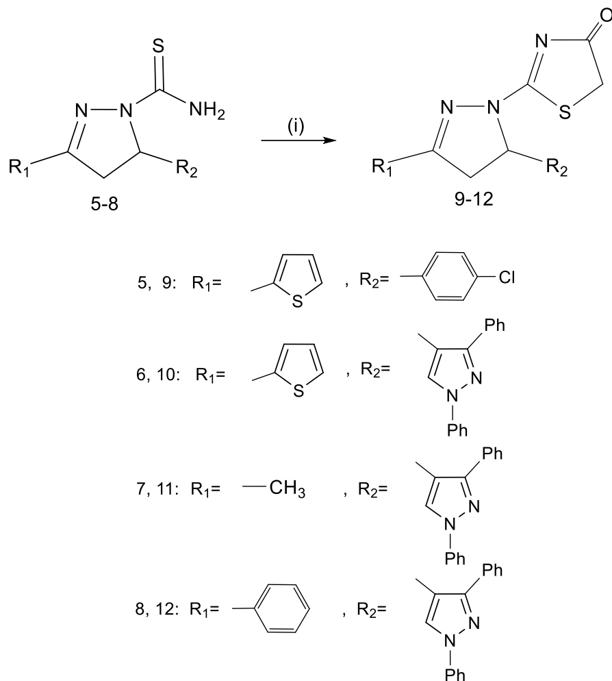
Scheme 2. The synthesis of 1,3-thiazol-4(5H)-one ( 9-12 ): (i) \text{ClCH}_2\text{COOH} , AcOH, AcONa, 8 h.
