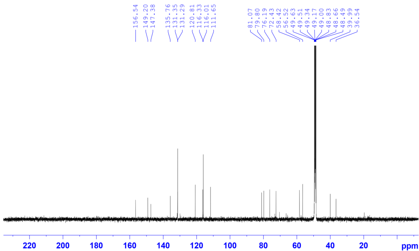
Figure S9. ^{13}\text{C} NMR spectrum of compound 2 (in \text{CD}_3\text{OD} )
