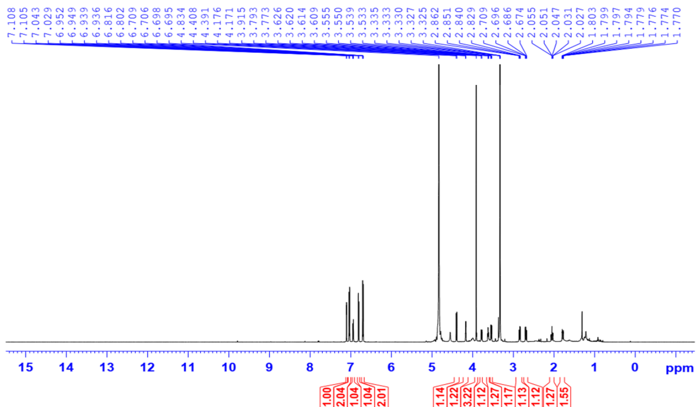
Figure S1. 1 H NMR spectrum of compound 1 (in CD 3 OD)
