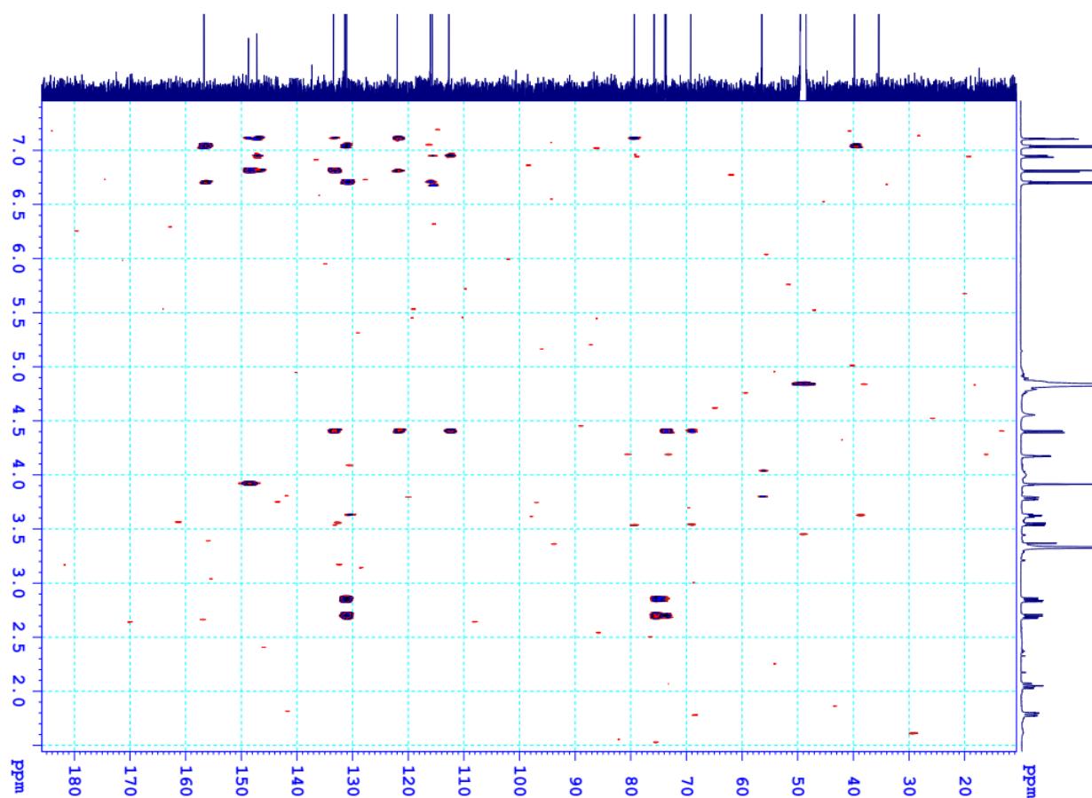
Figure S3. HMBC spectrum of compound 1 (in CD 3 OD)
