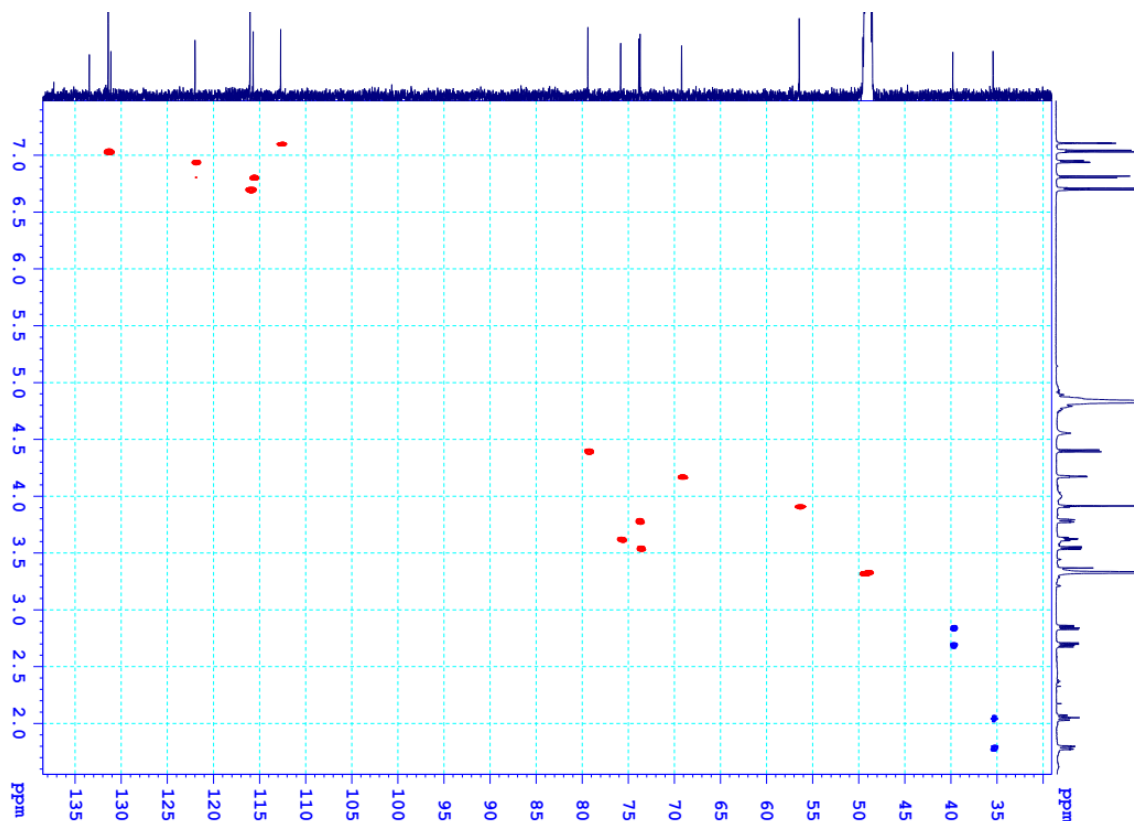
Figure S2. HSQC spectrum of compound 1 (in CD 3 OD)
