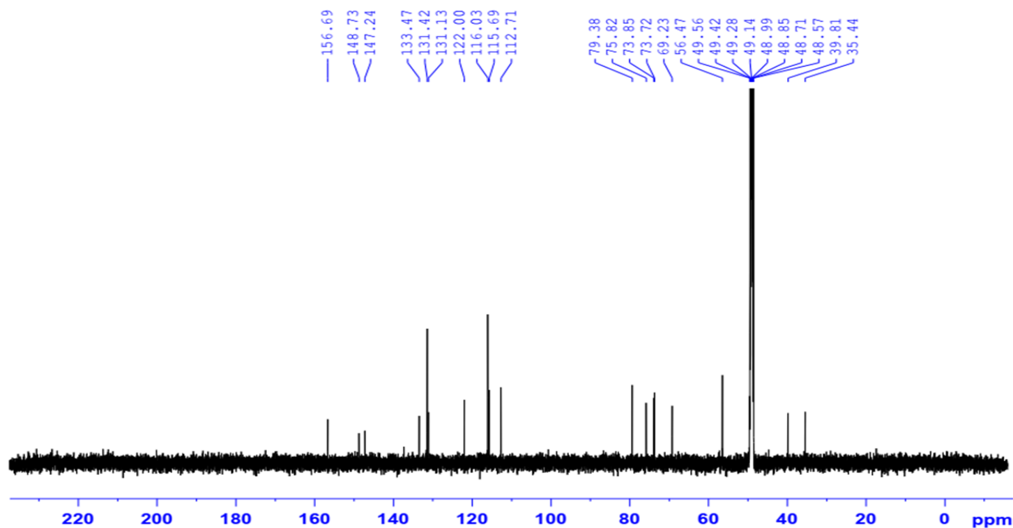
Figure S2. 13 C NMR spectrum of compound 1 (in CD 3 OD)
