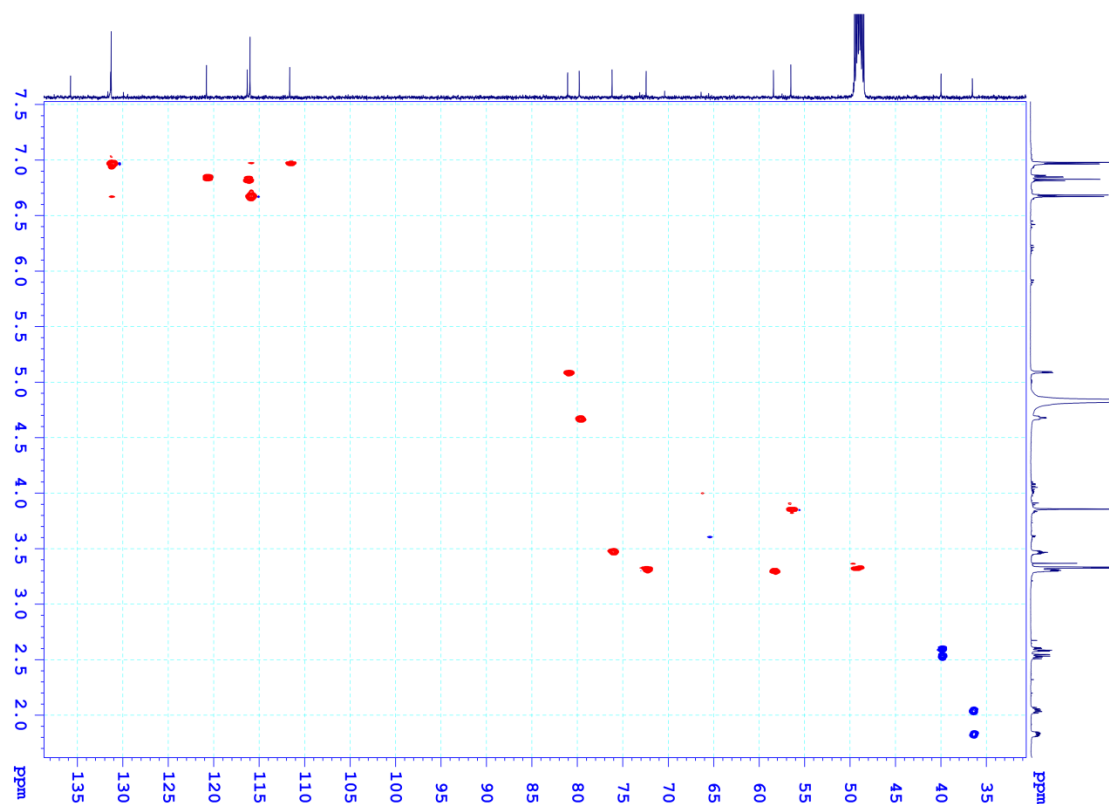
Figure S10. HSQC spectrum of compound 2 (in CD 3 OD)
