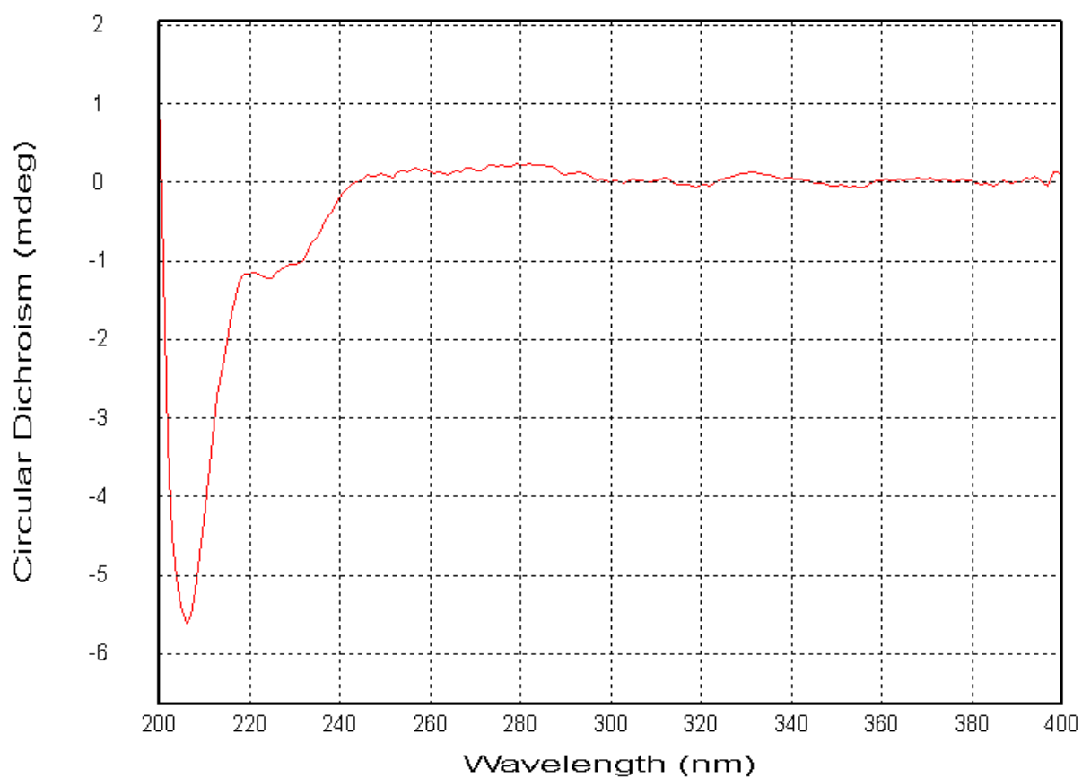
Figure S15. ECD spectrum of compound 2
