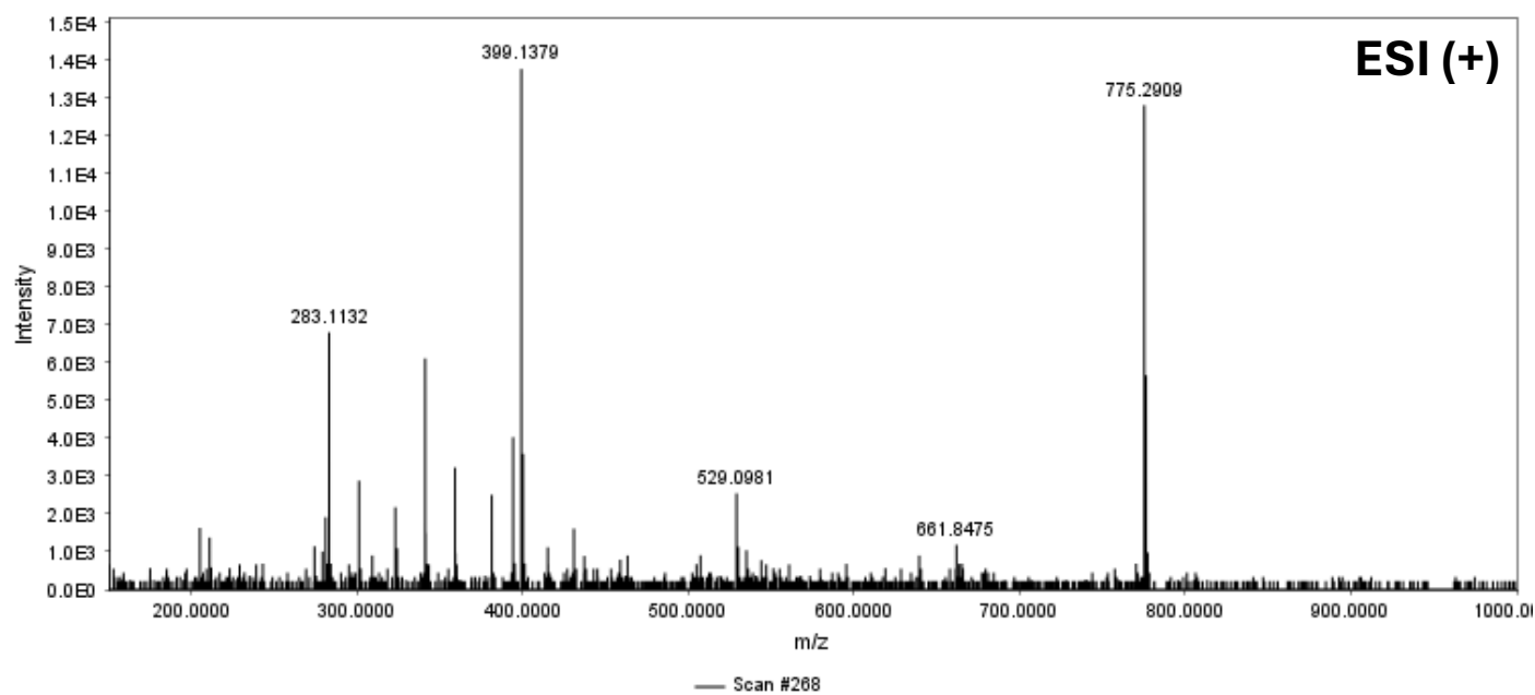
Figure S6. HR-ESI-MS spectrum of compound 1
