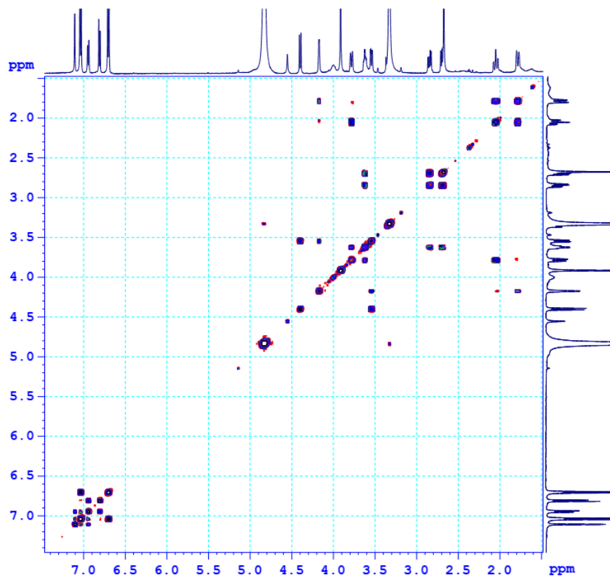
Figure S4. COSY spectrum of compound 1 (in CD 3 OD)
