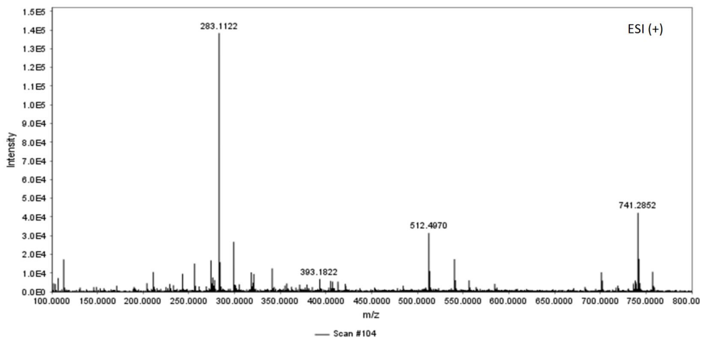
Figure S14. HR-ESI-MS spectrum of compound 2
