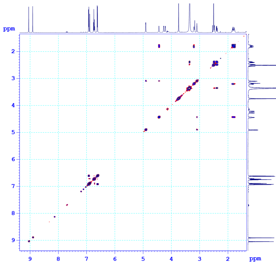
Figure S20. COSY spectrum of compound 2 (in DMSO- d 6 )
