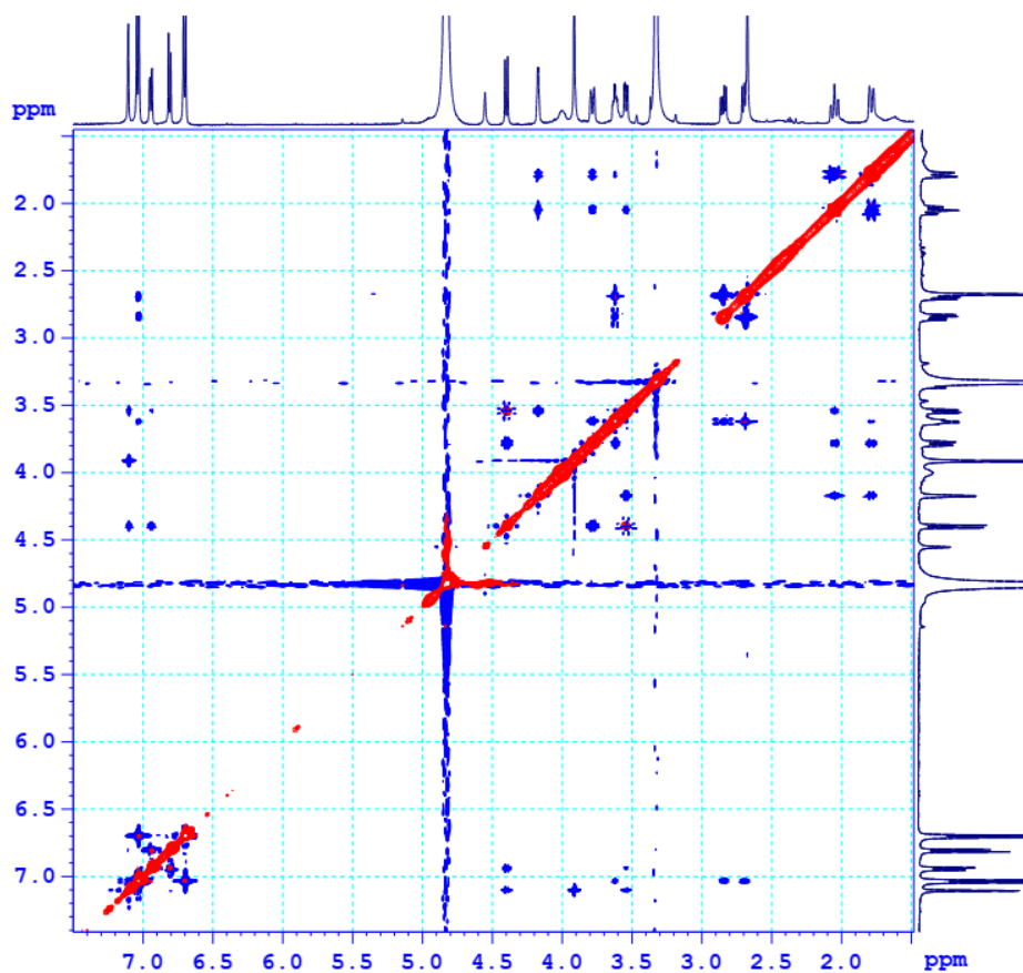
Figure S5. NOESY spectrum of compound 1 (in CD 3 OD)
