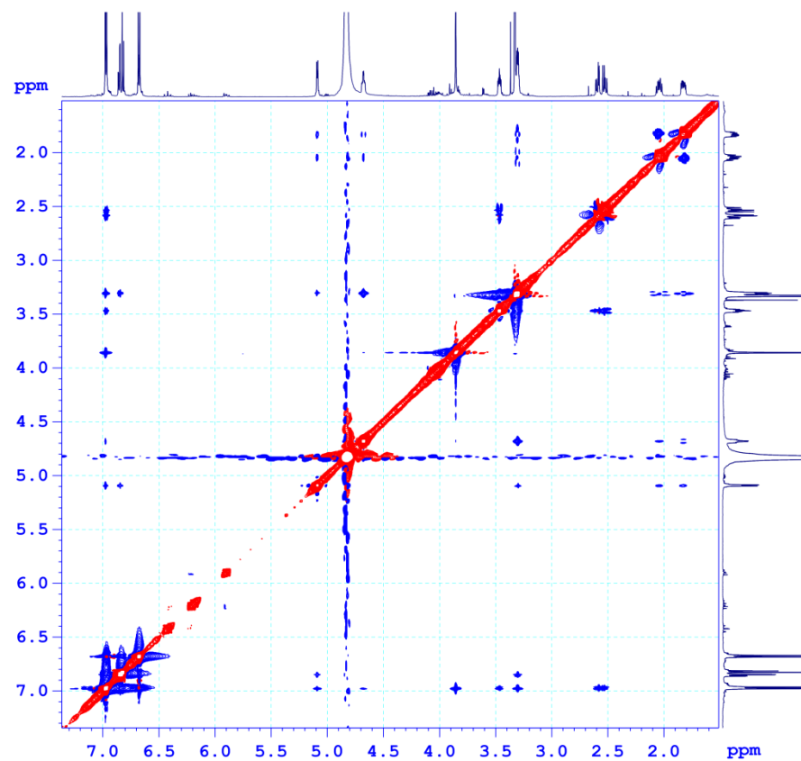
Figure S13. NOESY spectrum of compound 2 (in CD 3 OD)
