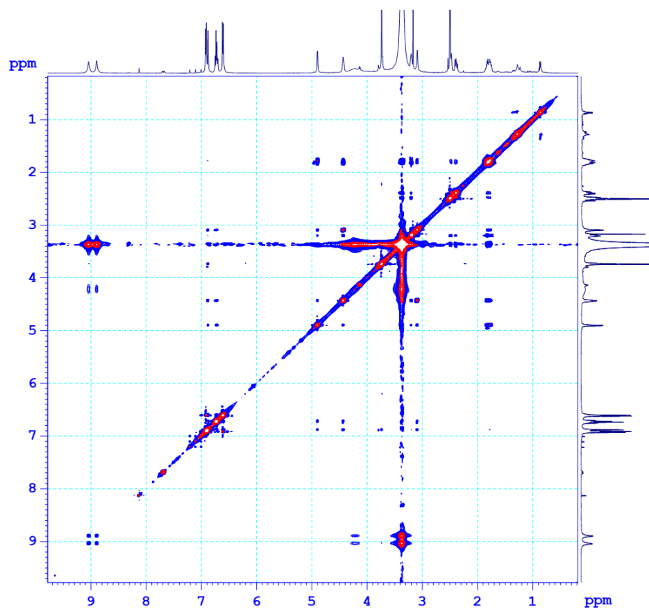
Figure S21. NOESY spectrum of compound 2 (in DMSO- d 6 )
