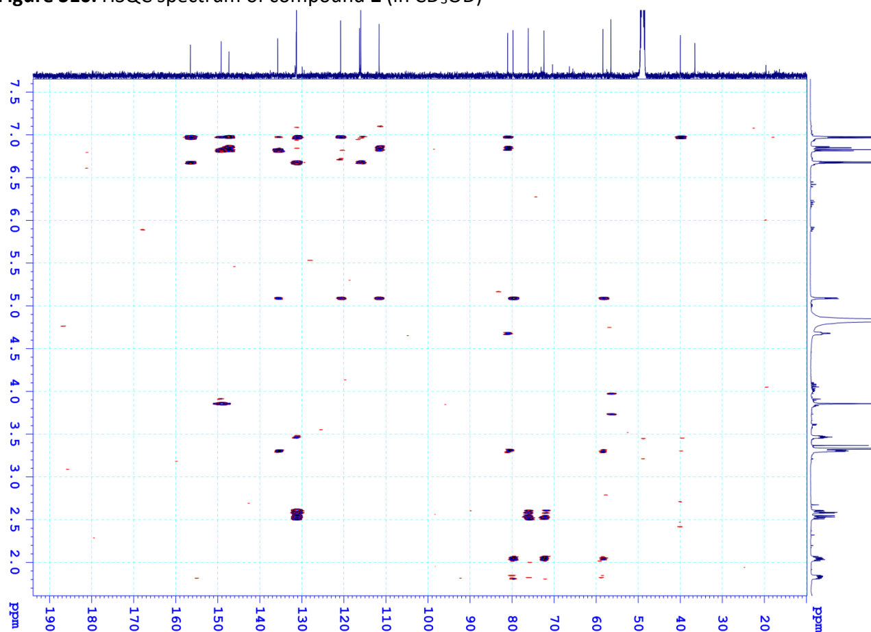
Figure S11. HMBC spectrum of compound 2 (in CD 3 OD)
