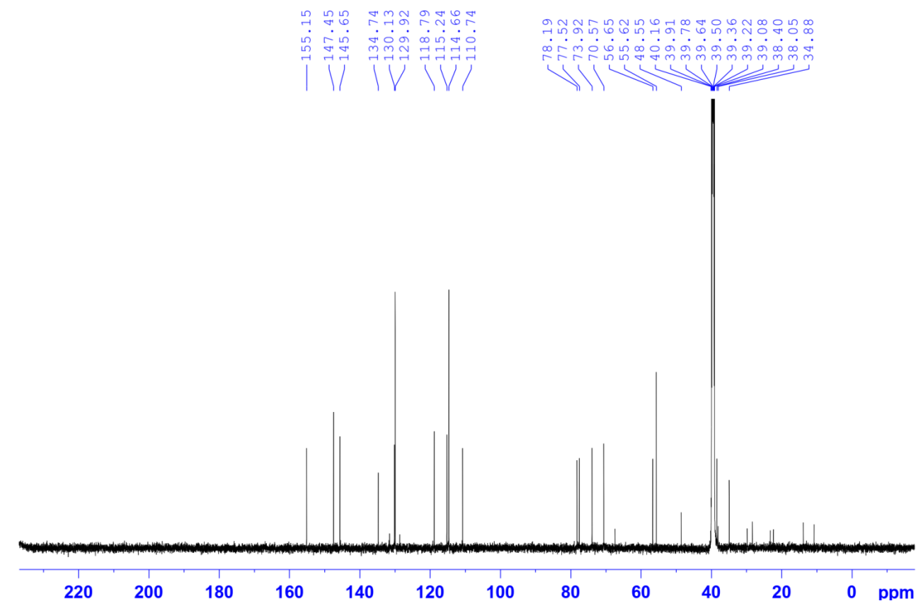
Figure S17. 13 C NMR spectrum of compound 2 (in DMSO- d 6 )
