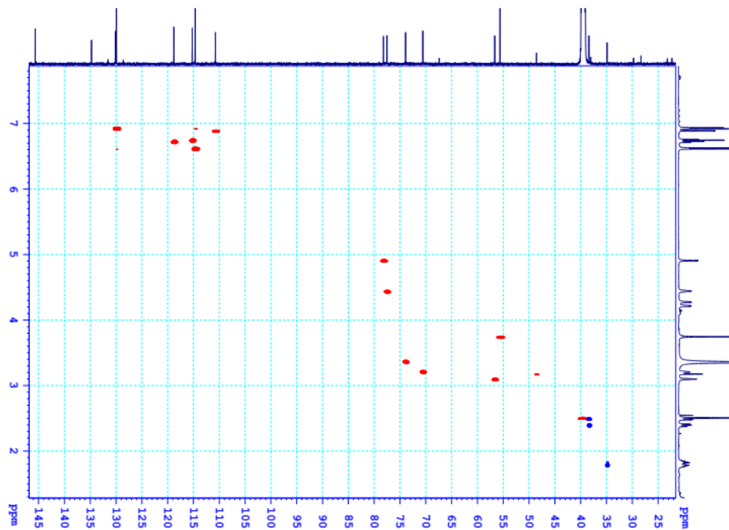
Figure S18. HSQC spectrum of compound 2 (in DMSO- d 6 )
