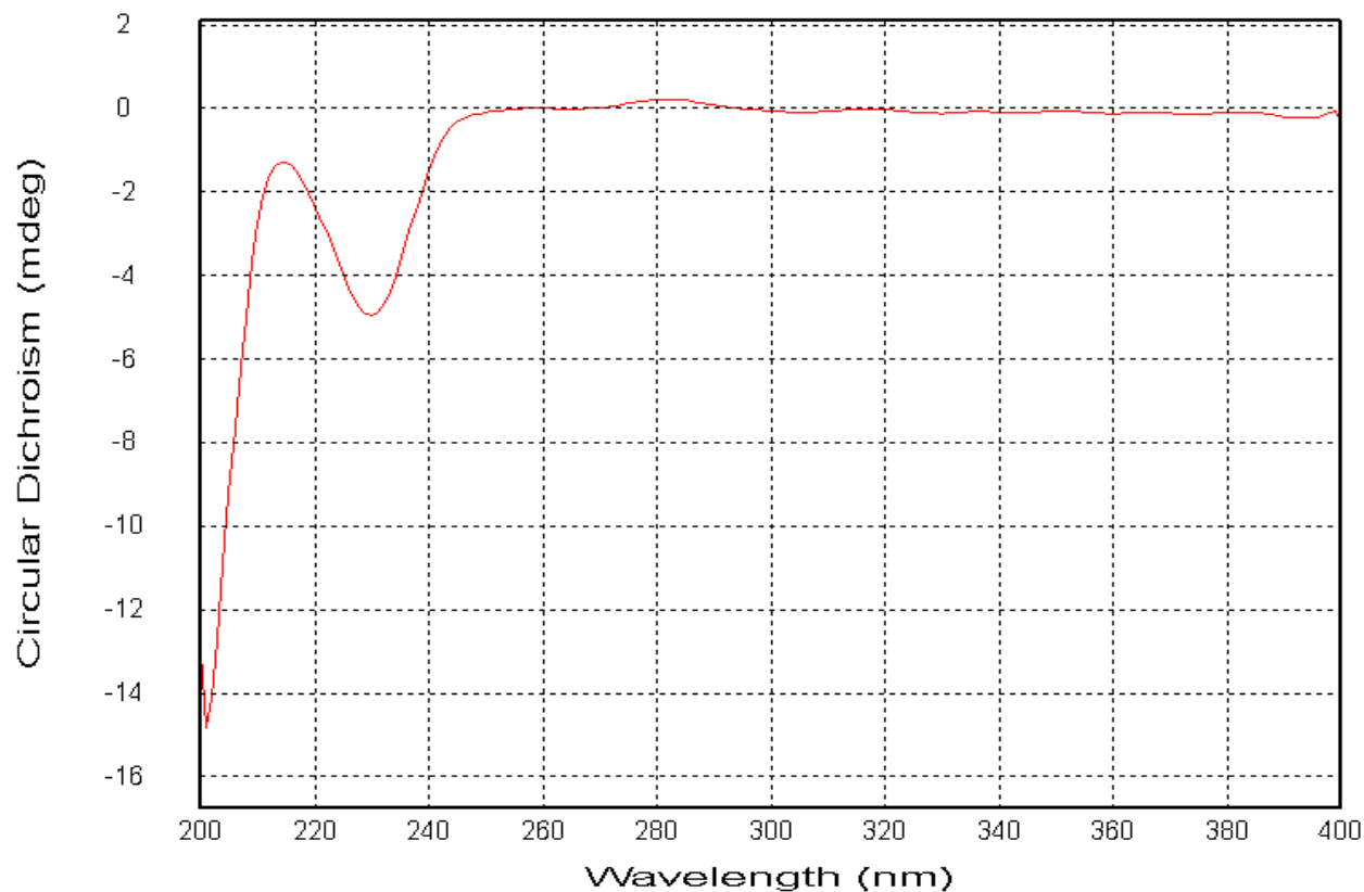
Figure S7. ECD spectrum of compound 1
