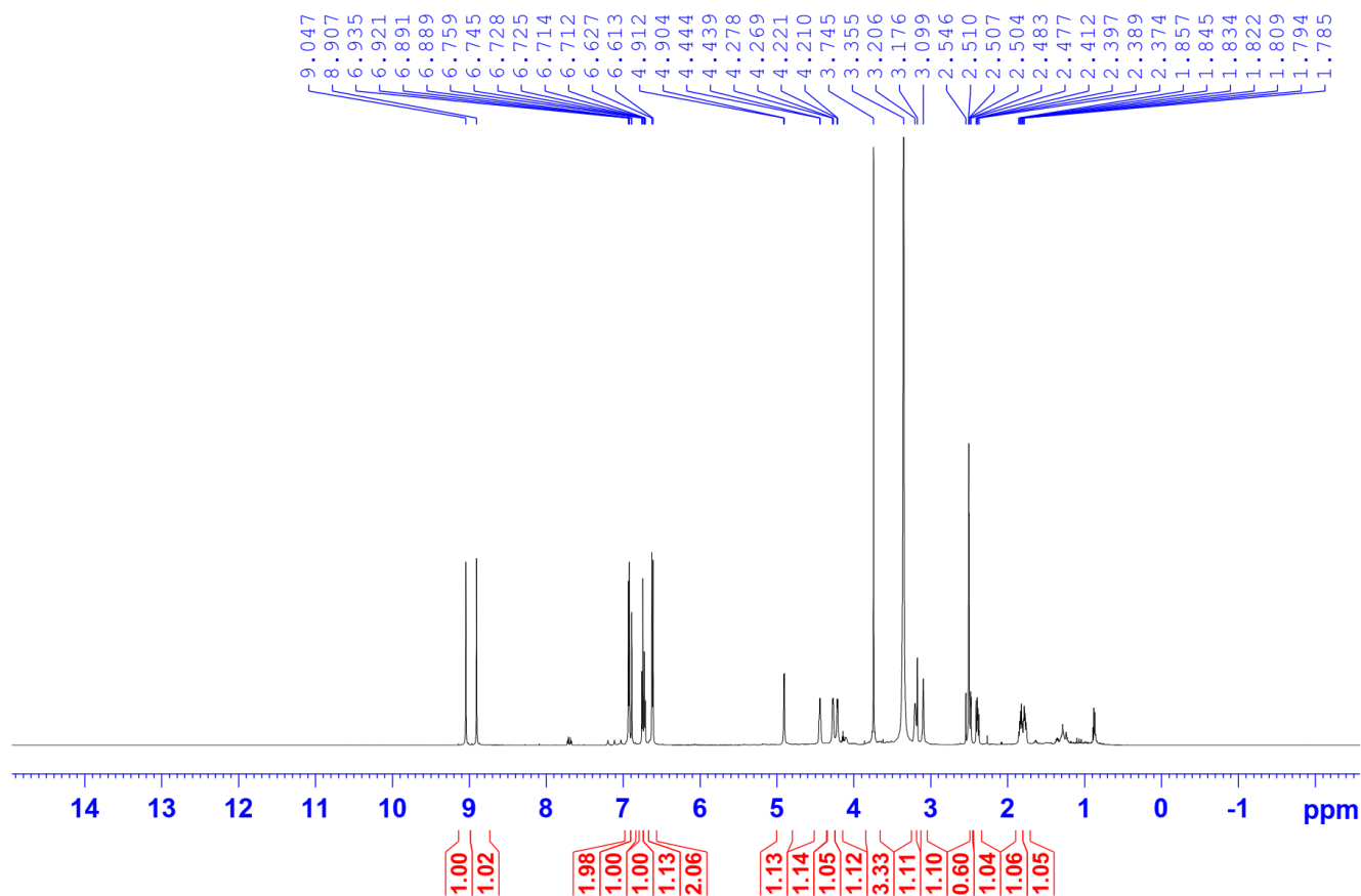
Figure S16. 1 H NMR spectrum of compound 2 (in DMSO- d 6 )
