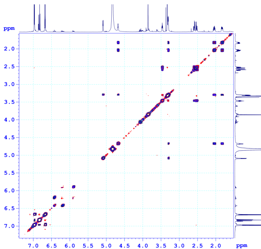
Figure S12. COSY spectrum of compound 2 (in CD 3 OD)
