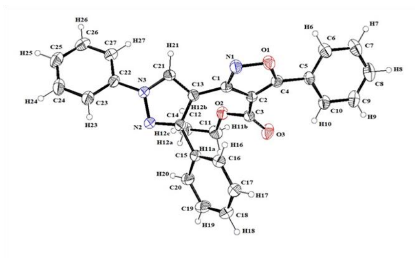
Figure 3. ORTEP view of ethyl-3-(1,3-diphenyl-1H-pyrazol-4-yl)-5-phenylisoxazole-4-carboxylate ( 2a ) (CCDC No. 2343634).
