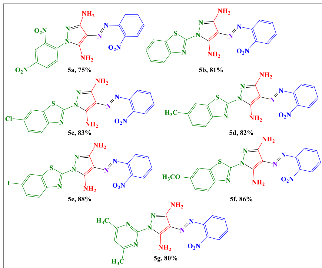
Figure 1. Substrate Scope.
