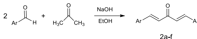
Figure 3. The general synthesis reaction of penta-1,4-diene-3-one derivatives
