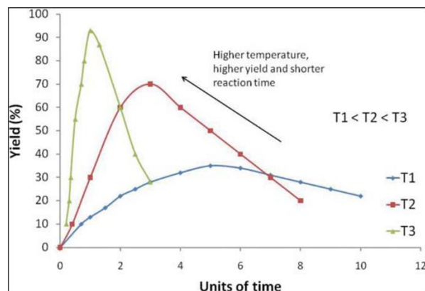
Figure 9. Influence of time and temperature upon the product yield for the same competitive thermal process performed at temperatures of T1 (lowest), T2 and T3 (highest). Reproduced from ref. 11 with permission.
