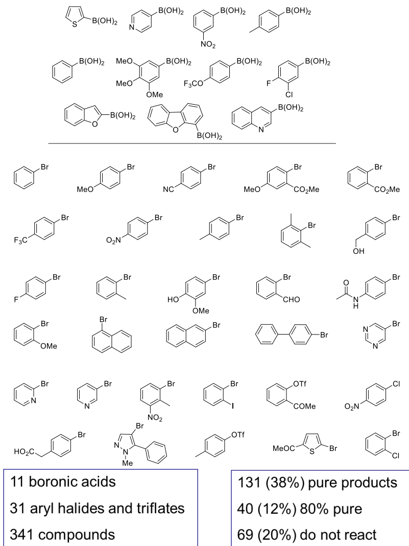
Figure 19. Suzuki coupling partners employed in library preparation.
