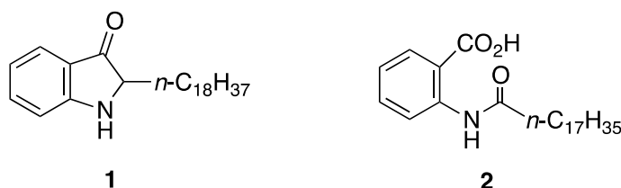
Figure 1. Structures of alleged fistulosin 1 and the likely structure 2-(1-oxooctadecyl)aminobenzoic acid ( 2 ).
