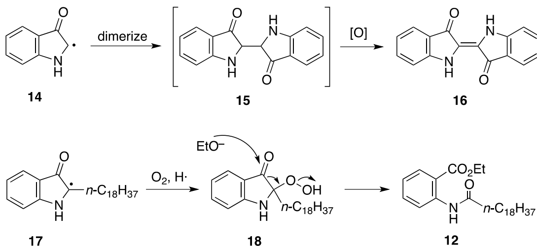
Scheme 2. A proposed mechanism for the formation of ethyl 2-(1-oxononadecyl)aminobenzoate ( 12 ).
