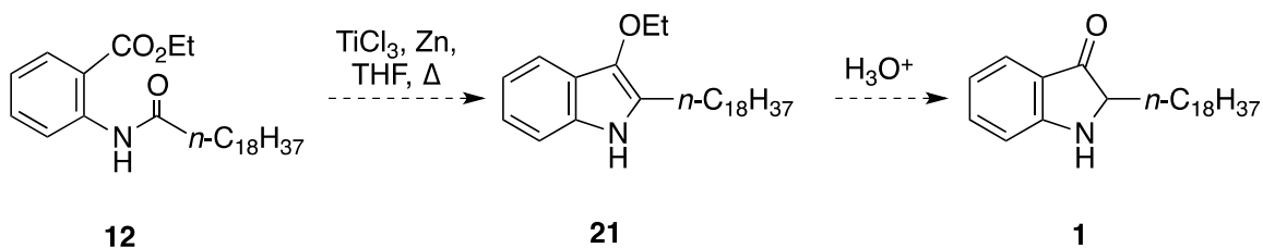
Scheme 4. A proposed route to 1 from 12 , which remains to be seen.
