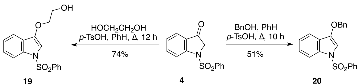
Scheme 3. A new synthesis of 3-alkoxyindoles 19 and 20 from indoxyl 4 .
