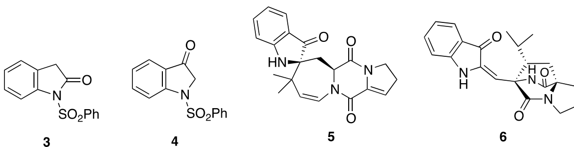
Figure 2. Structures of oxindole 3 and indoxyls 4–6 .
