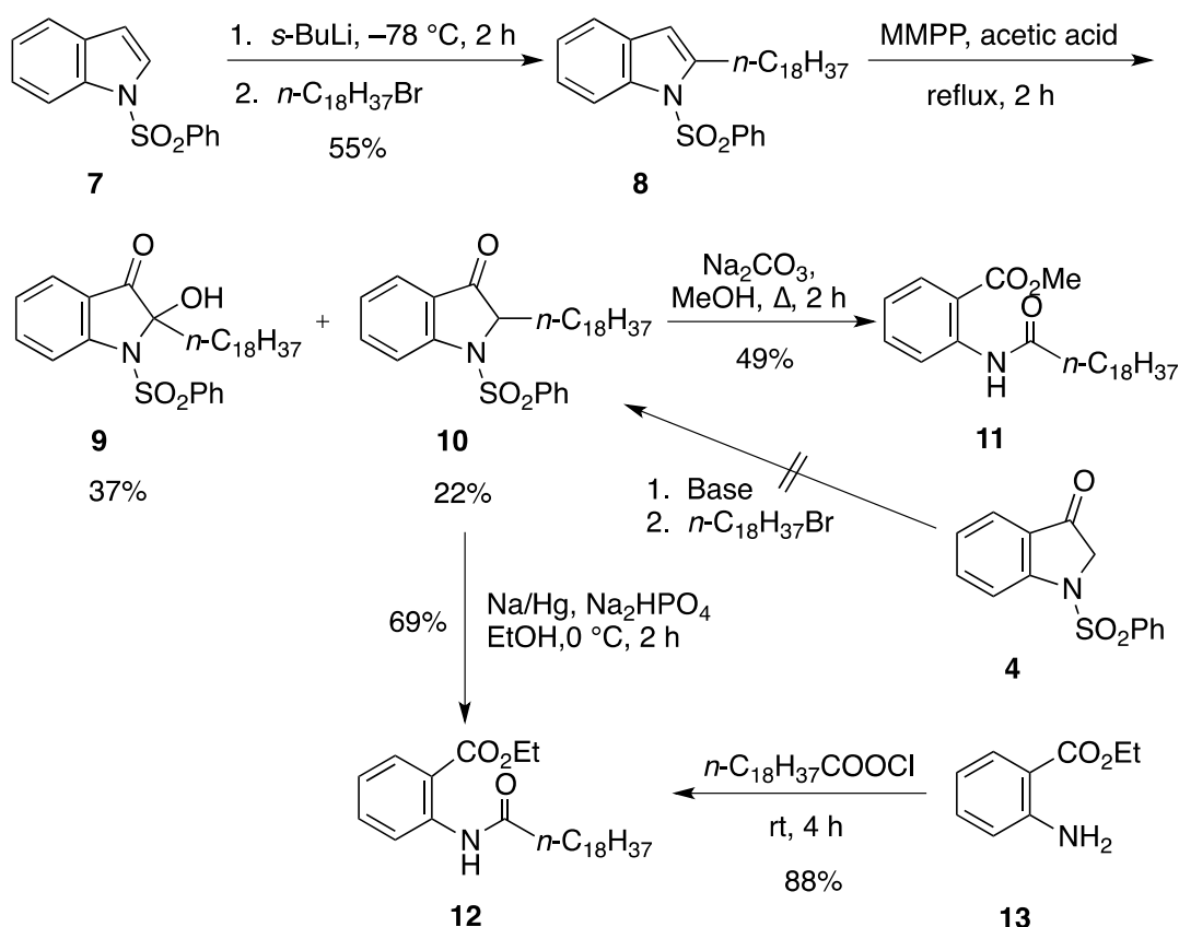
Scheme 1. Our attempted synthesis of 1 via the de-phenylsulfonylation cleavage of 10 .
