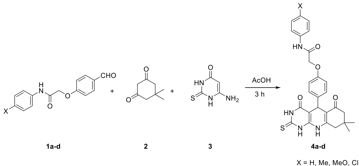
Scheme 1. Synthesis of pyrimido[4,5- b ]quinolines 4a-d .
