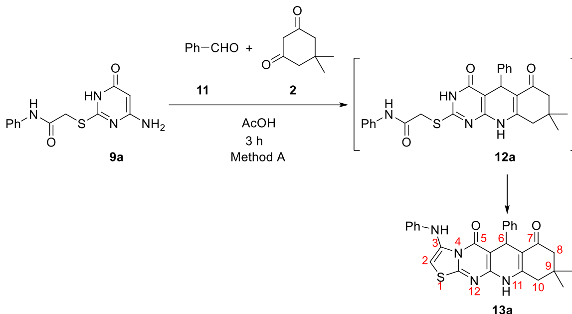
Scheme 3. A three-component synthesis of 6-phenyl-3-(phenylamino)-5H-thiazolo[3',2':1,2]pyrimido[4,5-b]quinoline 13a .
