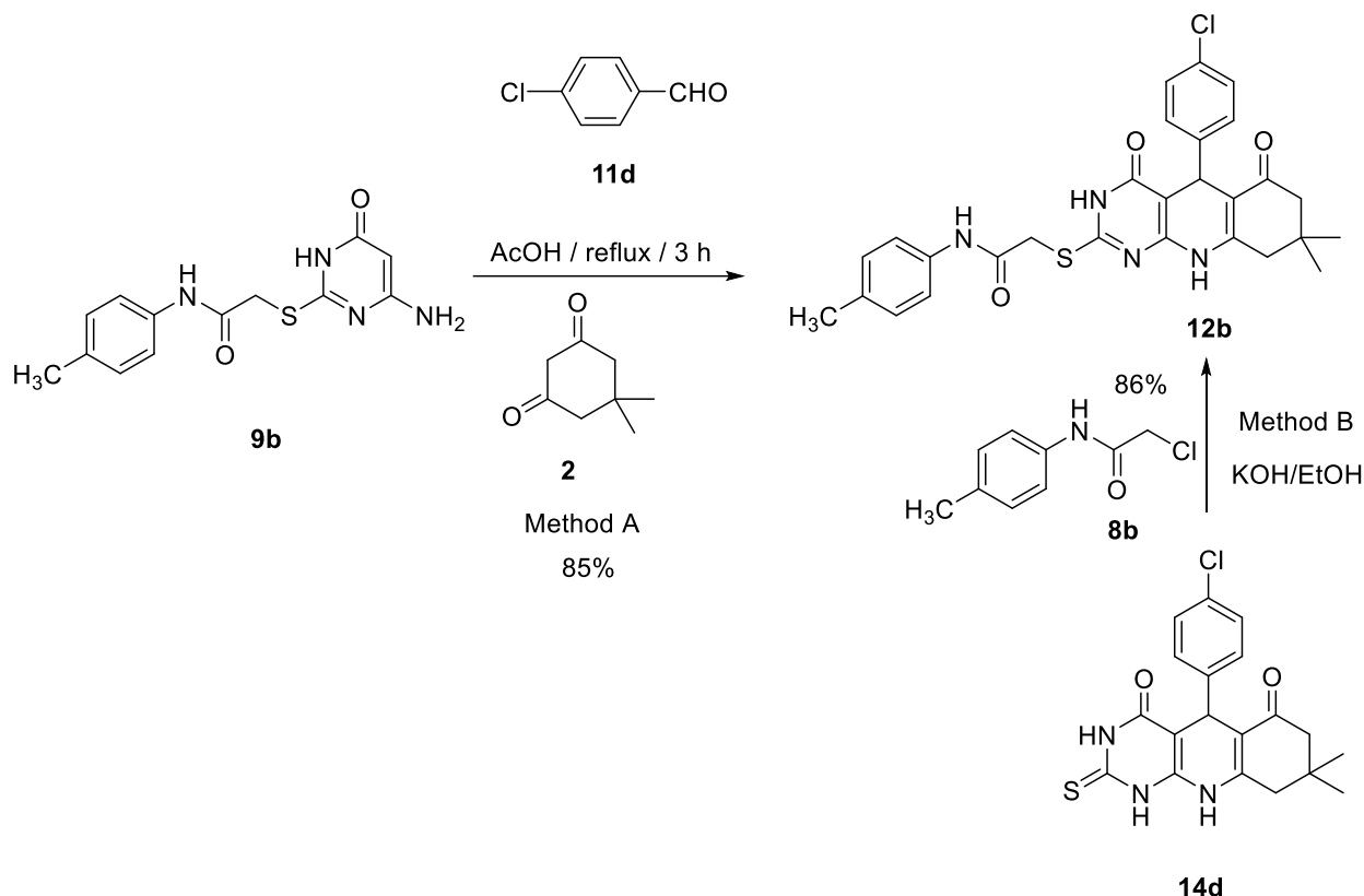
Scheme 6. Synthesis of 5-aryl-octahydropyrimido[4,5- b ]quinoline 12b .
