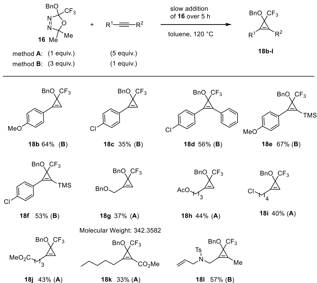
Scheme 4. Scope for the formation of cyclopropenes.
