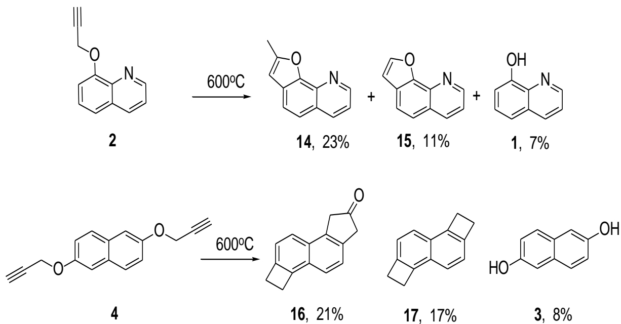
Scheme 4. FVP of propargyl ethers 2 and 4 .
