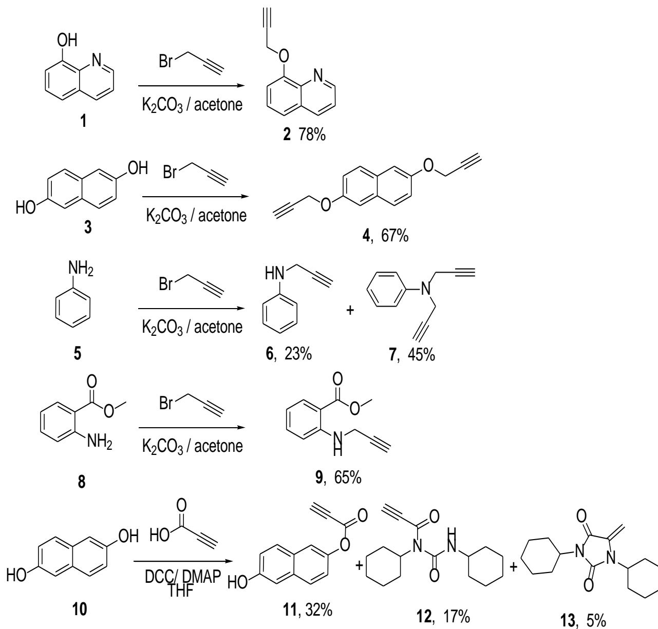
Scheme 3. Synthesis of propargyl ethers 2,4 , amines 6,7,9 , and ester 11 .
