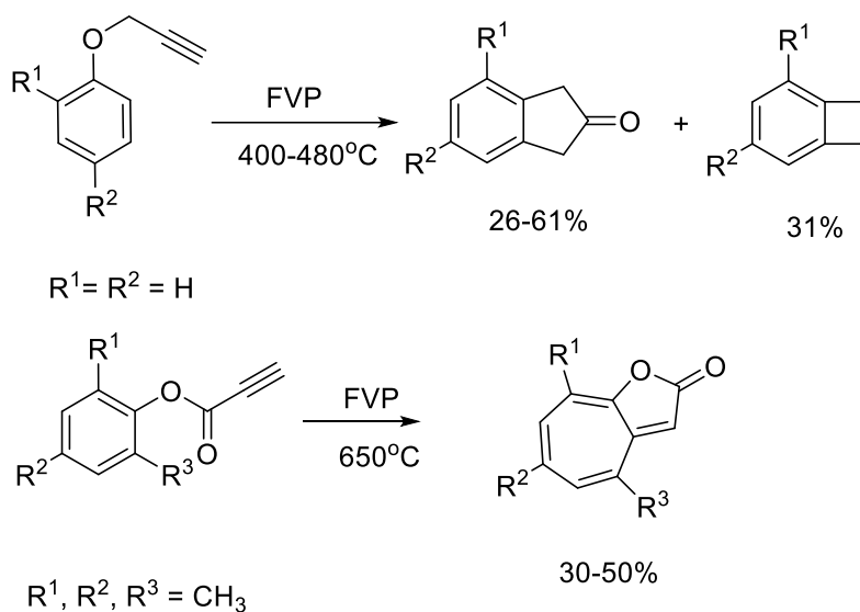
Scheme 2. FVP of aryl propargyl ethers.
