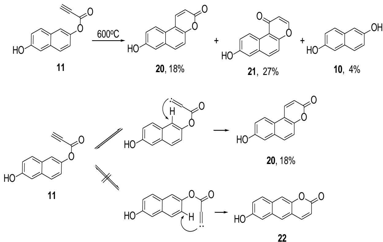
Scheme 6. FVP of acetylenic ester 11 .
