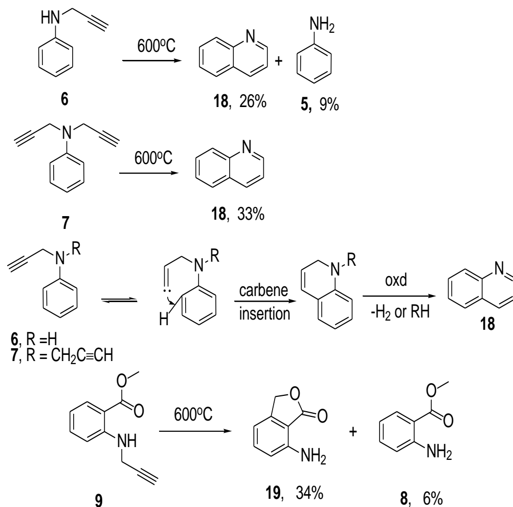
Scheme 5. FVP of propargyl amines 6-7 and 9 .
