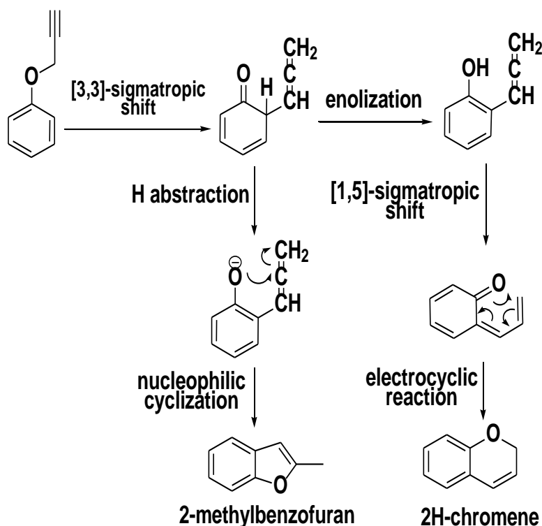
Scheme 1. Formation of benzofuran and chromene via Claisen rearrangement.
