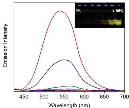
Figure 4. Fluorescence spectra of 2 at 50 \mu M in toluene/DMSO mixtures. ( \lambda_{\text{ex}}=386 nm) Inset: photographs of solutions of 1 in solvent mixtures of various toluene fractions (vol %), taken under UV irradiation at 365 nm. (red: 95%, blue: 90%, olive: 70%, magenta: 50%, orange: 30%, violet: 10%, black: 0%).
