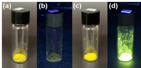
Figure 3. Images of the solid powder forms of (a, b) 1 and (c, d) 2 were captured in two lighting conditions: (a, c) ambient room lighting and (b, d) illumination with a 365 nm UV lamp.
