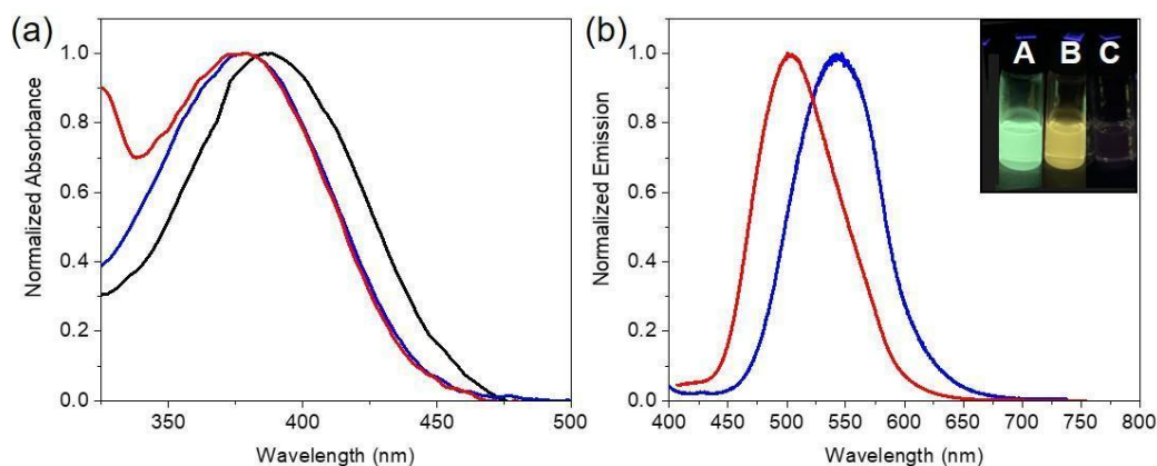
Figure 2. Normalized (a) UV-vis absorption and (b) fluorescence emission spectra of 2 at 50 \mu\text{M} in toluene (red), EA (blue) and DMSO (black). Insets are the photographs of solutions of 2 in (A) toluene, (B) EA and (C) DMSO, taken under UV irradiation at 365 nm.
