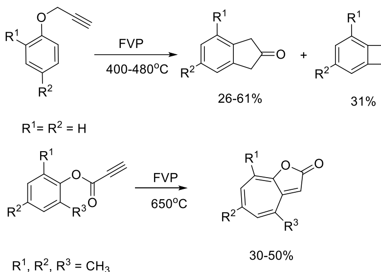
Scheme 2. FVP of aryl propargyl ethers
