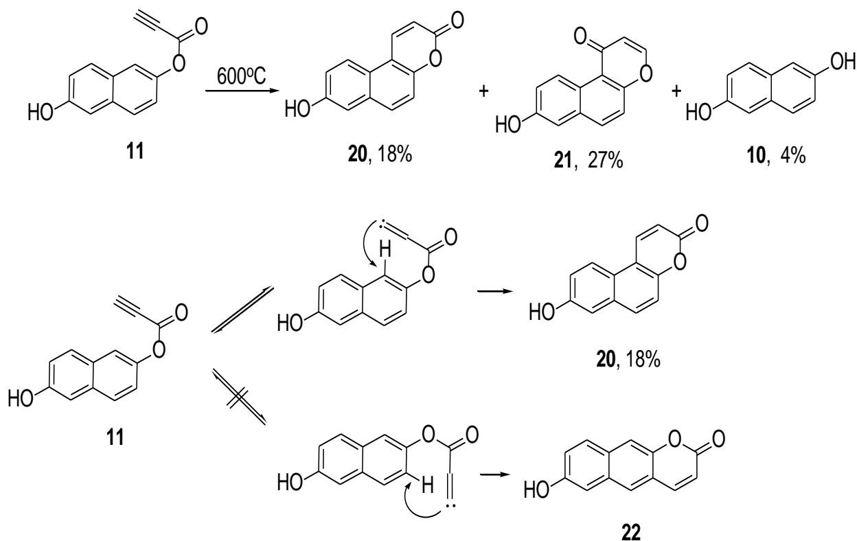
Scheme 6. FVP of acetylenic ester 11 .
