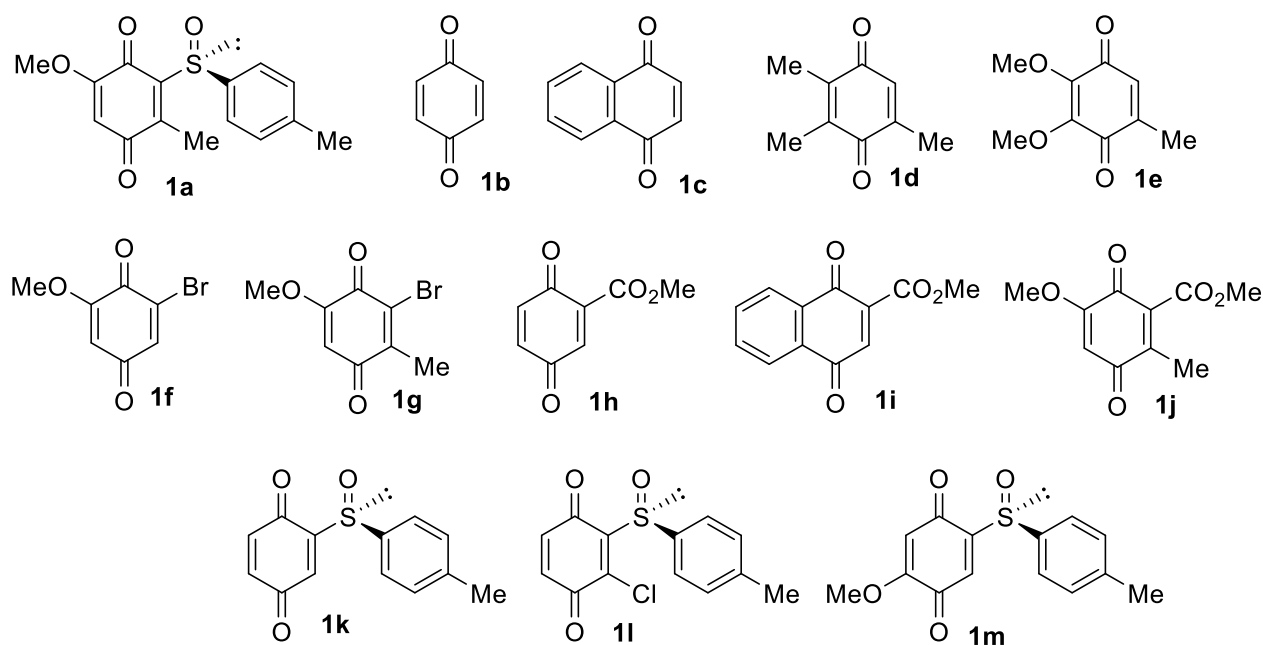
Figure 2. Structures of the quinones studied in this work.
