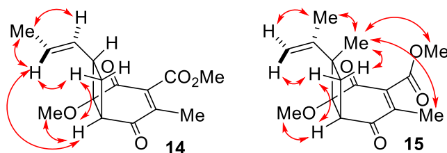
Figure 3. Tridimensional representation of products 14 and 15 and n.O.e correlations.
