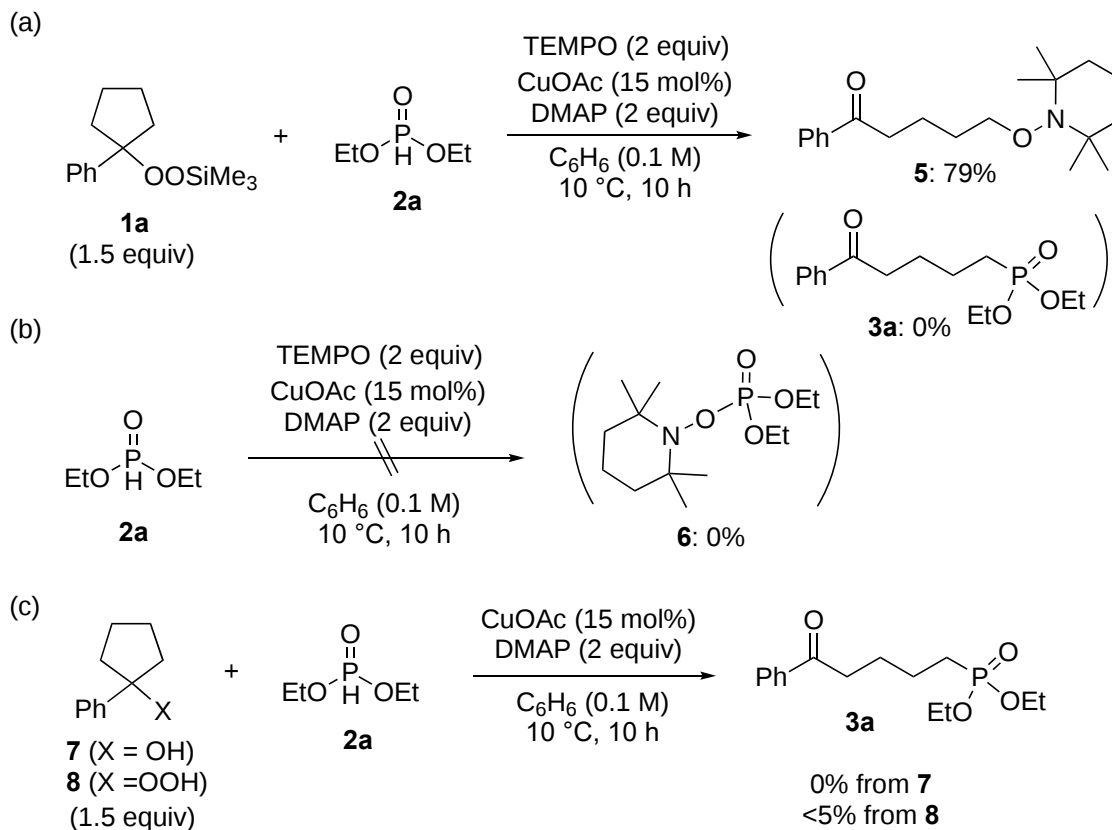
Scheme 2. Control experiments
