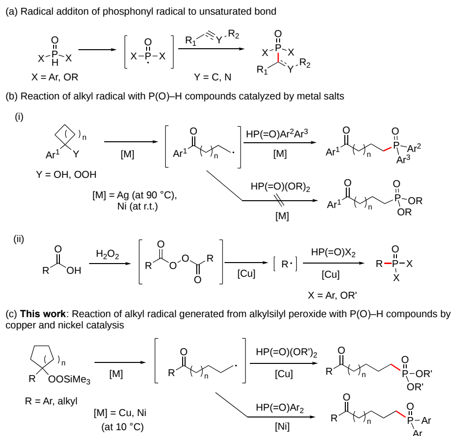
Scheme 1. Radical-mediated C–P coupling reactions
