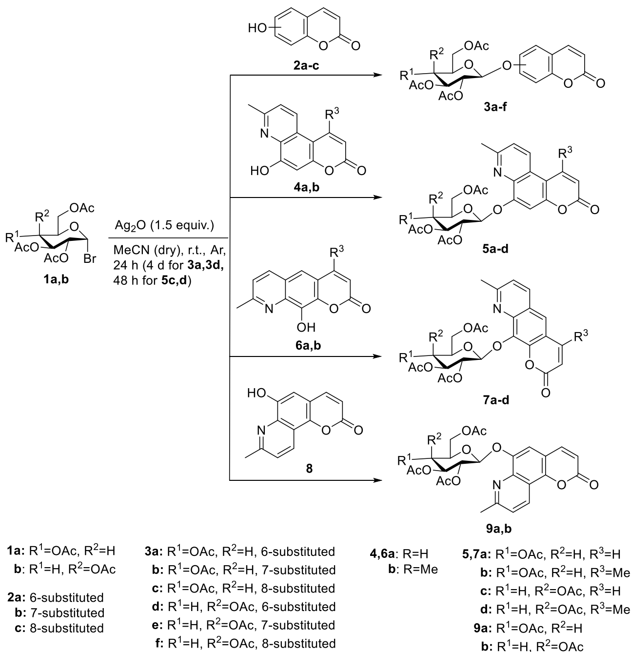
Scheme 1. Synthesis of \beta -glycosides of coumarins and fused pyridocoumarins.
