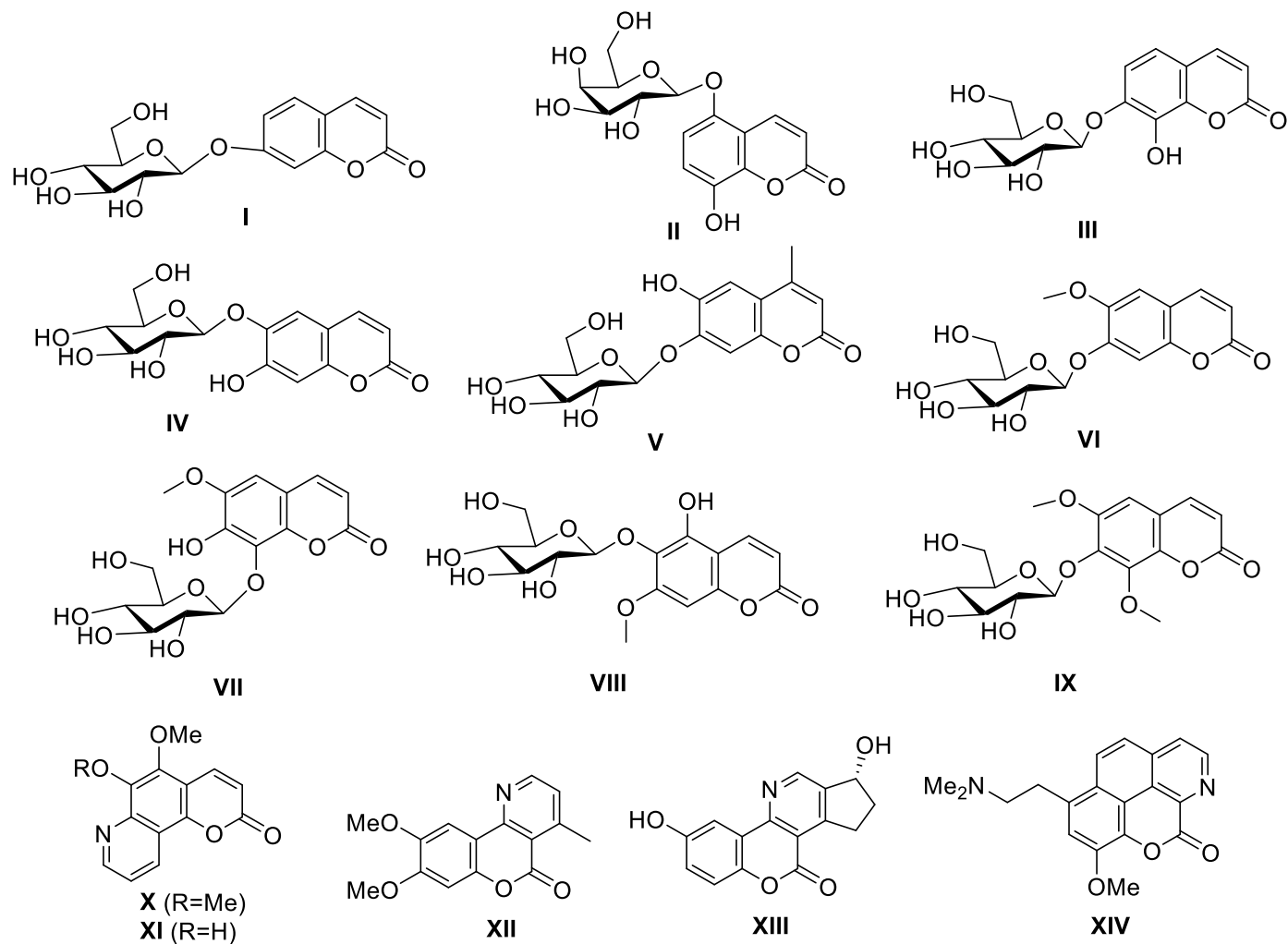
Figure 1. Natural coumarin \beta -glycosides and fused pyridocoumarins with biological activity.
