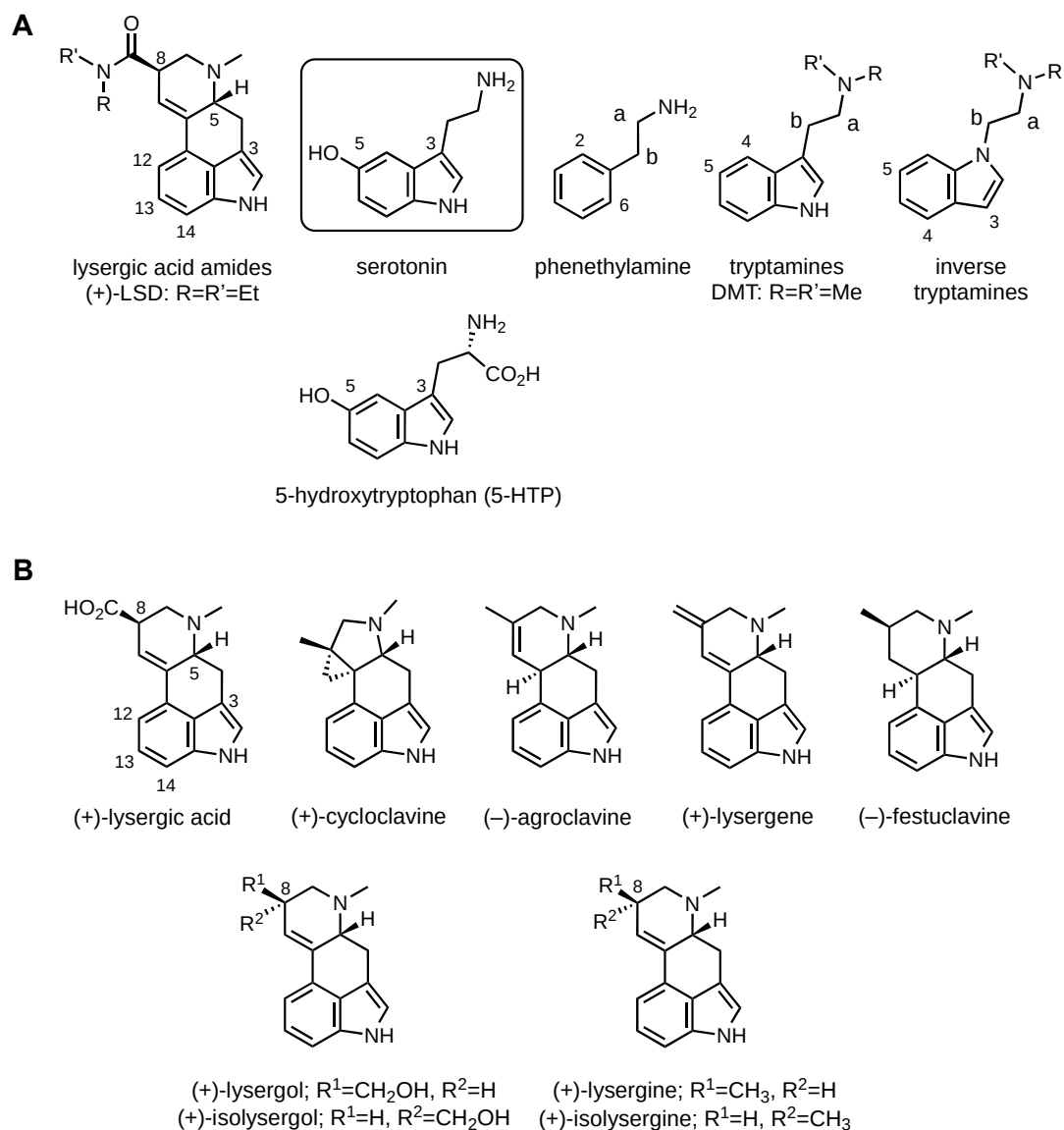
Fig. 1. Panel A: Serotonin, 5-hydroxytryptophan (5-HTP) and synthetic 5-HTR ligands. Panel B: Lysergic acid and representative ergot (lysergic acid, lysergol) and clavine (cycloclavine, agroclavine, lysergene, festuclavine, lysergine) natural products.
