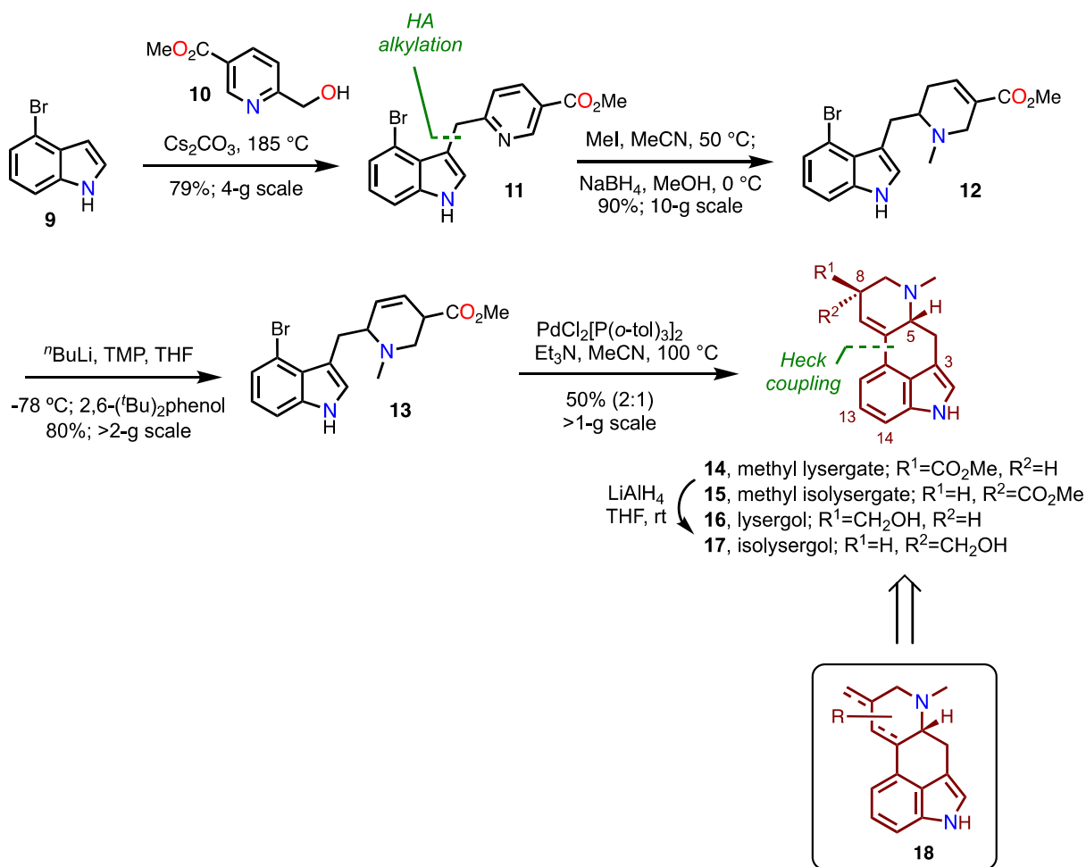
Scheme 2. Overview of a 5-step total synthesis of lysergols that serves as a segue to the preparation of other clavine alkaloids 18 . 17
