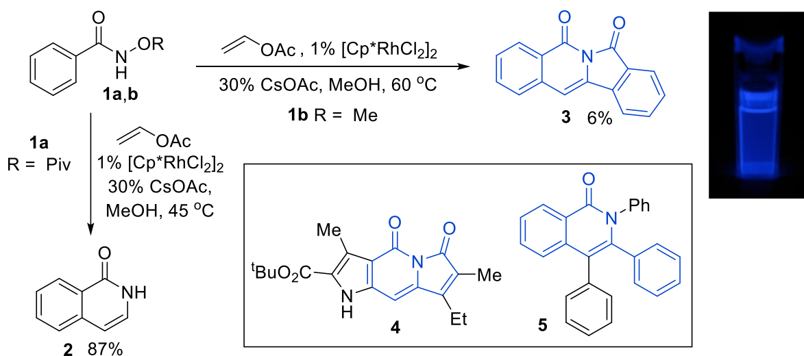
Scheme 1. Adventitious synthesis of fluorescent heterocycle 3 and similarity to previously reported fluorophores 4 and 5 .
