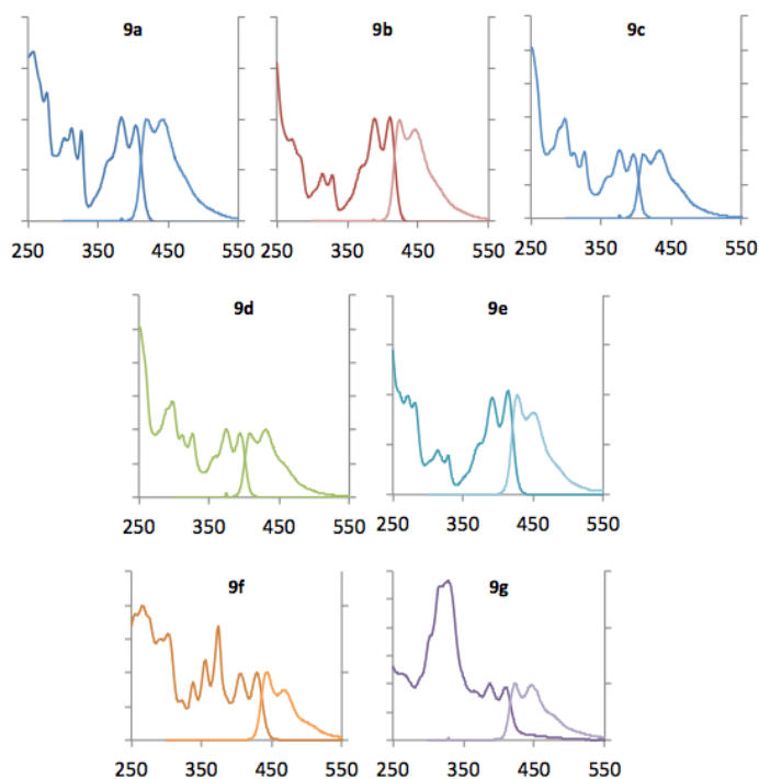
Figure 1. Absorption/emission spectra for 9a-9g . Absorption maxima normalised to A = 1.0 , fluorescence spectra in arbitrary units.
