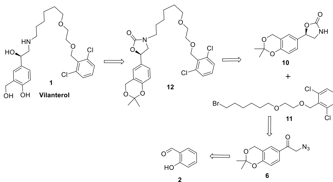
Scheme 2. Retrosynthesis of Vilanterol
