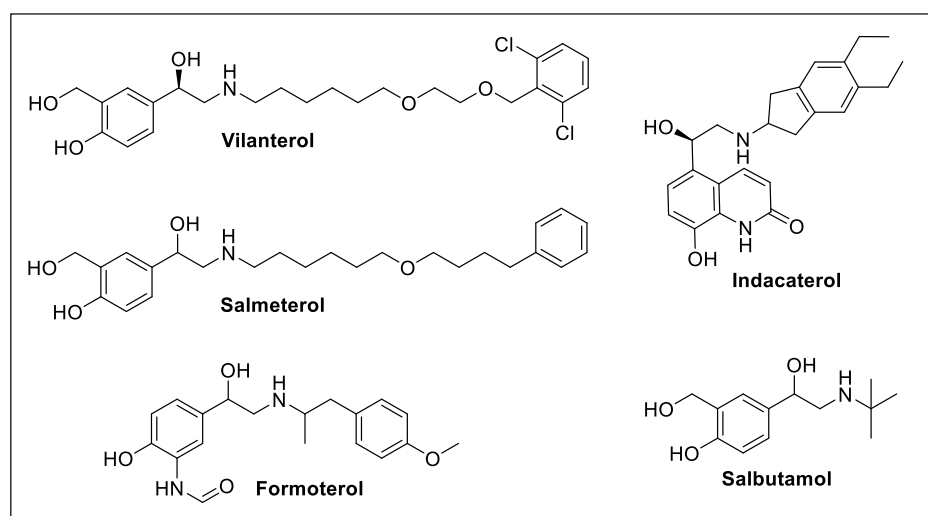
Scheme 1. Asthma and COPD potent drugs
