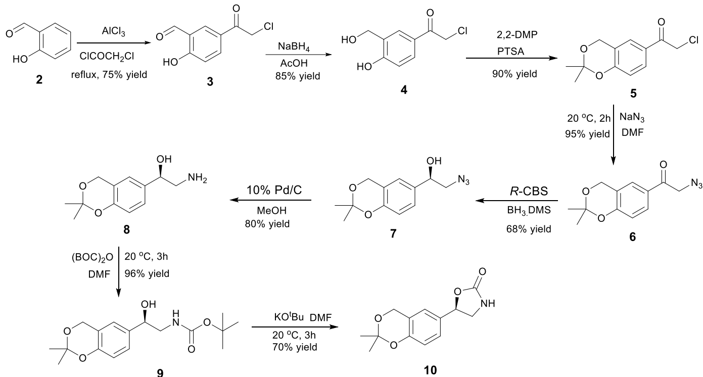
Scheme 3. Synthesis of oxazolidinone compound ( 10 )
