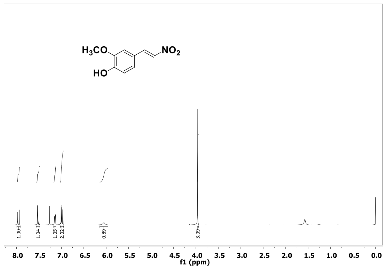
1 H NMR Spectrum of compound 3 in CDCl 3 (400 MHz)
