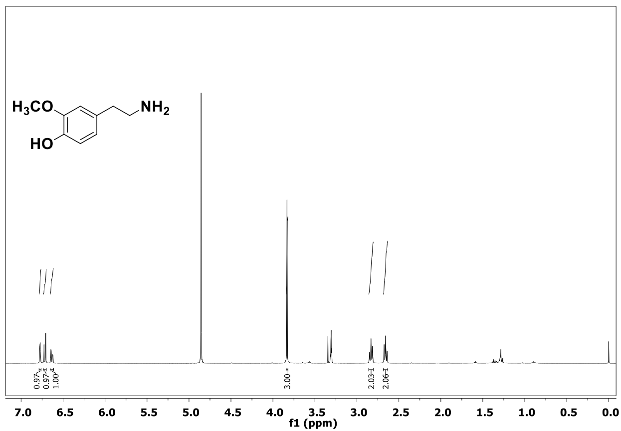
^1\text{H} NMR Spectrum of compound 4 in \text{CD}_3\text{OD} (400 MHz)
