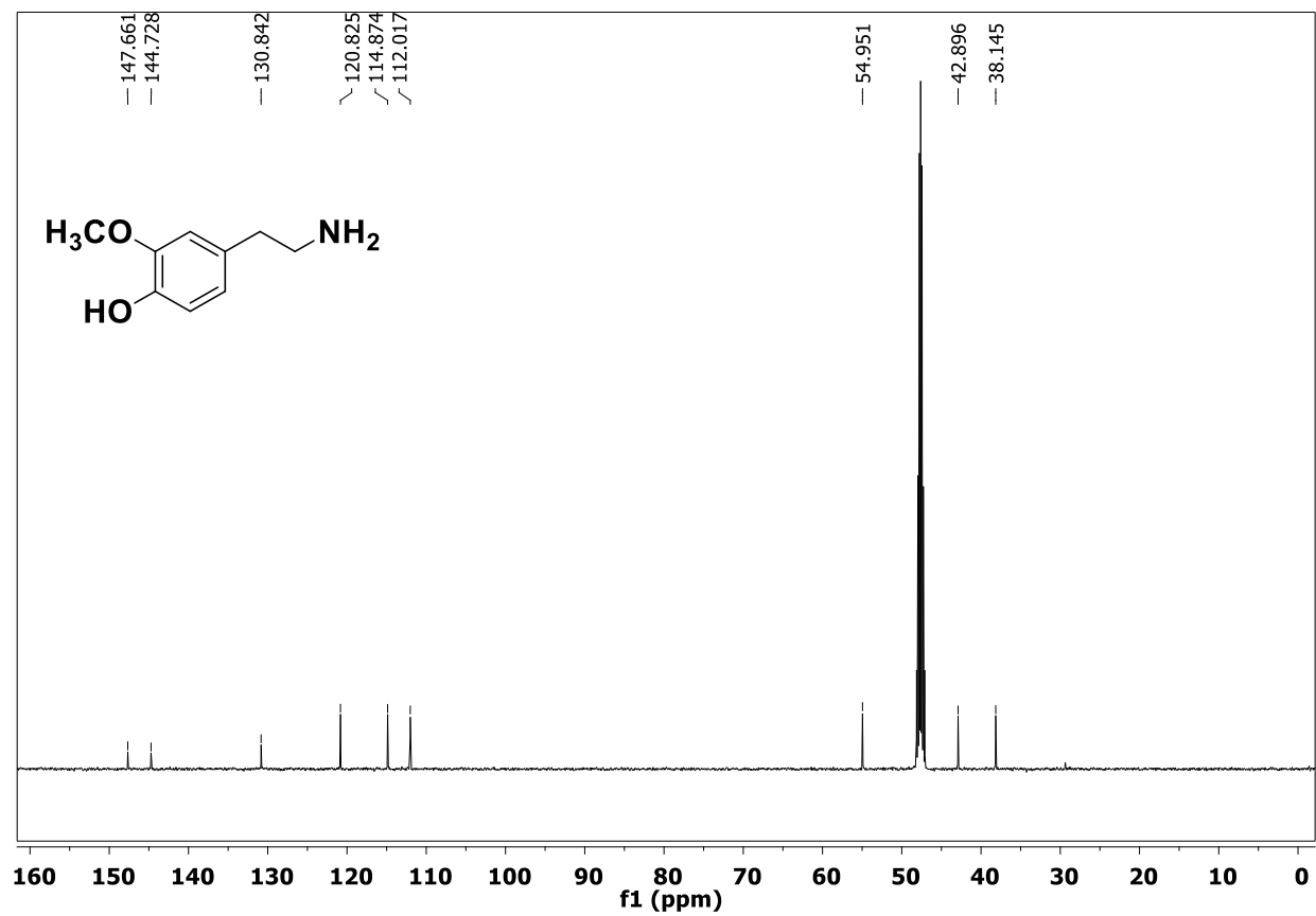
^{13}\text{C} NMR spectrum of compound 4 in \text{CD}_3\text{OD} (126 MHz)
