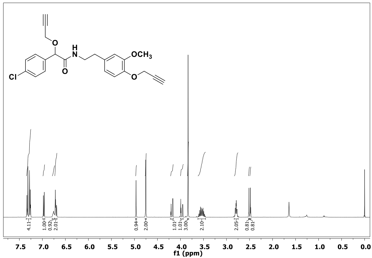
1 H NMR spectrum of compound 1 in CDCl 3 (400 MHz)
