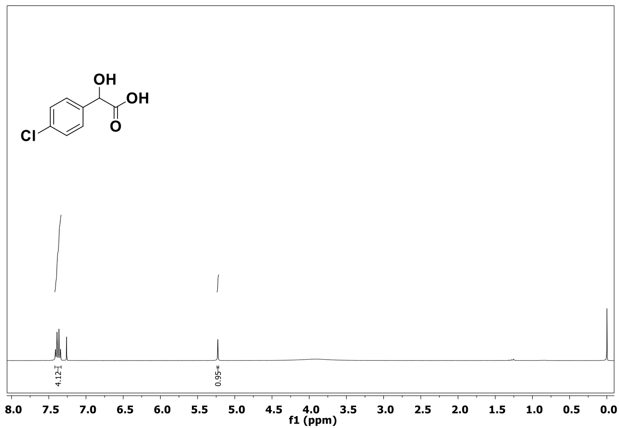
^1\text{H} NMR spectrum of compound 6 in \text{CDCl}_3 (400 MHz)
