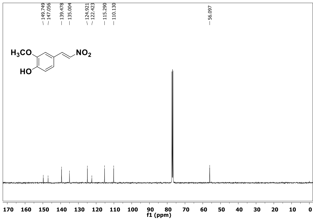
13 C NMR spectrum of compound 3 in CDCl 3 (101 MHz)
