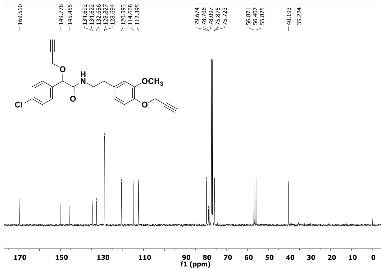
13 C NMR spectrum of compound 1 in CDCl 3 (101 MHz)
