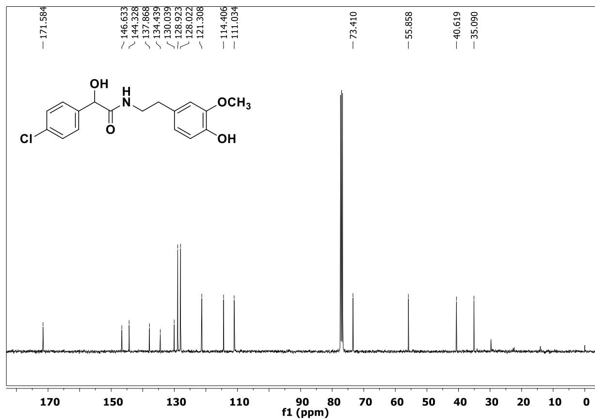
13 C NMR spectrum of compound 7 in CDCl 3 (101 MHz)
