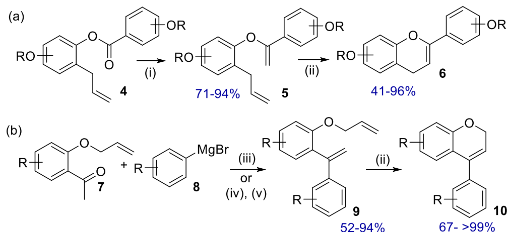
Scheme 1. The synthesis of flav-2-enes ( 6 ) and neoflav-3-enes ( 10 ) with ring-closing metathesis as key step. Reaction conditions: (i) Tebbe reagent (0.5 M, 1.2 – 2.7 eq.), THF (2 mL), 0 °C, 30 min., rt, 1 h, reflux, 2 h; (ii) GII (5 mol%), CH 2 Cl 2 , reflux; (iii) Al(OTf) 3 (1 eq.), Et 2 O, -30 °C – rt; (iv) THF, -60 °C – rt; (v) anhydrous CuSO 4 , hexane, reflux.
