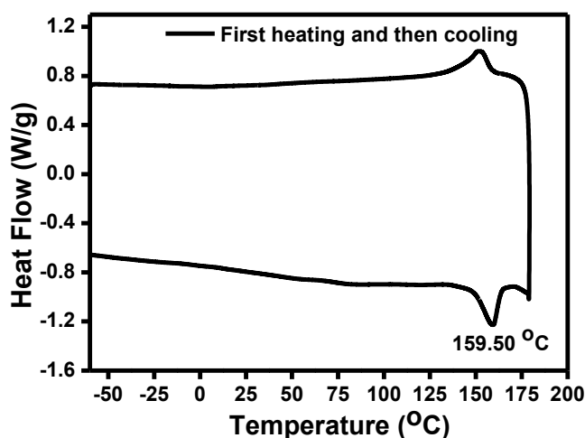
Figure 6. DSC curves of cholesterol based oxa -triquinane ( 15 )
