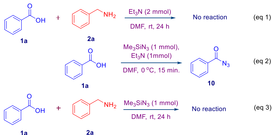
Scheme 2. Control experiments.
