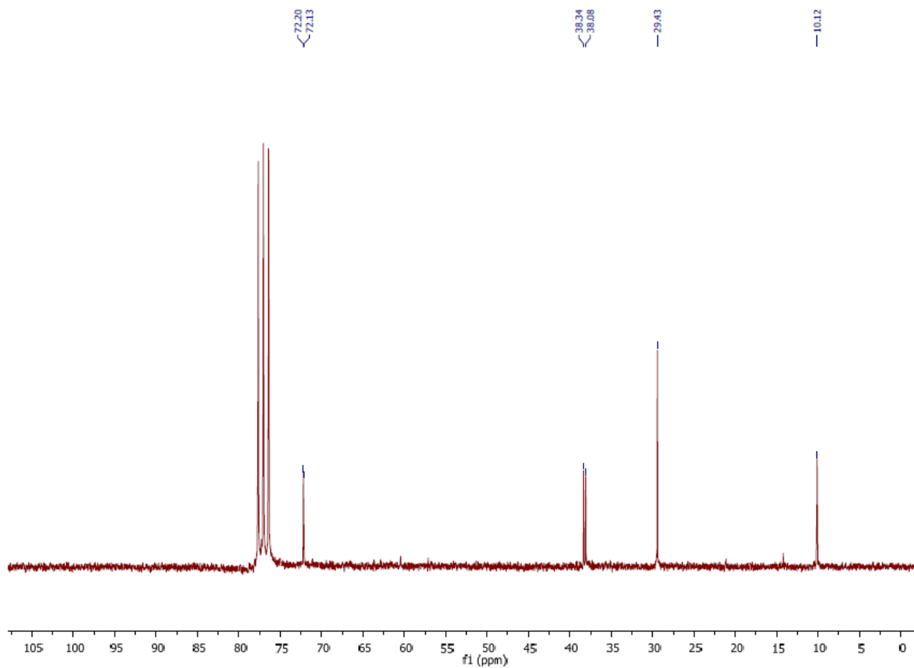
^{13}\text{C} NMR spectrum of compound 3e ( \text{CDCl}_3 , 50 MHz)
