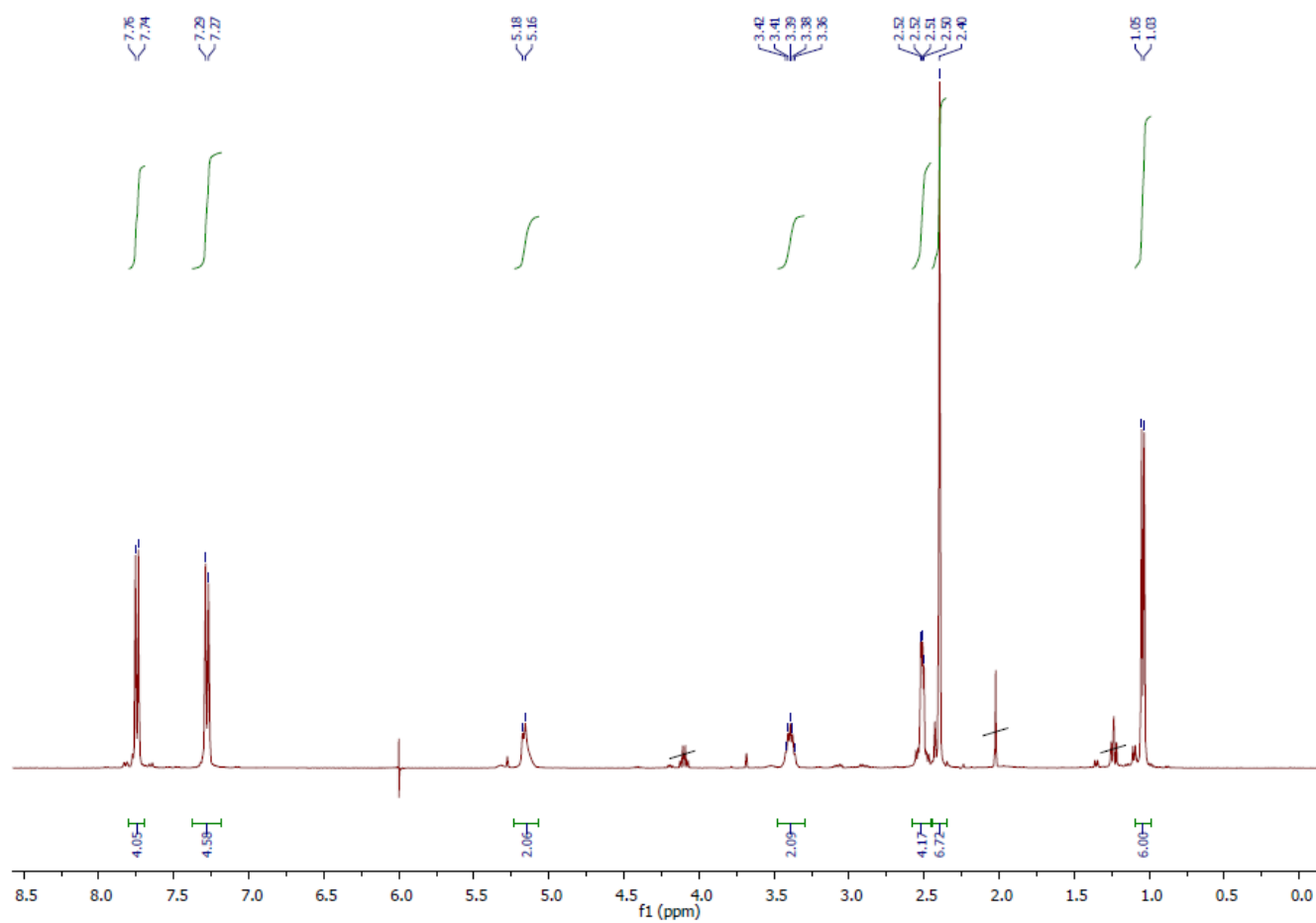
^1\text{H} NMR spectrum of compound (2R,2'R)-5 ( \text{CDCl}_3 , 400 MHz)
