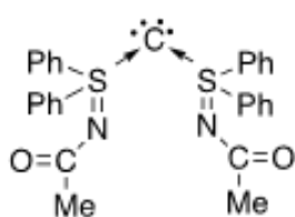
Carbene
