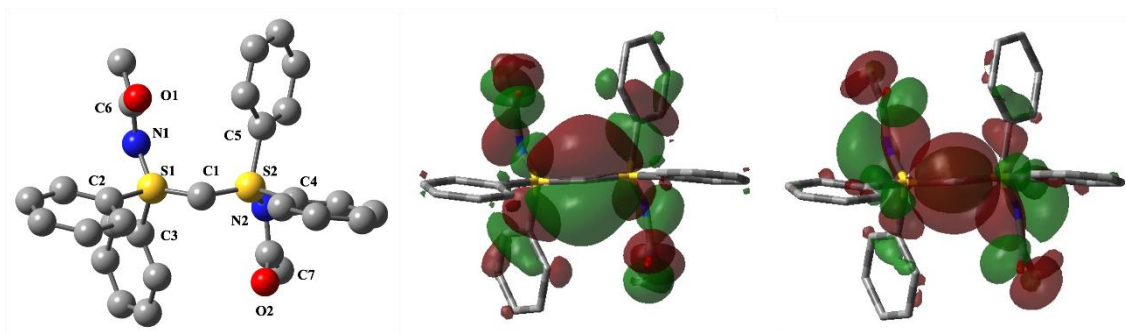
Figure 3. The optimized structure of 3 (left, hydrogen atoms are omitted for clarity) and its HOMO (center) and HOMO–1 (right).
