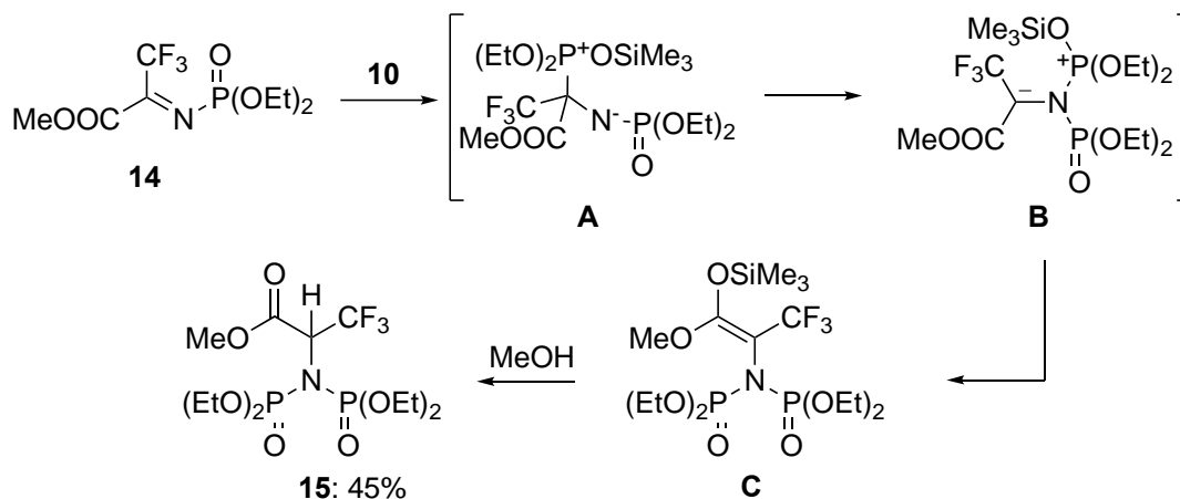
Scheme 11. Reaction of iminopyruvate 14 with silylphosphite 10 .
