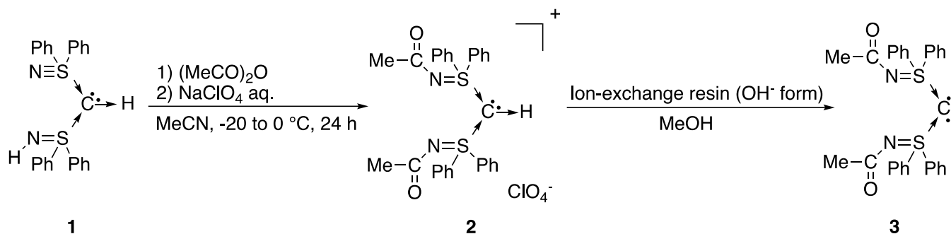
Scheme 1. Synthesis of 3 .
